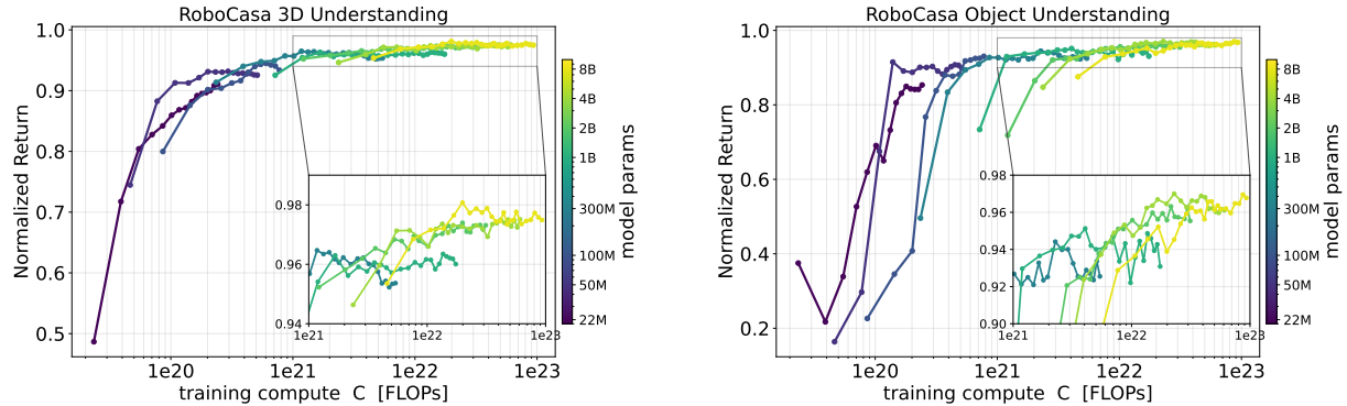
(a) The normalized return for the pose reach task in RoboCasa environment evaluated in unseen kitchens.
