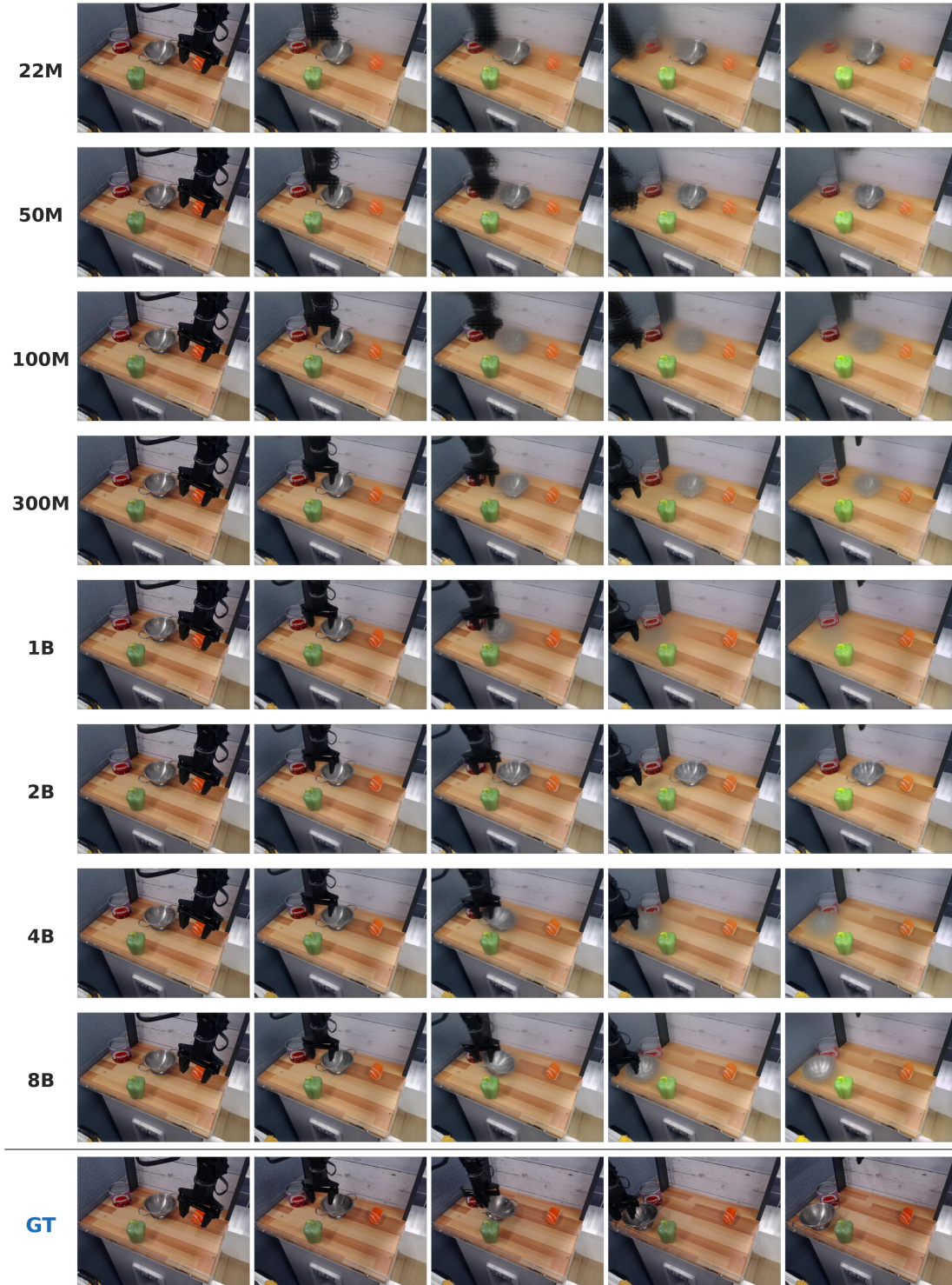
Figure 13 Open X-Embodiment Bridge (single view), 480×640. Physical contact between the gripper and the object develops only for the larger models.
