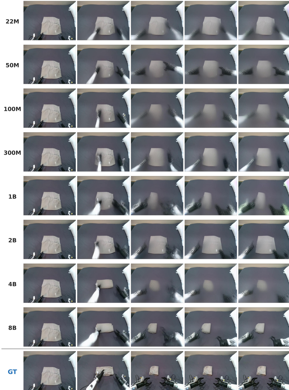
Figure 12 AgiBot (single view), 480 \times 640 . Model-size comparison of world-model imaginations against ground truth; folding structure emerges only at larger scales.
