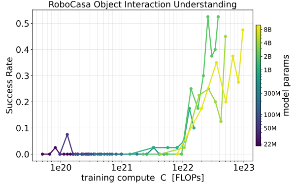
Figure 9 Downstream success rate on the RoboCasa push task versus training compute, for the long-horizon ( K = 10 ) models.
