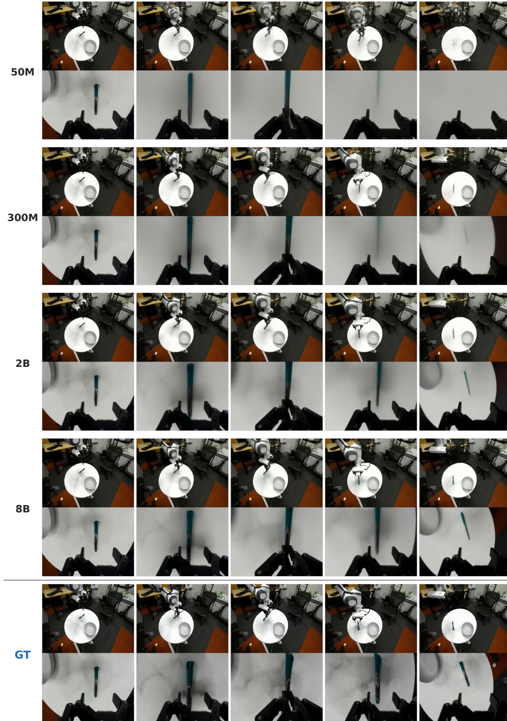
Figure 19 Franka / DROID (two views), 240 \times 320 , joint-space actions. Two-view manipulation rollout across model sizes.
