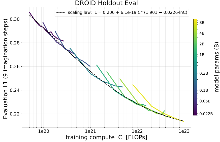
Figure 32 Long-horizon training scaling law on DROID. Long-horizon prediction training alone: per-size checkpoint curves colored by parameter count, with the fitted second-order power law (dashed) on the compute-optimal frontier of the DROID holdout evaluation.
