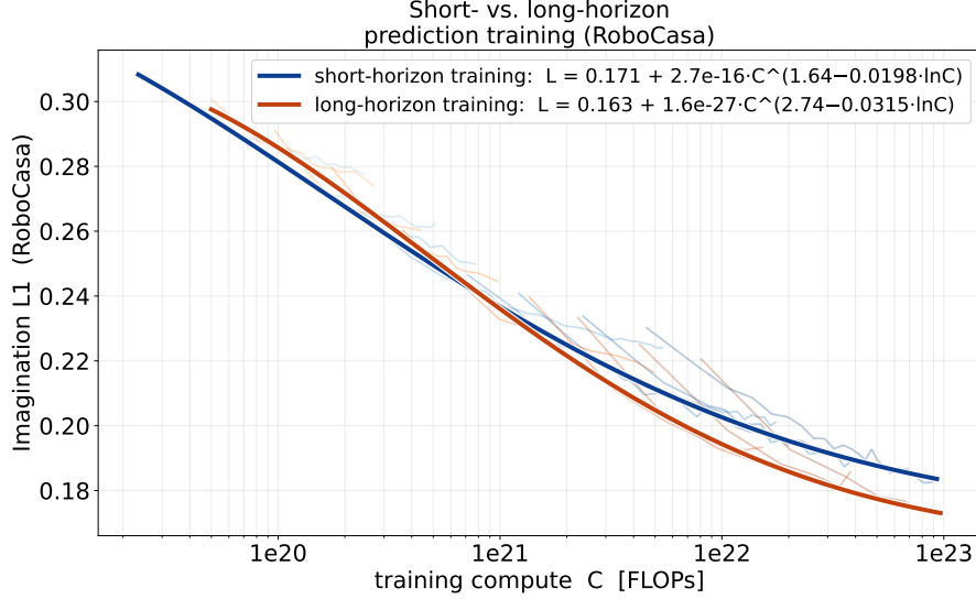
Figure 31 Short- vs. long-horizon prediction training on RoboCasa. As Figure 30, for the RoboCasa target evaluation. The same crossover and lower floor for long-horizon training hold on the simulated suite.
