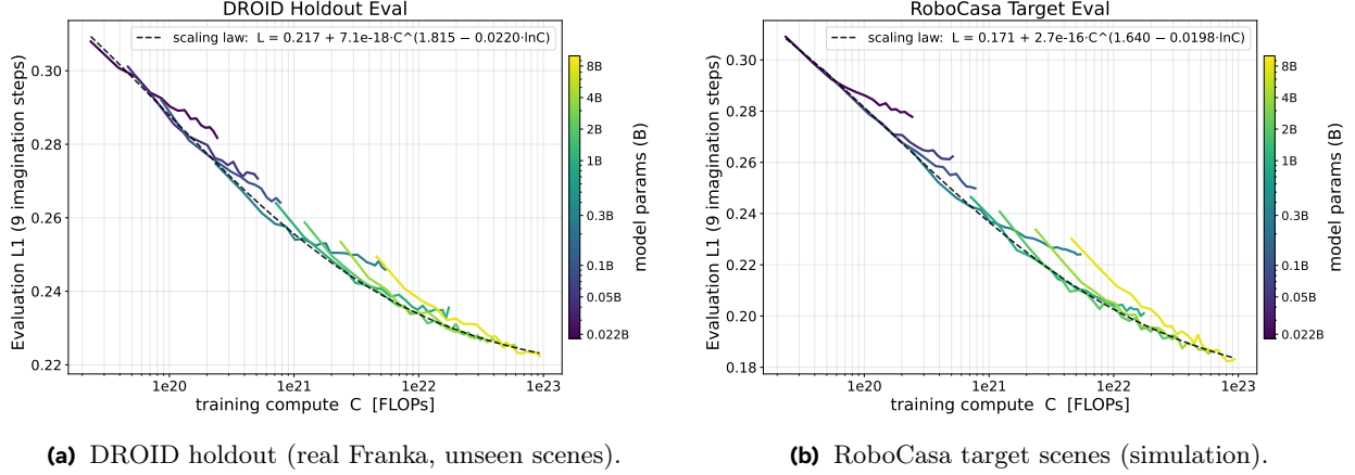
Figure 5 World-model scaling laws. Out-of-distribution forward-prediction L_1 error versus training compute for RoboJEPA models from 22M to 8B parameters (color), evaluated on a real-robot DROID holdout and simulated RoboCasa scenes. The compute-optimal frontier (lower envelope) follows the second-order power law L(C) = E + A C^{\alpha - \gamma \ln C} (dashed).
