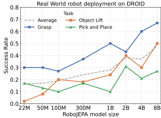
Figure 10 Real-world deployment on DROID. Success rates across model sizes for three manipulation tasks; the dashed line shows their average.
