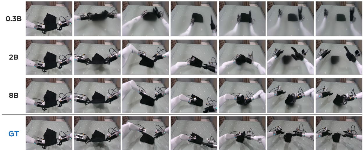
Figure 2 World-model imagination improves with scale. Decoded imagination rollouts on an AgiBot episode for RoboJEPA at 0.3B, 2B, and 8B parameters, compared against the ground-truth (GT) video (bottom row). Each row shows the same rollout sampled at equal-time steps; larger models track the true dynamics and preserve object and contact detail markedly better. All world models share the same encoder (V-JEPA 2.1-G) and decoder.
