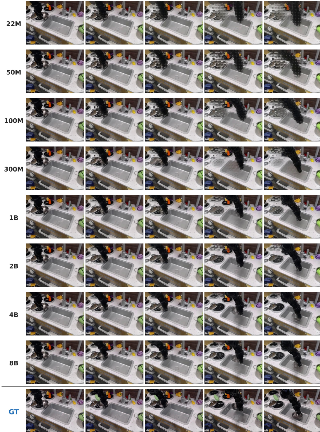
Figure 16 Open X-Embodiment Bridge (single view), 240×320. Contact with the manipulated object develops only in the larger models.
