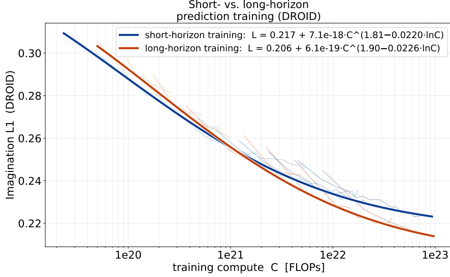
Figure 30 Short- vs. long-horizon prediction training on DROID. Out-of-distribution imagination L1 on the DROID holdout versus training compute. Faded curves are per-size checkpoints (blue: short-horizon training, orange: long-horizon training; shade encodes model size); the bold curves are the two second-order power laws fit on each recipe’s frontier. The long-horizon training law overtakes the short-horizon training one at high compute and reaches a lower irreducible floor.
