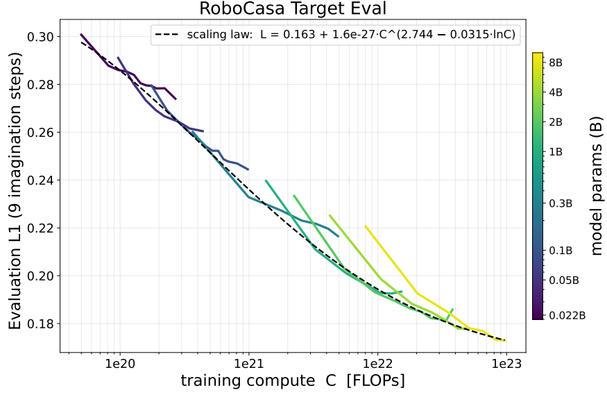
Figure 33 Long-horizon training scaling law on RoboCasa. As Figure 32, for the RoboCasa target evaluation.
