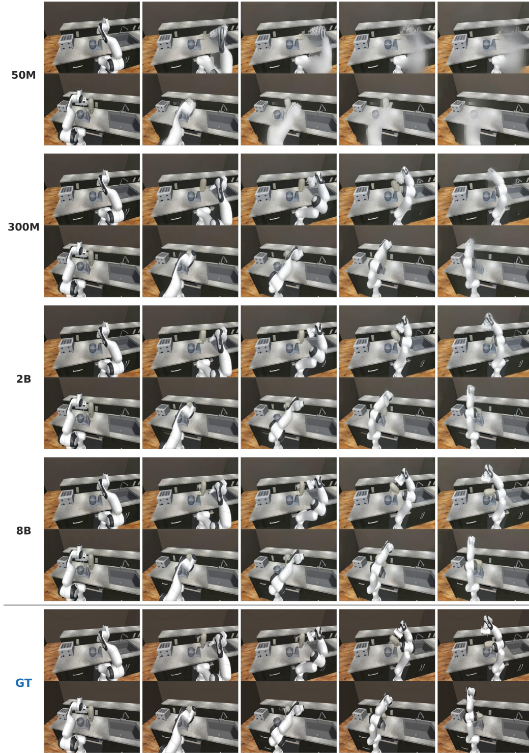
Figure 15 RoboCasa (two views), 480 \times 640 . Simulated kitchen manipulation rollout across model sizes.
