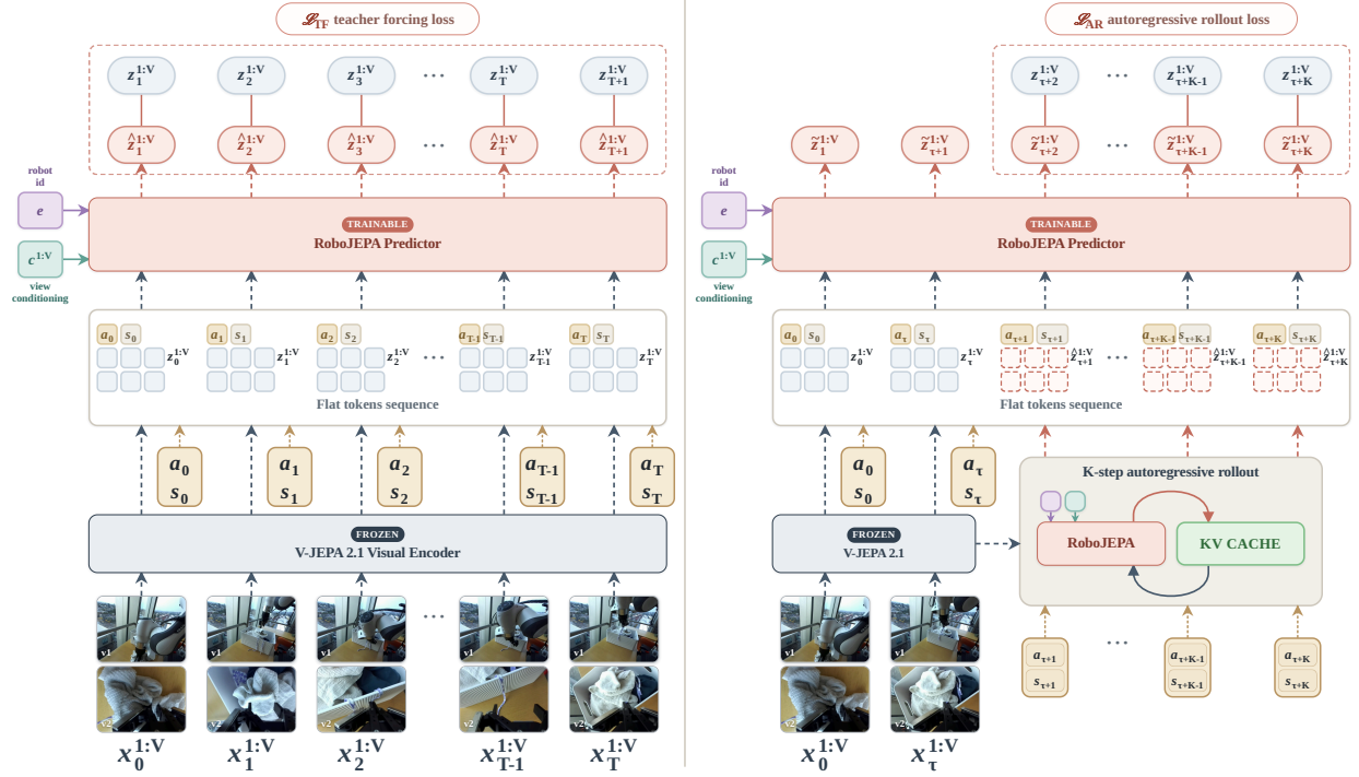
Figure 3 RoboJEPA training. The frozen V-JEPA 2.1 encoder f (Mur-Labadia et al., 2026) maps the input multiview frames x_t^{(1:V)} to a grid of features. The predictor g_\theta consumes per-step sequences of multiview visual ( z_t^{(1:V)} ), action ( a_t ) and proprioceptive state ( s_t ) tokens, conditioned on view and embodiment identifiers, and predicts the next-step features \hat{z}_{t+1} . Training minimises two losses: (left) the teacher-forcing loss , the per-token \ell_1 distance between predicted features and the next-step features from the encoder (Equation (5)); and (right) the rollout loss , which attempts to predict the same target sequence as the teacher-forcing loss, but given fewer input frames. The model is given the full training sequence of actions but only a prefix of the encoded features, and predicts the remaining features autoregressively, with a KV-cache. This way the model learns to make accurate long term predictions.
