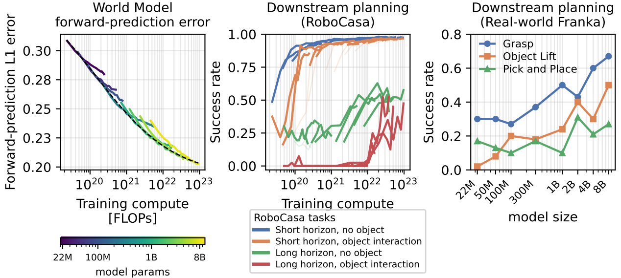
Figure 1 RoboJEPA scales predictably from offline prediction to real-robot control. Left: the world model’s forward-prediction ( \ell_1 ) error, averaged over the DROID and RoboCasa held-out sets, follows a scaling law in training compute. Middle: downstream planning success in RoboCasa improves predictably with compute across tasks of increasing difficulty. Right: on the real Franka robot, the success rate improves with model size across Grasp, Object Lift, and Pick and Place. Actions are sampled from a uniform distribution and prioritized using the World Model during planning.
