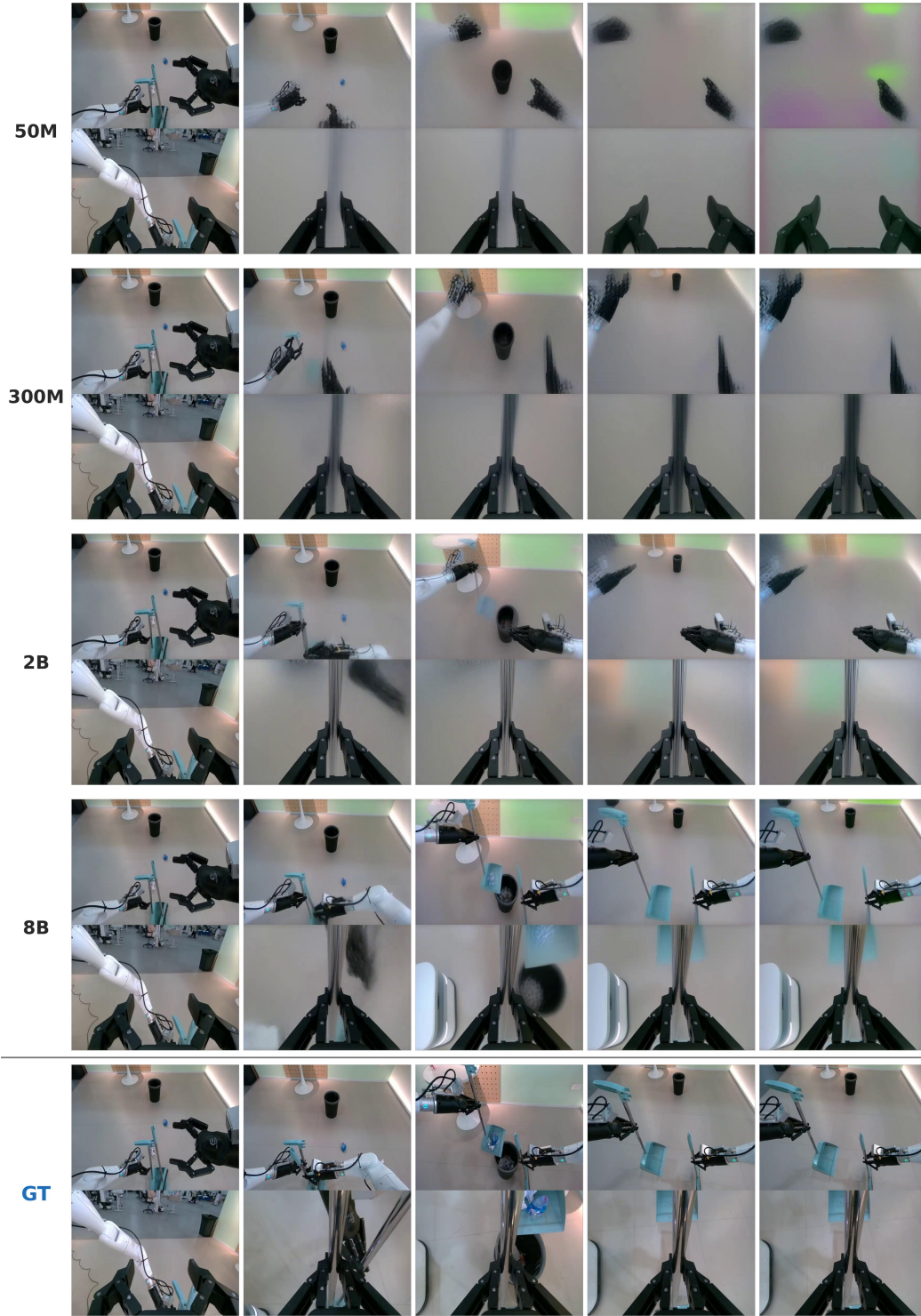
Figure 14 AgiBot (two views), 480 \times 640 . Bimanual manipulation rollout across model sizes; finer details are preserved as scale increases.
