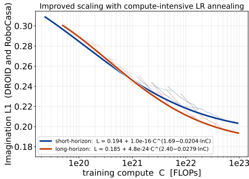
(a) Imagination error scaling for short- vs. long-horizon prediction training.
