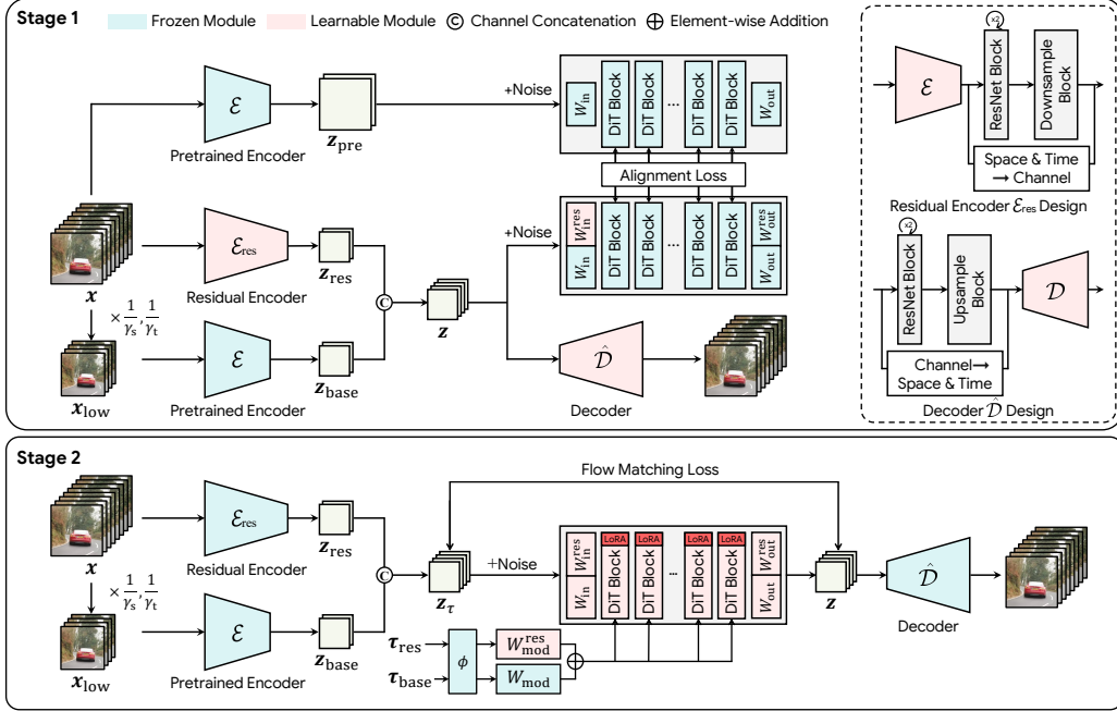
Figure 2: Overall architecture. Stage 1 trains the autoencoder. The frozen encoder \mathcal{E} maps the downsampled input to \mathbf{z}_{\text{base}} , the residual encoder \mathcal{E}_{\text{res}} maps the full-resolution input to \mathbf{z}_{\text{res}} , and \hat{\mathcal{D}} decodes both, while \mathcal{L}_{\text{align}} matches the compressed latent to the pre-trained latent inside the frozen DiT. The dashed box on the right of Stage 1 shows a simplified view of the blocks added to \mathcal{E}_{\text{res}} and \hat{\mathcal{D}} . Stage 2 adapts the DiT to the compressed latent with LoRA, denoising \mathbf{z}_{\text{base}} at a lower noise level than \mathbf{z}_{\text{res}} at every step, so the base is denoised first.
