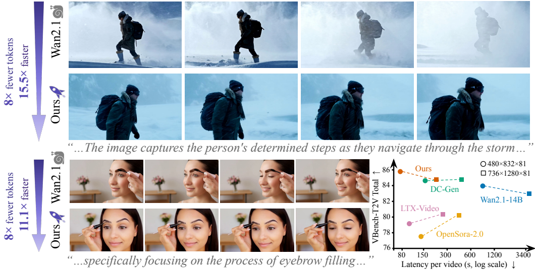
Figure 1: Teaser. We present GRACE , a novel latent compression technique that fine-tunes pre-trained video generation models, such as Wan2.1-14B (Wan et al., 2025), to generate from substantially fewer latent tokens (e.g., nearly 8× fewer). (Top) Text-to-video (T2V) samples at 736p from Wan2.1-14B before compression and from GRACE, using the same prompt. (Bottom left) The same comparison at 480p. (Bottom right) On V-Bench-T2V (Huang et al., 2023; 2024), GRACE preserves the generation quality of Wan2.1-14B before compression and achieves higher scores than existing high-compression autoencoders (HaCohen et al., 2024; Zheng et al., 2026; He et al., 2026), while generating 11.1× faster at 480p and 15.5× faster at 736p. All models in the plot are evaluated at matched resolutions with 50 sampling steps. The plot reports text-to-video, and the speedups above are measured on image-to-video.
