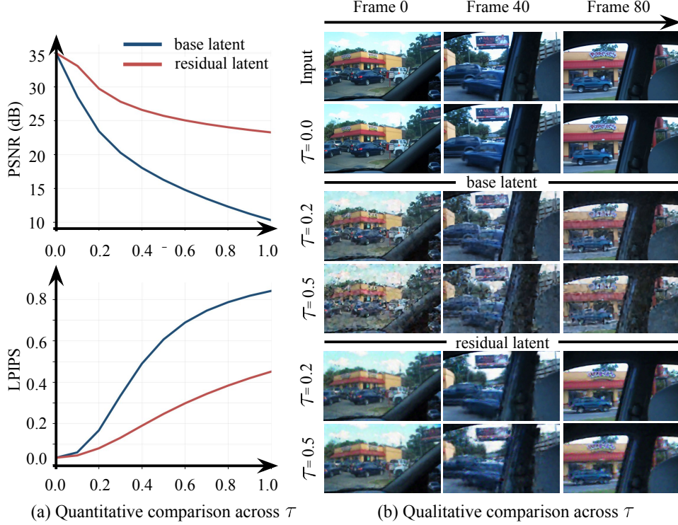
Figure F.1: Reconstruction under latent noise. We noise \mathbf{z}_{\text{base}} or \mathbf{z}_{\text{res}} at level \tau , leave the other unchanged, and reconstruct. (a) Reconstruction quality on Panda-70M (Chen et al., 2024) at 480 \times 832 \times 81 as \tau grows, measured in PSNR and LPIPS. (b) Reconstructed frames at two levels of \tau , shown below the input and the noise-free reconstruction, with the first block noising \mathbf{z}_{\text{base}} and the second noising \mathbf{z}_{\text{res}} .
