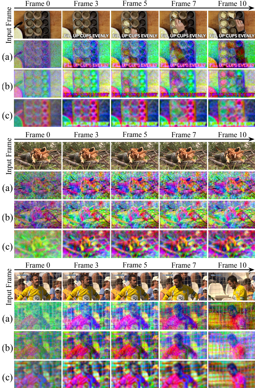
Figure I.11: Additional latent PCA visualizations. Principal components of the full C+C' latent at f16t8p2, encoded from 480 \times 832 \times 81 videos, for (a) a single encoder, (b) ours without \mathcal{L}_{\text{align}} , and (c) ours, with the input frames on top. The three leading components are computed per clip and mapped to RGB, so colors are not comparable across panels.
