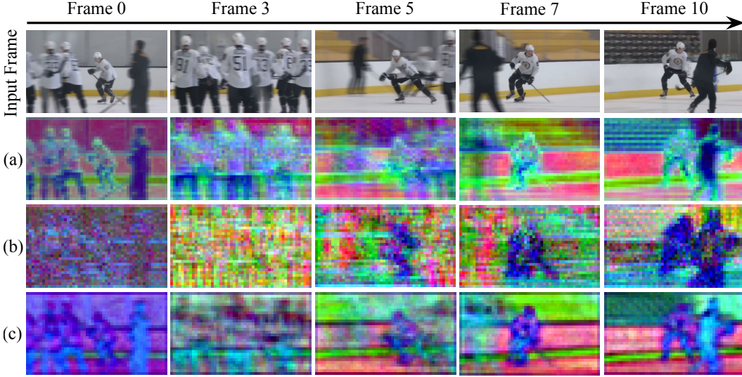
Figure F.2: PCA visualization of the base and residual latents. Principal Component Analysis (PCA) of each part at f16t8p2, encoded from a 480 \times 832 \times 81 video, for (a) \mathbf{z}_{\text{base}} , (b) \mathbf{z}_{\text{res}} without \mathcal{L}_{\text{align}} , and (c) \mathbf{z}_{\text{res}} with \mathcal{L}_{\text{align}} . Since \mathcal{E} is frozen, \mathbf{z}_{\text{base}} is the same in both settings.
