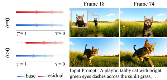
Figure 4: Denoising order. Each row shows the sampling steps of \mathbf{z}_{\text{base}} and \mathbf{z}_{\text{res}} ( Left ) and the generated frames ( Right ), with \tau = 1 pure noise and \tau = 0 clean. ( Top ) Both parts are denoised at the same noise level. ( Bottom ) \mathbf{z}_{\text{base}} stays \delta ahead of \mathbf{z}_{\text{res}} in schedule time u (Eq. 11) at every step.
