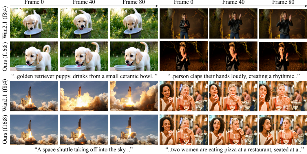
Figure 6: Qualitative comparison at 736 \times 1280 \times 81 . VBench (Huang et al., 2023; 2024) samples from Wan2.1-14B (Wan et al., 2025) before compression and GRACE (Ours), generated from the same prompt, for text-to-video ( top ) and image-to-video ( bottom ). Best viewed when zoomed in.
