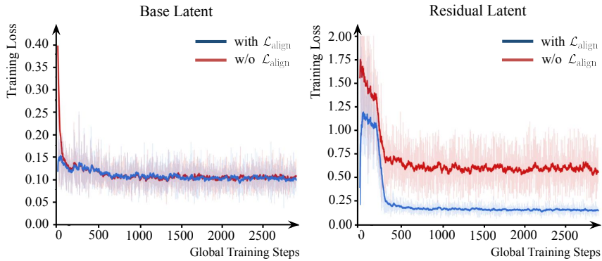
Figure F.3: Convergence of the base and the residual. Flow matching loss on the base channels (left) and the residual channels (right) during DiT adaptation, for the dual latent with and without \mathcal{L}_{\text{align}} . Each part is standardized with its own statistics. Faint curves show the raw loss and solid curves its EMA.
