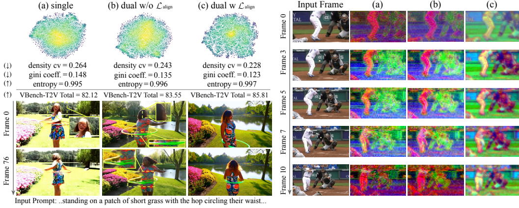
Figure 3: Effect of the dual latent and \mathcal{L}_{\text{align}} . (a) single latent, (b) dual-latent representation without \mathcal{L}_{\text{align}} , and (c) ours, all generated at 480 \times 832 \times 81 . (Left) latent distribution, projected with t-SNE and colored by kernel density, with its uniformity metrics (Yao et al., 2025) and the total VBench (Huang et al., 2023; 2024) score below, followed by T2V samples generated after Stage 2. (Right) spatio-temporal structure of the latent, shown as its principal components mapped to RGB under the input frames. More samples are in Figs. I.11 and I.12.
