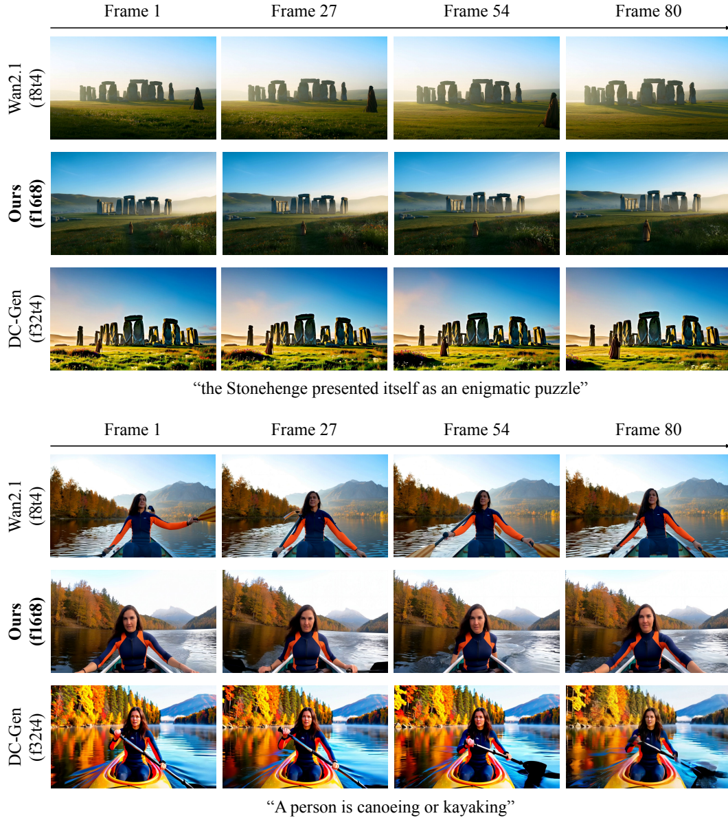
Figure I.5: Additional high-resolution text-to-video results. Samples at 736 \times 1280 \times 81 , generated by the pretrained Wan2.1-14B (Wan et al., 2025) at f8t4p2, ours at f16t8p2, and DC-Gen (He et al., 2026) at f32t4p1, from the same prompt.
