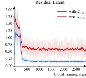
Figure 7: Convergence during DiT adaptation. With and without \mathcal{L}_{\text{align}} ; solid lines show EMA.
