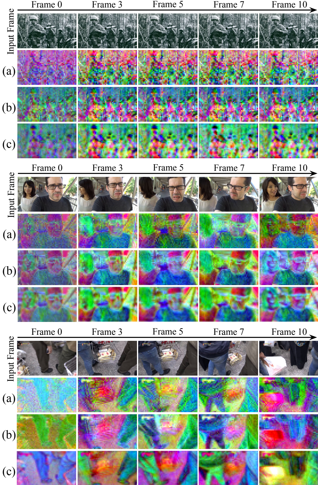
Figure I.12: Additional latent PCA visualizations (continued). Principal components of the full C+C' latent at f16t8p2, encoded from 480 \times 832 \times 81 videos, for (a) a single encoder, (b) ours without \mathcal{L}_{\text{align}} , and (c) ours, with the input frames on top. The three leading components are computed per clip and mapped to RGB, so colors are not comparable across panels.
