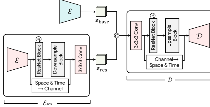
Figure A.1: Detailed autoencoder architecture. \mathcal{E}_{\text{res}} adds a downsampling stage between its middle blocks and head, consisting of residual blocks and a strided causal convolution, paired with a parameter-free shortcut that folds space and time into channels.
