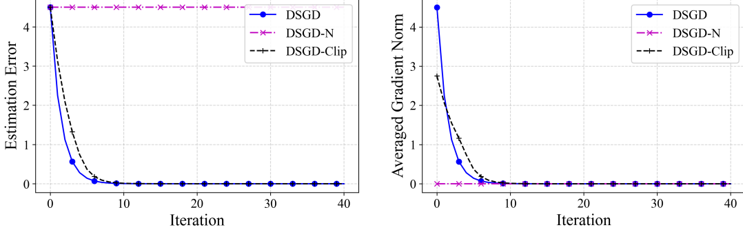
Figure 4: Convergence of vanilla, normalized and clipped DSGD on a quadratic example.
