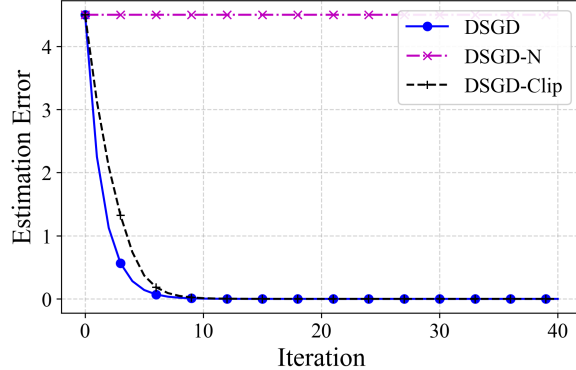
Figure 1: Convergence of vanilla, normalized and clipped DSGD on a quadratic cost. While normalization gets stuck at the initial point and fails to converge, both vanilla and clipped DSGD converge to the true minima. For more details, see Supplement C.
