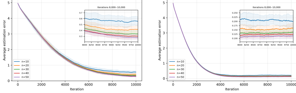
Figure 3: Convergence of DSGD-Clip under heavy-tailed noise for networks of size n \in \{10, 20, 30, 40, 50\} . Left: Student’s t noise; right: Lévy \alpha -stable noise. We can see that DSGD-Clip accelerates with network size, achieving linear speed-up.
