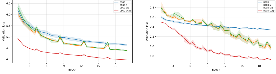
Figure 5: Validation loss versus training epoch for decentralized transformer training. Left: “Multi30k”; right: “Tiny Shakespeare” dataset.
