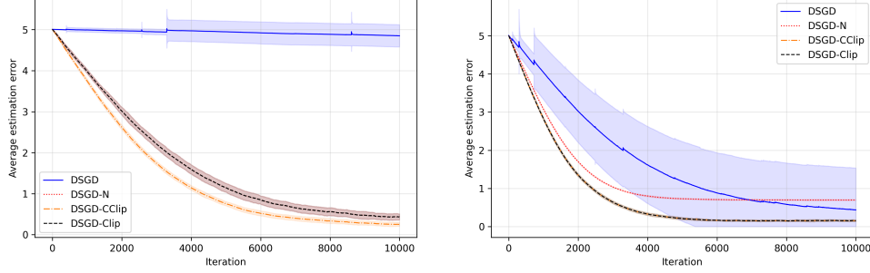
Figure 2: Convergence of decentralized methods under heavy-tailed gradient noise. Left: Student’s t noise; right: Lévy \alpha -stable noise. Solid curves show the mean estimation error, while shaded regions indicate one standard deviation.
