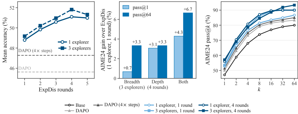
Figure 4: Under a fixed RL compute budget, how we allocate compute impacts downstream student policy performance. We vary the number of explorers and rounds under a fixed compute budget, and find complementary impacts of each scaling axis. Under a fixed budget, adding rounds improves pass@1 more than adding explorers, and combining both gives the largest gains in pass@1 and pass@64. All results are reported on Qwen3-1.7B.
