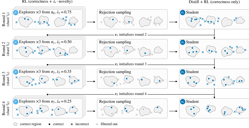
Figure 2: ExpDis scales across parallel explorers and iterations. Within a round, several explorers are trained in parallel with a novelty bonus, and their traces are pooled to distill a single student. Across rounds, that student initializes both the next round’s explorers and the next round’s student, so every round starts from a stronger model. Each round trains on its own shard of the training prompts, and the novelty weight anneals from \lambda_1=0.75 to \lambda_4=0.25 . We study how to allocate a fixed RL budget across explorers and rounds in Section 5.
