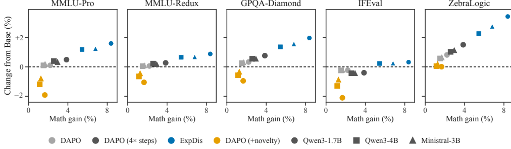
Figure 12: We report the degradation from adding a novelty bonus directly to the DAPO reward.
