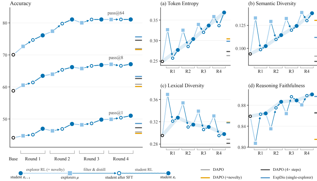
Figure 7: In successive ExpDis iterations, the student captures more of the explorer’s diversity while avoiding its degradations. We track the explorers and the student as they evolve during several ExpDis rounds and report the final baseline policies to the right of each panel. (a) Explorer RL causes a rise in token entropy often at the expense of accuracy, whereas the student’s entropy generally rises together with its accuracy across rounds. (b) The explorer policy semantic diversity stays roughly constant, and the student closes most of the gap to it by the final round. (c) We find that the student does not retain the lexical diversity of its explorers: it declines over rounds even as the student’s accuracy improves. Together with Figure 5, where large \lambda harms the student, this suggests that lexical diversity is not a useful target for exploration. (d) Reasoning faithfulness, as defined by Rahman et al. [31], measures whether a response’s reasoning supports its final answer. We find that novelty bonus typically causes faithfulness to decline, though the impact is mild by the final round. Results are averaged over three models (breakdown in Figure 14).
