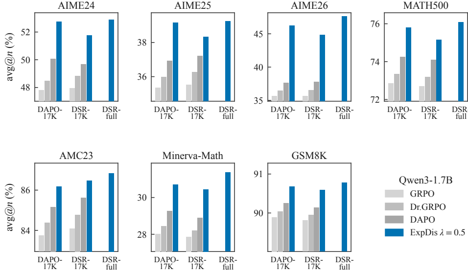
Figure 16: We ablate the choice of training dataset, sampling a fixed prompt budget from each and training with a single-explorer ExpDis approach. We find a consistent gain over several RLVR baselines.
