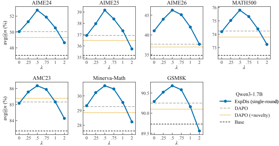
Figure 11: On Qwen3-1.7B, we find that a novelty bonus weight of \lambda=0.5 on the explorer policy roughly maximizes downstream student policy performance, though several values of \lambda outperform the DAPO baseline.
