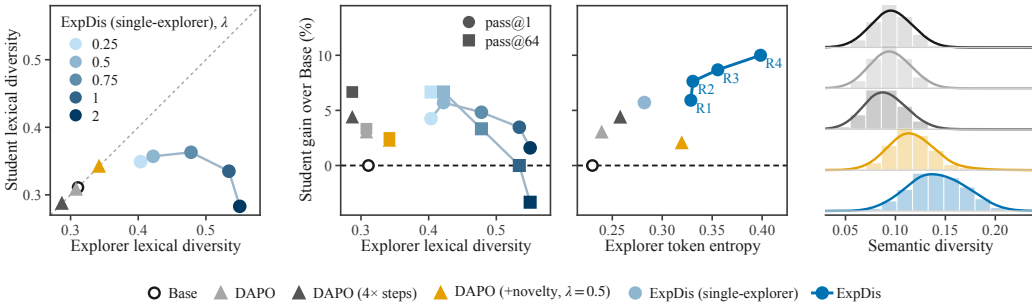
Figure 5: Explorer policy can be driven to more diversity without harming the student. Left: We study how explorer policy diversity impacts the downstream student in ExpDis. In general, we find that we can push the diversity of the explorer policy without corrupting the downstream student policy. Since we filter for correctness and quality before distilling, a moderate increase in explorer diversity (for example, lexical diversity) brought on by tuning the novelty bonus weight \lambda does not negatively impact the student policy. Similarly, we can increase the explorer token entropy far beyond that of DAPO (+novelty) without incurring downstream reasoning degradation. Right: We find that ExpDis generations contain more semantically diverse mathematical reasoning strategies. We define each diversity metric in Appendix D.
