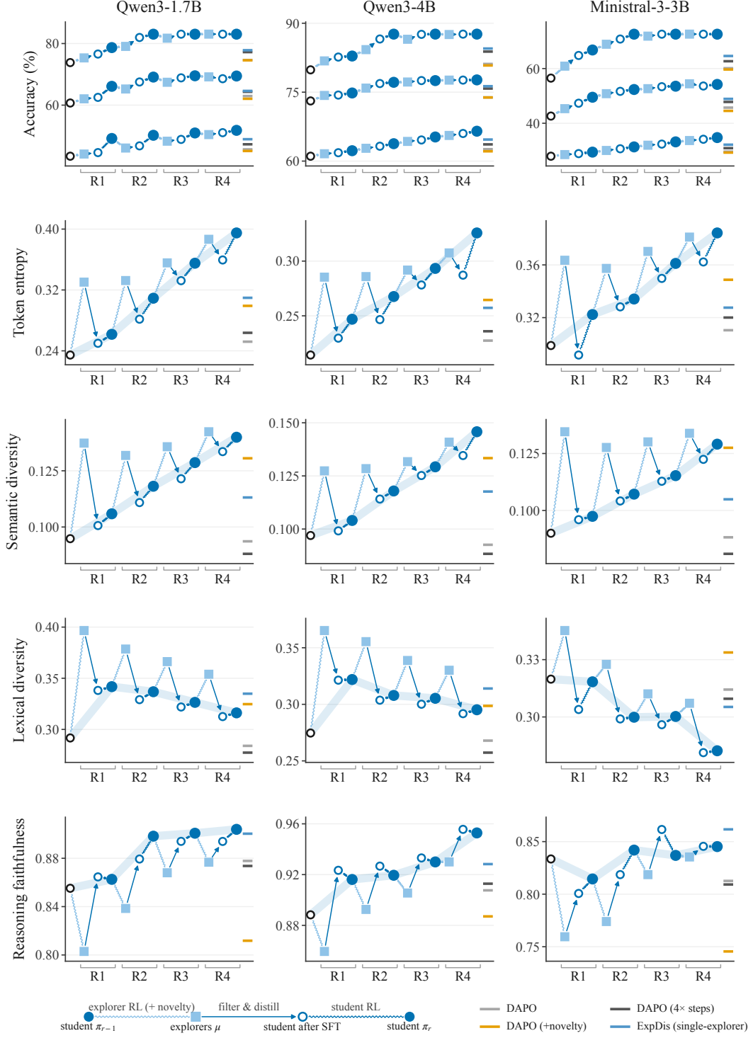
Figure 14: We study the evolution of student and teacher policies during several stages of ExpDis.
