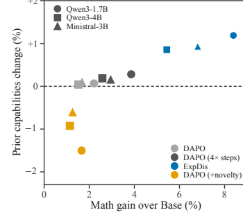
Figure 6: Adding RND novelty bonus to DAPO degrades prior capabilities.
