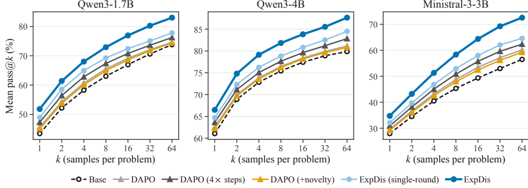
Figure 3: ExpDis outperforms all baselines under the same RL compute budget. By partitioning this budget into alternating rounds of exploration and optimization (as described in Section 3.2), we can surpass DAPO and even a single round of ExpDis. We report full benchmark results in Appendix B.
