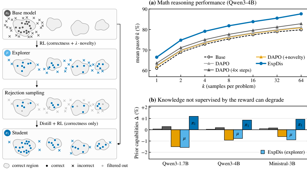
Figure 1: Decoupling exploration from optimization improves math accuracy without degrading prior capabilities. Left: Rather than coupling exploration and optimization in a single RLVR run, ExpDis assigns these roles to separate policies. We first train an explorer \mu with a novelty bonus in its reward, then distill a diverse pool of its reasoning traces to cold start a student, and finally train the student with standard RLVR using only a correctness reward. As depicted in the figure, this allows us to explore a diverse set of reasoning strategies and preserve this diversity in our student policy. (a) ExpDis outperforms DAPO in both average accuracy and pass@ k , even when DAPO is trained for 4 \times as long (Qwen3-4B, mean pass@ k over five math benchmarks). (b) Adding a novelty bonus (RND) directly to the DAPO reward degrades performance on prior capabilities relative to the base model. Because the reward supervises only a narrow slice of the model’s knowledge (here, mathematical reasoning), achieving high reward does not prevent general capability degradation. By decoupling the explorer from the student policy, we avoid this degradation.
