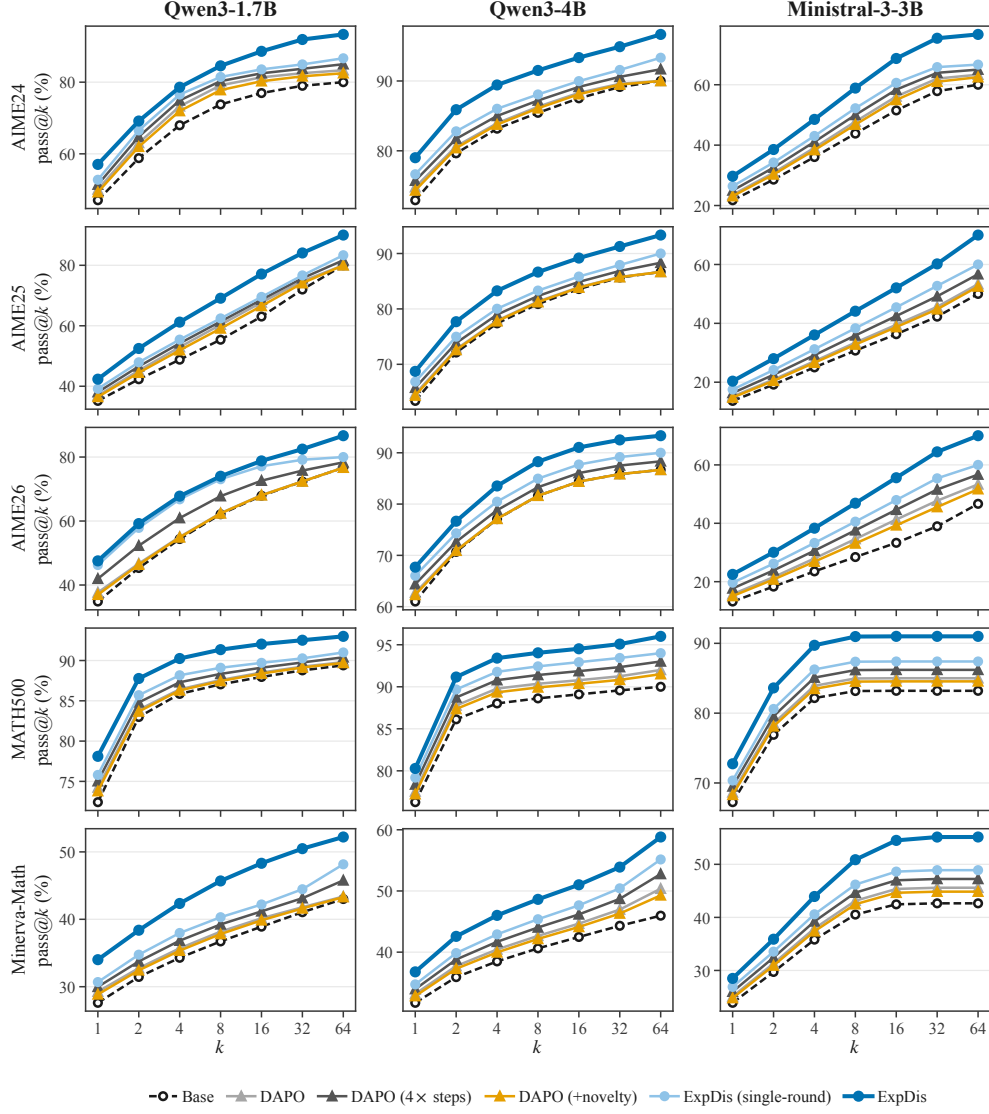
Figure 9: Full pass@k results.
