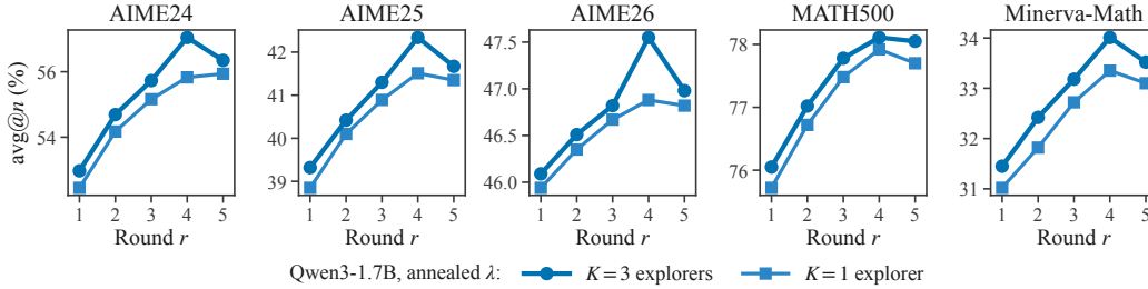
Figure 13: Impact of increasing rounds given a fixed number of explorers per round.
