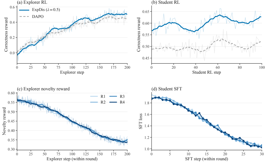
Figure 8: Training dynamics of continued training on Qwen3-1.7B with our ExpDis setup ( \lambda=0.5 ).
