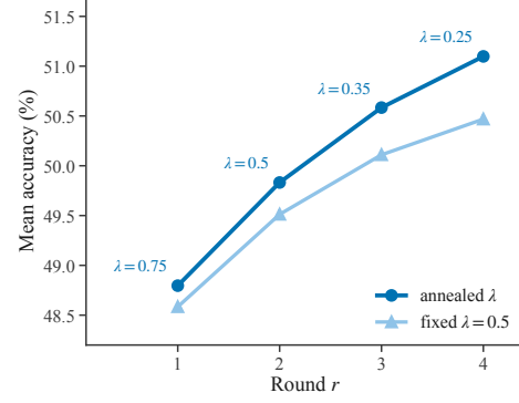
Figure 15: Fixed versus annealed \lambda across four rounds (Qwen3-1.7B, single-explorer). The annealed schedule uses \lambda=0.75, 0.5, 0.35 , and 0.25 .
