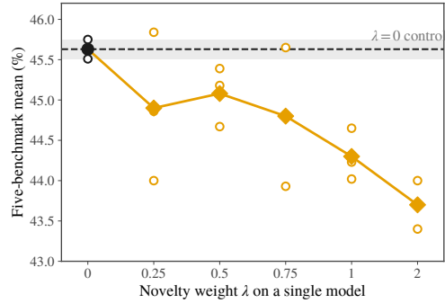
Figure 10: Adding a novelty bonus directly to the reward in DAPO degrades accuracy on math reasoning.
