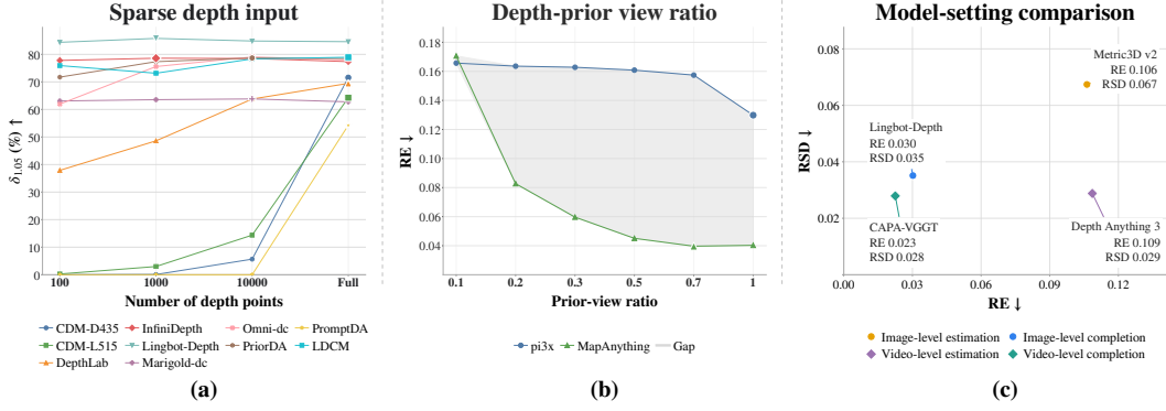
Figure 5: (a) Image-level completion accuracy ( \delta_{1,05} ) with 100, 1,000, or 10,000 randomly sampled depth points, or full sensor depth (Full). (b) Video-level completion RE as the fraction of views with depth priors increases from 0.1 to 1.0; shading indicates the gap between models. Enlarged markers in (a,b) highlight each model’s best setting. (c) RE versus RSD of predicted distances for representative image- and video-level estimation and completion models. Points closer to the lower-left corner indicate greater accuracy and cross-frame consistency.
