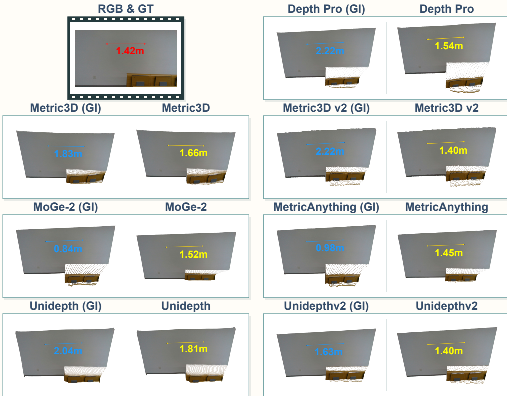
Figure 8: Qualitative comparison for image-level geometry estimation models between back-projecting with ground-truth intrinsics and models' predicted intrinsics. Ground-truth annotations are shown in red , (ground-truth intrinsics + depth maps) are shown in blue , (predicted intrinsics + depth maps) are shown in yellow .
