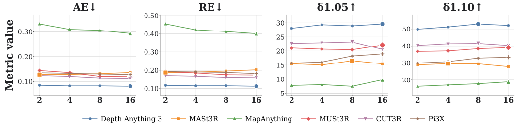
Figure 7: Effect of sampling stride on video-level geometry estimation models (normal subset only). Each curve corresponds to one model, and the highlighted marker on each curve indicates that model’s best-performing stride.
