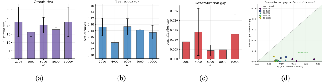
Figure 1: Relationship between training-set size N Vs (a) circuit size T^* , (b) test accuracy, (c) generalization gap, and (d) Generalization gap versus the full Caro et al. Theorem 3 bound B_K . The shaded region indicates where the bound holds.
