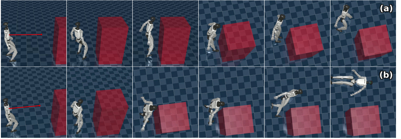
Fig. 6. Push-Avoid simulation. The red box marks the protected region and the arrow denotes the push. (a) The robot remains upright while staying outside the region. (b) When the push is too hard, the robot sacrifices balance and falls away while protecting its head and hands.
