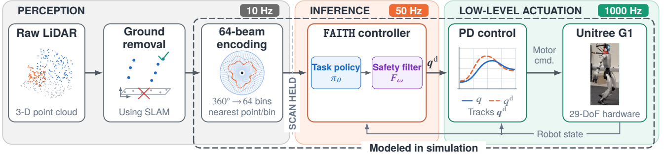
Fig. 7. Hardware control pipeline. SLAM-based ground removal and angular binning produce a 64-beam LiDAR observation. FAITH generates joint targets tracked by PD control. The dashed box marks simulated components, including G1 dynamics and analytically generated beam inputs.
