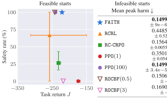
Fig. 3. Double integrator results: safety rate and task return of feasible starts, and mean peak harm of infeasible starts. Left: For feasible starts, FAITH achieves a 100% safety rate, and the highest return among all safe methods (error bars show min-max ranges). Right: For infeasible starts, FAITH achieves the lowest peak harm ( \pm shows the standard deviation).
