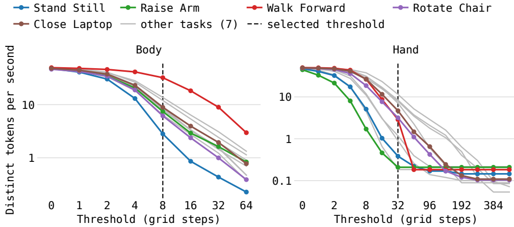
Figure 12: Token counts vs. threshold. Curves show how grouping distance changes the number of distinct body and hand representatives. Each recording’s count is divided by its duration before averaging within each task; the vertical axis is logarithmic. Colored curves identify the five tasks in Figure 5; gray curves show seven additional tasks. Dashed lines mark the reported body and hand thresholds of 8 and 32.
