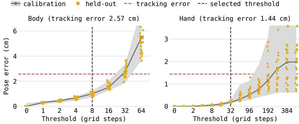
Figure 11: Threshold calibration. Each episode is summarized by the 95th percentile of framewise error, averaged over 14 body links or six fingertip proxies. The gray line shows the median of the calibration episodes’ errors; shading spans their minimum and maximum. Gold dots show held-out episodes; triangles mark values above the displayed range. Red horizontal lines mark the tracking-error references (2.57 cm body, 1.44 cm hand). Vertical dashed lines mark the reported thresholds of 8 and 32, chosen finer than the permitted 16 and 96 to reduce wrist and individual-finger deviations.
