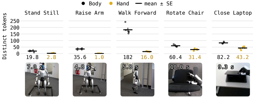
Figure 5: Complex movements have compact descriptions in motion tokens. Each dot is the number of distinct body (black) or hand (gold) motion tokens over one complete recording, after grouping similar predictions as described in Appendix A.10. Horizontal marks show the mean and vertical whiskers one standard error across five recordings per task. Numbers below give mean counts and durations. Chair rotation and laptop closing require tens of distinct body and hand tokens over roughly ten seconds of execution.
