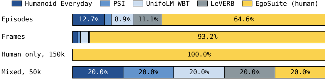
Figure 9: Dataset size and VioLA training schedule. The first two bars show each source’s share of episodes and frames in the converted pool. The last two show sampling probabilities during 150k steps of human-only training and 50k steps of uniform sampling over all five corpora. Human recordings supply 93.2% of available frames; the training schedule determines how often they are sampled.
