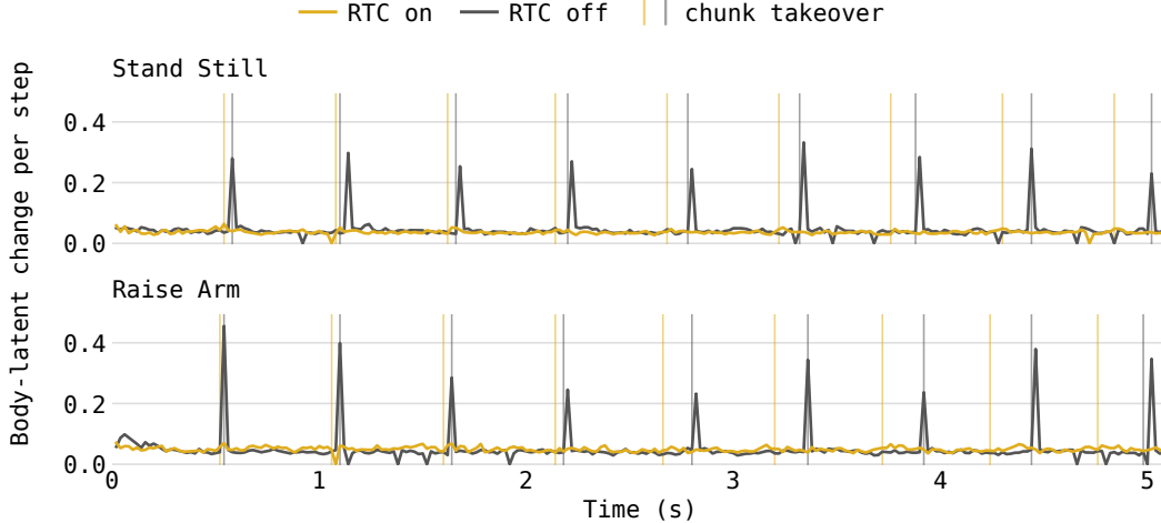
Figure 8: RTC reduces jumps when a new motion chunk takes over. Each row compares VioLA recordings with RTC on (gold) and off (gray). Curves show the L2 change in the 64-coordinate body latent between consecutive 20 ms control steps. Vertical lines mark chunk switches in the corresponding condition’s color. RTC-off traces show sharp spikes near these switches, whereas RTC-on traces remain close to their between-switch variation. Each recording is aligned to the start of policy execution and shown for 5.1 s; the initial idle-to-policy transition is excluded.
