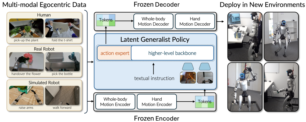
Figure 1: VioLA. Human and robot motion encoders produce targets in shared body and hand latent spaces. The generalist policy predicts motion latents from vision, language, and proprioception; frozen robot controllers execute its predictions. Annotated human motion therefore supervises the policy in the same action representation as robot motion.
