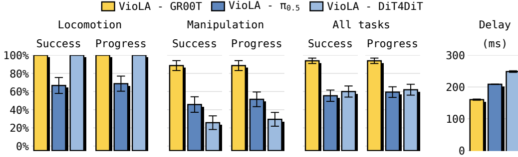
Figure 7: VioLA with two VLA backbones and one WAM backbone. The variants use the same training data and budget and are evaluated without task-specific fine-tuning. Bars report success and progress over 30 locomotion trials, 35 manipulation trials, or all 65. VioLA reaches 100% locomotion success with either GR00T or DiT4DiT, while GR00T performs best on manipulation. The final panel shows measured prediction delay. Error bars show one standard error over trials for performance and over recorded episodes for delay.
