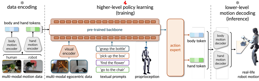
Figure 2: VioLA overview. Left: frozen motion encoders construct body and hand action targets from human or robot demonstrations. Center: the generalist policy predicts motion latents from an egocentric image, an instruction, and proprioception. It is the only component updated during training. Right: a frozen body controller and hand decoder convert the predicted latents into robot joint commands. Human and robot encoders produce targets for these same decoders.
