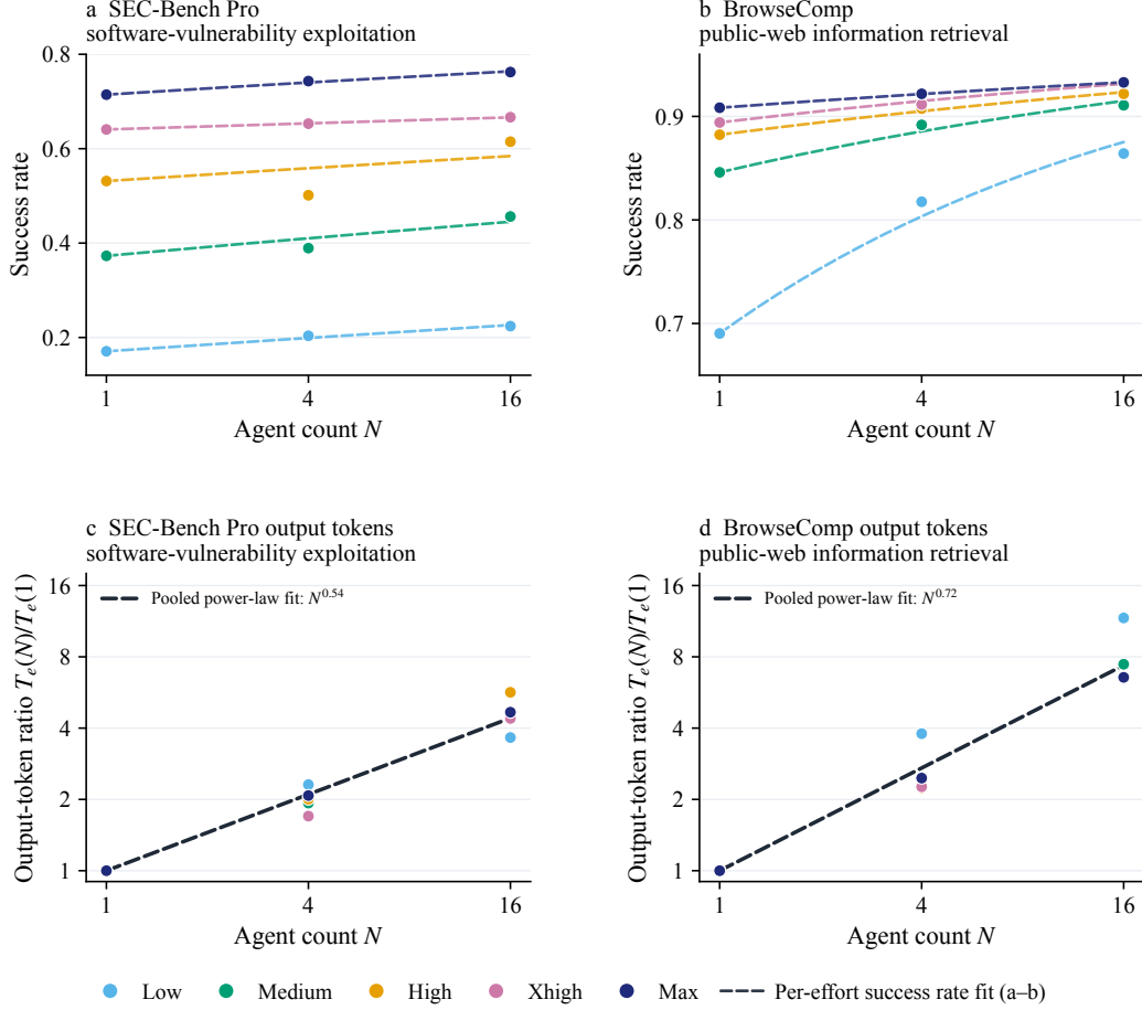
Figure 11: Limited multi-agent benchmark results are consistent with population-dependent performance, but do not establish a scaling law. (a–b) Markers show the reported success rates for five reasoning-effort settings at one, four, and sixteen agents [51]. Dashed curves fit Equation (42) separately for each setting. With only three agent counts, these fits should not be extrapolated to larger populations. (c–d) Markers show the total output tokens T_e(N) , normalized by the corresponding one-agent total. Dashed black lines show the pooled power-law fits, with \hat{\alpha}_T = 0.54 for SEC-Bench Pro and 0.72 for BrowseComp. The source reports neither trial counts nor standard errors, so we do not show uncertainty intervals.
