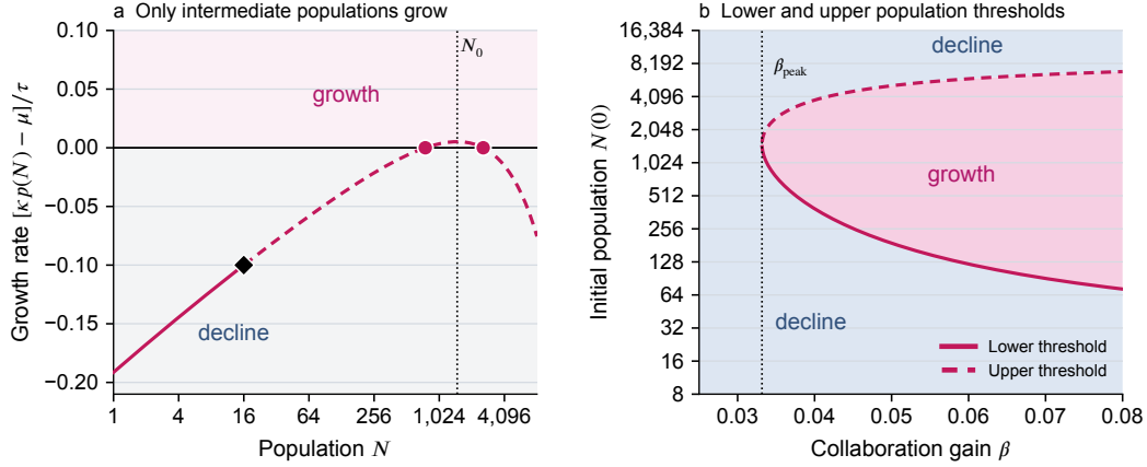
Figure 10: Unavoidable congestion creates lower and upper bounds for population growth. The pink curves show the congestion model with illustrative scale N_0 = 1500 , with other parameters chosen as in Figure 7 ( p_{\text{ref}} = 0.10 , p_{\text{crit}} = \mu/\kappa = 0.20 , and \beta = 0.035 in panel a). (a) Per-unit growth rate is plotted against population. It is positive only between N_{\text{crit}}^{(0)} \simeq 761 and N_{\text{crit}}^{(-1)} \simeq 2,610 . The diamond marks N_{\text{ref}} = 16 , the vertical dotted line marks where effective work reaches a maximum at N_0 , and the dashed portion is extrapolated beyond N_{\text{ref}} . (b) Initial population is plotted against collaboration gain, \beta . The solid and dashed pink curves mark the lower and upper population thresholds; they meet at N_0 when \beta = \beta_{\text{peak}} \simeq 0.0332 . Populations between the curves grow, whereas populations outside them decline.
