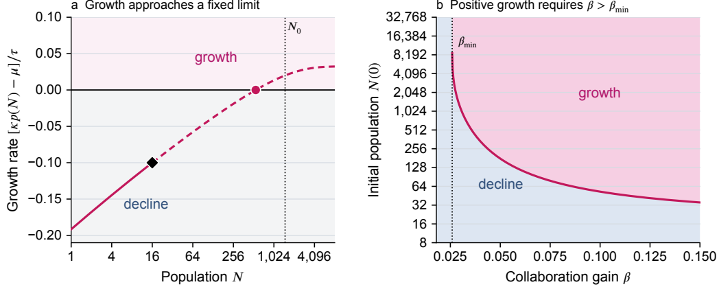
Figure 9: Effective-work saturation creates a minimum collaboration gain for population growth. The pink curves show the saturating-work model with illustrative scale N_0 = 1500 , with other parameters chosen as in Figure 7 ( p_{\text{ref}} = 0.10 , p_{\text{crit}} = \mu/\kappa = 0.20 , and \beta = 0.035 in panel a). (a) Per-unit growth rate is plotted against population. It crosses zero at N_{\text{crit}} \simeq 550 and approaches a positive constant as effective work saturates. The diamond marks N_{\text{ref}} = 16 , the vertical dotted line marks N_0 , and the dashed portion is extrapolated beyond N_{\text{ref}} . (b) Initial population is plotted against collaboration gain, \beta . A finite critical-population boundary exists only for \beta > \beta_{\min} \simeq 0.0259 : populations above the curve grow and populations below it decline. For \beta \leq \beta_{\min} , every population declines.
