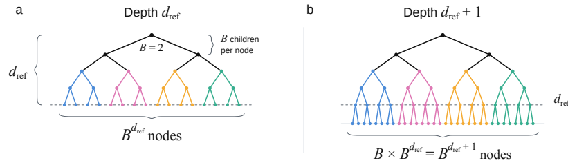
Figure 4: Search-tree exploration grows exponentially with depth. Schematic of a search tree with branching factor B = 2 . (a) At some reference depth d_{\text{ref}} , there are B^{d_{\text{ref}}} possible paths. (b) Increasing the search depth by one level generates B children from each previous endpoint node, so the number of possible paths increases to B^{d_{\text{ref}} + 1} . While this diagram illustrates exactly B children per node, in our model, B is an effective branching factor: individual nodes may have different numbers of children, and B captures the average multiplicative increase in the number of possible paths upon increasing the depth by one.
