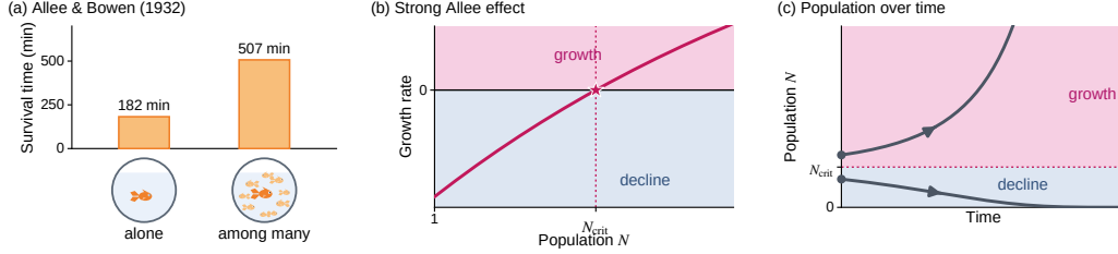
Figure 1: Allee effect. (a) In 1932, the ecologists Allee and Bowen discovered that the survival time of a collective of goldfish is longer than that of an isolated single goldfish [40]. Such observations led to the conception of a weak Allee effect, where a larger population and cooperation among its members positively affect their fitness, as well as a strong Allee effect (b), where cooperation creates an emergent population threshold below which the population declines, but above which it grows. (c) Population dynamics over time with examples of initial populations below and above the critical threshold.
