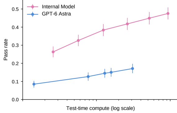
Figure 6: Motivation from test-time compute scaling. This figure is redrawn from the data reported in OpenAI [3] on the Navier–Stokes Millennium Prize Problem. Over the measured range, the pass rate on a set of open math problems increases with log test-time compute. This motivates a locally logarithmic increase in success probability with respect to effective work done. However, on its own, this does not establish that increasing the number of units is equivalent to increasing test-time compute, since it is not explicitly stated whether the reported compute was measured in a single-agent or multi-agent setting.
