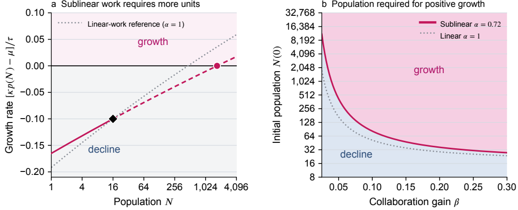
Figure 8: Sublinear effective work shifts the N_{\text{crit}} boundary to larger populations. The pink curves show sublinear effective work ( \alpha = 0.72 ) while dotted black curves show the linear case ( \alpha = 1 ) for comparison, with other parameters chosen as in Figure 7 ( p_{\text{ref}} = 0.10 , p_{\text{crit}} = \mu/\kappa = 0.20 , and \beta = 0.035 ). (a) Per-unit growth rate is plotted against population. Per-unit growth crosses zero at N_{\text{crit}} \simeq 1,714 for sublinear scaling and N_{\text{crit}} \simeq 463 for linear scaling. The diamond marks N_{\text{ref}} = 16 . (b) Initial population is plotted against collaboration gain, \beta . Populations above each curve grow and populations below it decline.
