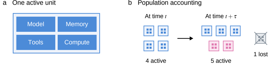
Figure 3: Active units and population accounting. (a) One “unit” is defined as the set of model, memory, tools, and compute required to set up additional units. (b) A schematic of the population dynamics model: over each time period, \tau , some number of new units are established and some existing units are lost.
