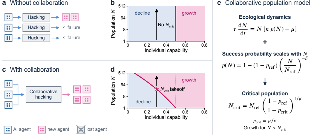
Figure 2: Collaboration creates a population threshold for takeoff. An overview of our model. Members of an AI population may make hacking attempts to gain computational resources and establish additional units, either independently or through collaboration. (a) Agents may make individual attempts at gaining access, after which only the successful agents can create new agents. (b) With no collaboration, the growth boundary depends on individual capability but not on N , so there is no critical population size. (c) Agents can attempt a resource acquisition task collaboratively. The probability that such an attempt is successful is p(N) ; upon success, each agent can add an average of \kappa new agents to the population. (d) If the initial population is larger than a critical value N_{crit} (pink curve), the population is capable of unchecked growth. Increasing the initial population beyond a critical size can trigger takeoff even when individual capabilities remain fixed. (e) A schematic of the minimal mathematical model: the critical threshold arises from combining a population dynamics model with cybersecurity capability that increases with population size.
