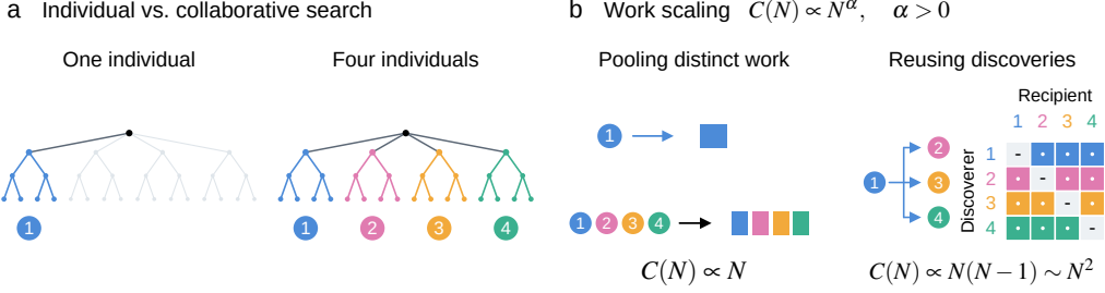
Figure 5: Individual and collaborative search. (a) Multiple individuals can explore different branches of a search tree. (b) For a population of N individuals, pooling distinct work gives C(N) \propto N , while reusing discoveries across individuals can give C(N) \propto N(N-1) \sim N^2 .
