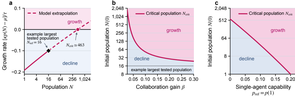
Figure 7: Safety evaluation for a small population does not establish safety at larger populations. Population curves as predicted by our model. (a) Per-unit growth rate (setting \tau = 1 ) is plotted against population, N , with p_{\text{ref}} = 0.10 , p_{\text{crit}} = \mu/\kappa = 0.20 , and \beta = 0.035 . In this case, a laboratory would observe that the population is not capable of growth at its largest tested population, N_{\text{ref}} = 16 (marked by a diamond). However, a population larger than N_{\text{crit}} \approx 463 would be capable of growth. (b) The critical population as a function of the collaboration gain \beta , with p_{\text{ref}} = 0.10 and p_{\text{crit}} = 0.20 held fixed. N_{\text{crit}} is marked in pink; initial populations above the curve grow and initial populations below it decline. For the example reference population size of N_{\text{ref}} = 16 , the population could be in the decline regime even at large collaboration gain. (c) The critical population as a function of the single-agent ( N_{\text{ref}} = 1 ) capability, p_{\text{ref}} = p(1) , with \beta = 0.035 and p_{\text{crit}} = 0.20 held fixed. As in panel (b), populations above the pink N_{\text{crit}} boundary grow and populations below it decline. Increasing single-agent capability lowers the critical population.
