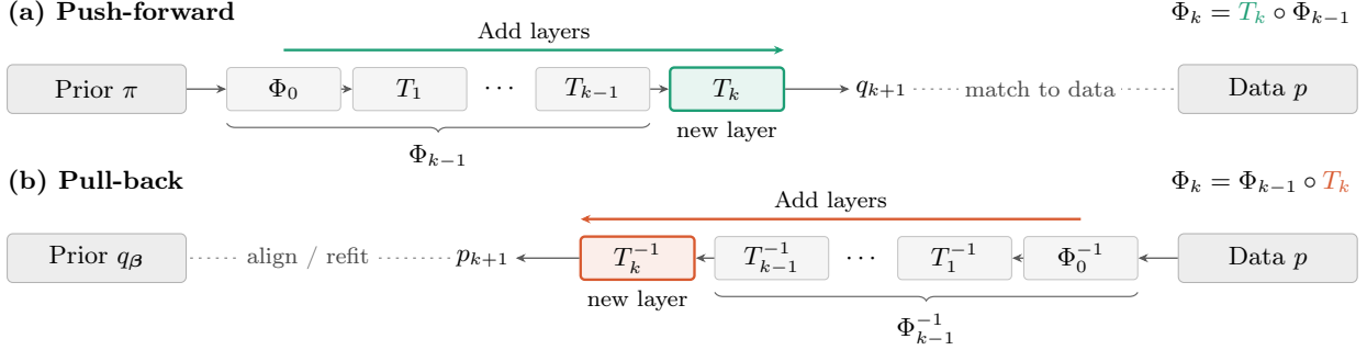
Figure 1: Layer construction in the push-forward and pull-back algorithms. Push-forward appends T_k to the model output; pull-back applies T_k^{-1} to the current latent samples and refits the base between layers. In both panels, \Phi_k maps the latent base to data.
