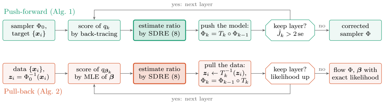
Figure 2: Iteration loops for the two inference algorithms of Section 4.
