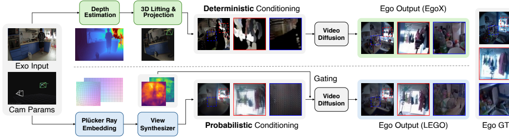
Figure 3: Condition generation. EgoX estimates depth, lifts the exocentric video into a point cloud, and re-renders it along the egocentric trajectory; LEGO renders the egocentric view directly with a frozen synthesizer.
