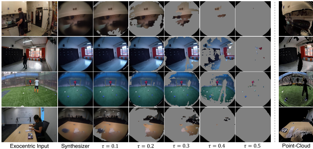
Figure 7: Effect of the gate threshold. The synthesizer render gated at \tau = 0.1, \dots, 0.5 , shown between the ungated render and the point-cloud render of Kang et al. (2026).
