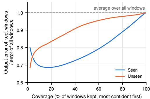
Figure 5: Confidence is informative. Windows of the generated video are sorted by confidence; the curve is the error of the most confident fraction relative to all windows, on Ego-Exo4D. Dashed: the average over all windows.
