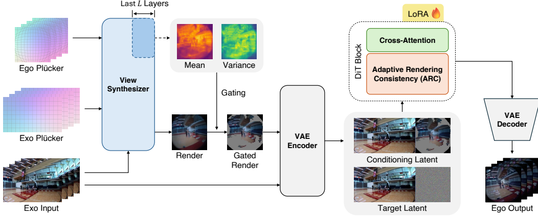
Figure 2: Overview of LEGO. The frozen synthesizer F renders the egocentric view once per latent frame and exposes a confidence map. The render, gated to gray where confidence is low, fills the egocentric half of the conditioning latent; the confidence also drives ARC during the early denoising steps. The generator is unchanged.
