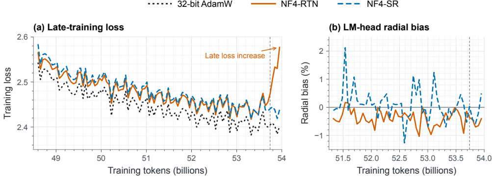
Figure 4: Late-training instability and LM-head directional bias in GPT-style 2.7B pretraining. (a) Cooldown training loss averaged in 100-update bins; NF4-SR uses SR on the LM-head first moment. (b) Radial bias b_{\text{rad}}(\tilde{\mathbf{m}}_t) logged every 100 steps, with FP32 non-head first moments and Dyn4/Update-SR second moments. The vertical dashed line marks the first global gradient-clipping event of the NF4-RTN continuation.
