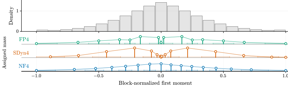
Figure 3: Empirical distribution of block-normalized FP32 first-moment values from the layer-12 MLP up-projection at step 15,908 of GPT-style 834M pretraining, together with the probability mass assigned to each reconstruction level by FP4, SDyn4, and NF4 under RTN.
