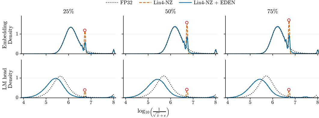
Figure 5: Matched next-step preconditioner distributions at 25%, 50%, and 75% of training. Columns show checkpoints and rows show embedding and LM-head states. Curves compare FP32, Lin4-NZ, and Lin4-NZ with EDEN; open circles mark the Lin4-NZ floor atom.
