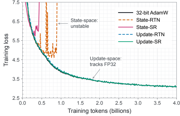
Figure 1: Rounding space controls training stability. Training loss over the first 4B tokens of GPT-style 834M pretraining, with FP32-m and zero-inclusive Dyn4-v. State-RTN/SR become unstable and exceed the plotted range, while Update-RTN/SR closely track 32-bit AdamW.
