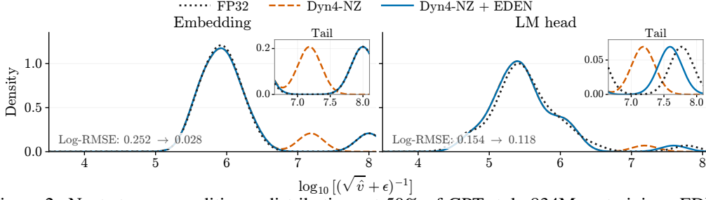
Figure 2: Next-step preconditioner distributions at 50% of GPT-style 834M pretraining. EDEN partially restores the large-preconditioner tail suppressed by Dyn4-NZ in the embedding and LM-head states. Log-RMSE measures coordinate-wise error from FP32.
