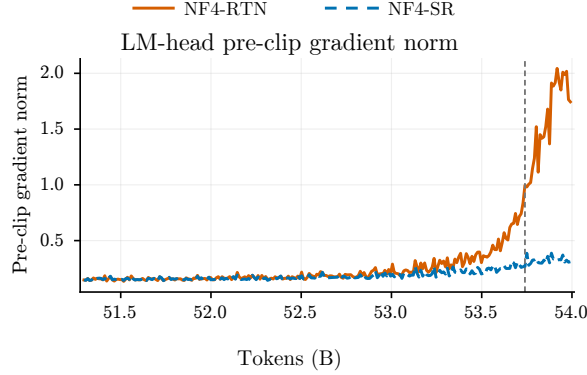
Figure 6: LM-head gradient growth in the matched continuations. The solid orange curve denotes NF4-RTN and the dashed blue curve denotes NF4-SR. The vertical dashed line marks step 102,500 (53.74B tokens), at which the NF4-RTN continuation first triggers global gradient clipping.
