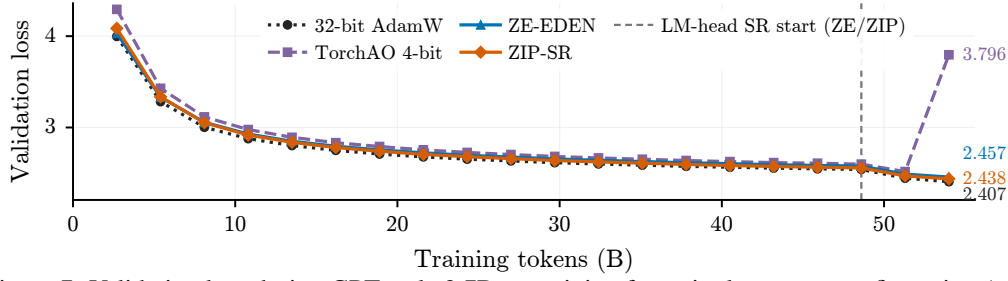
Figure 7: Validation loss during GPT-style 2.7B pretraining for a single run per configuration (seed 42). The dashed line marks the switch from NF4-RTN to NF4-SR for the LM-head first moment at 90% of training in ZE-EDEN and ZIP-SR. TorchAO exhibits a sharp regression, whereas ZE-EDEN and ZIP-SR remain close to 32-bit AdamW.
