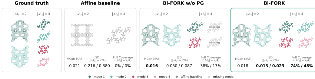
Figure 6: Mechanical metamaterials result comparison. Ground truth modes and generated samples are shown for representative conditions with |\mathcal{M}_c| = 2 and |\mathcal{M}_c| = 4 buckling modes. Colors indicate the mapped ground-truth mode; missing modes are shown in gray. Affine baseline results in mean prediction. Reported MCon-MAE is averaged over the full test set, while JSD and full coverage are reported for |\mathcal{M}_c| \in \{2, 4\} . Metrics reported over five random seeds on the test dataset.
