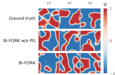
Figure 8: Visual comparison of ground truth vs predicted samples for \mu = 0.86 and \epsilon = 0.094 .
