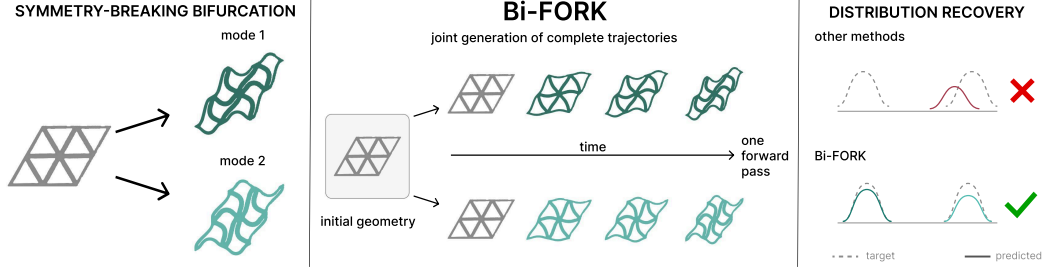
Figure 1: Learning bifurcating solution distributions. Left: Symmetry breaking results in multiple valid trajectories for the same control parameter and initial state. Center: Latent flow matching jointly samples trajectories and resolves distinct branches in one forward pass. Right: Unlike mode-averaging baselines, Bi-FORK recovers the target distribution.
