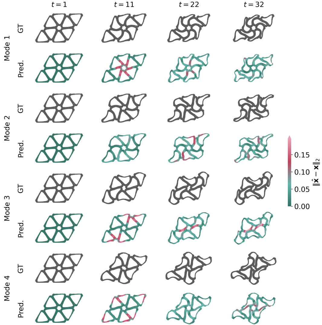
Figure 16: Visualization of a four-mode sample generated by Bi-FORK with K = 16 . The ground truth is compared with the closest predicted mode.
