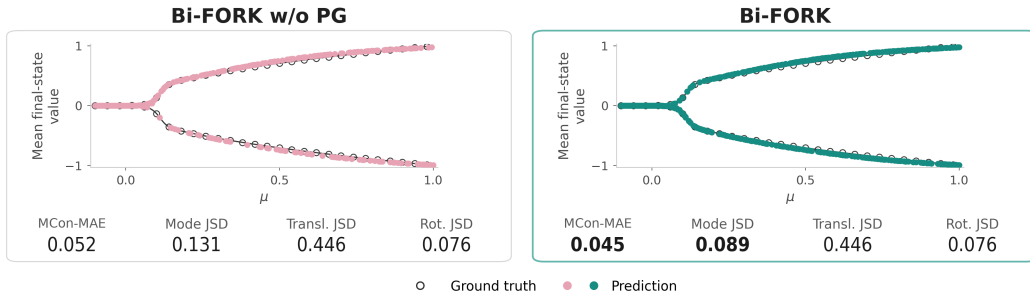
Figure 7: Allen-Cahn result comparison. Ground truth (black open circles) and predictions (teal and pink circles) are shown across a parameter sweep \mu \in [-0.1, 1.0] at fixed \epsilon = 0.1 . The vertical axis shows the final-frame mean value. We evaluate metrics on the test dataset and average over five random seeds; lower values indicate better performance.
