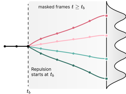
Figure 4: Particle guidance during sampling. Trajectories evolve identically up to bifurcation point t_b . From t_b , the repulsion term acts on the masked frames t \geq t_b , pushing the K trajectories apart, yielding a multimodal distribution.
