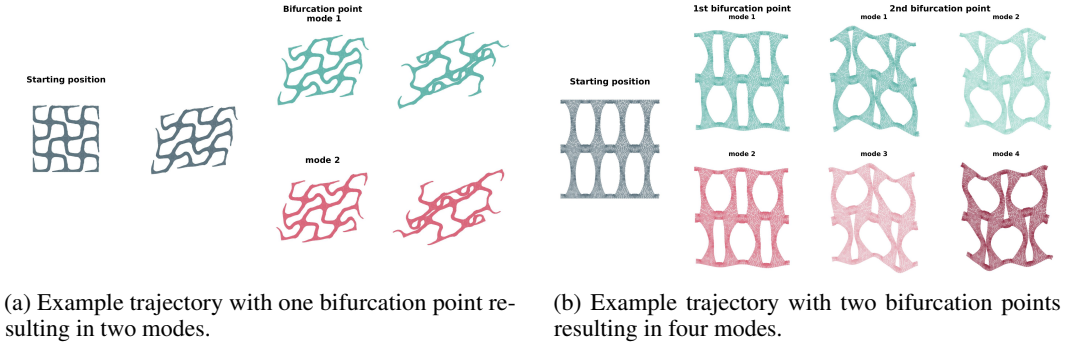
Figure 10: Example mechanical metamaterials trajectories with distinct post-buckling mode structures.
