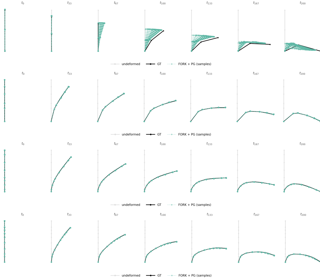
Figure 12: Beam bending process: showing predicted (green) vs actual (black) trajectory evolution for 180 samples. Node count ranging from 3 to 11 nodes
