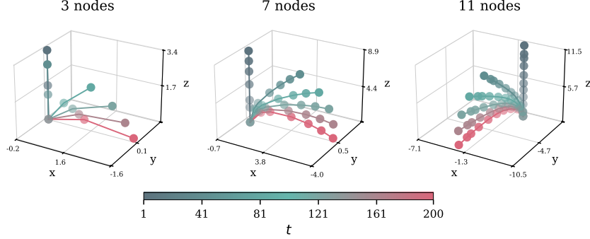
Figure 9: Example trajectories from the 3D beam dataset with different buckling directions \phi for diverse node counts over timestep t .
