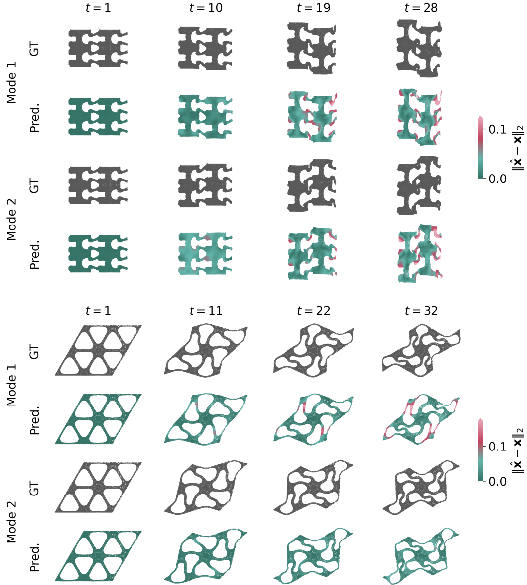
Figure 15: Visualization of two-mode samples generated by Bi-FORK with K = 16 . The ground truth is compared with the closest predicted mode.
