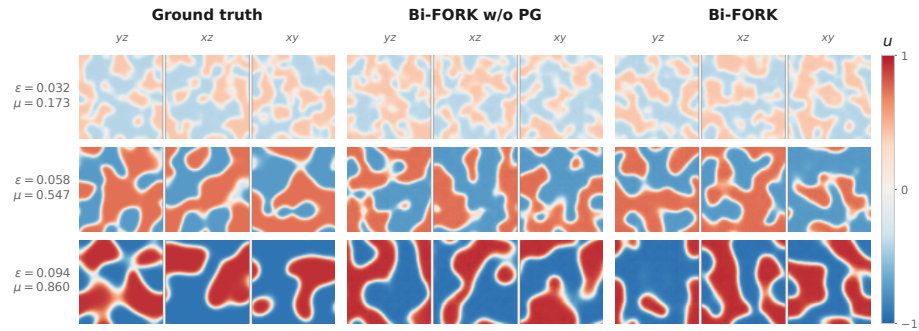
Figure 13: Sample comparison for increasing \mu and \epsilon , showcasing the diversity of potential solutions compared to the ground truth.
