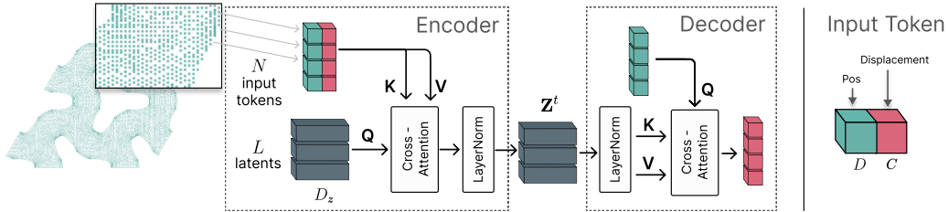
Figure 3: Encoder-decoder structure for point cloud datasets. Input tokens (reference positions \mathbf{X}^1 and displacements) are encoded into latent representation by cross-attending to L learned latent query tokens. The decoder reconstructs the displacements conditioned on the reference positions.
