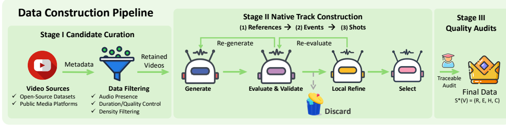
Figure 2: OmniCapBench data construction pipeline. The construction proceeds in three stages. Stage I filters raw videos to isolate inputs with rich audio–visual complexity. Stage II generates atomic units (References \rightarrow Events \rightarrow Shots) through an iterative multi-model loop, enforcing structural integrity before semantic refinement. Stage III applies traceable human audits to finalize the rigorously verified audio–visual reference system.
