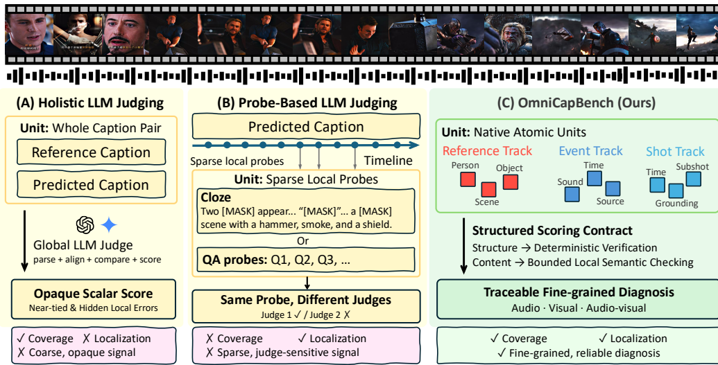
Figure 1: Comparison of existing evaluation frameworks and the deep-structured evaluation framework. Both (A) Holistic Evaluation and (B) Probe-Based Evaluation derive scores from predicted unstructured, free-form text captions, but introduce distinct limitations. The former uses a global LLM-judge approach that treats the caption as a whole, resulting in an opaque score that masks local errors and lacks granularity, whereas the latter adopts a QA-probe approach to detect local errors but sacrifices global coverage and introduces instability across different LLMs. (C) OmniCapBench (Ours) proposes a deep-structured evaluation framework. The caption is first natively represented as atomic, verifiable audio-visual units. Deterministic rules then verify structural and temporal relationships and dispatch these aligned units to localized, reliable LLMs to perform fine-grained semantic checks. This design preserves comprehensive coverage and achieves fine-grained error localization while eliminating the uncertainty associated with global LLM-based judges.
