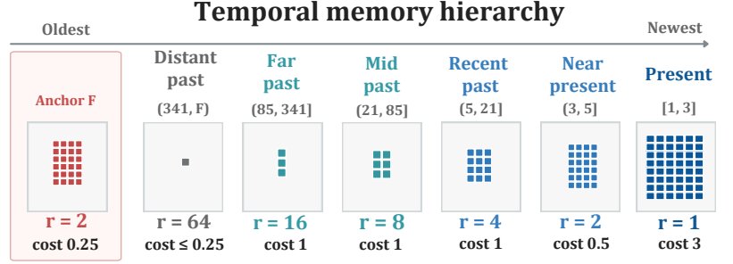
Figure 3: Longest-history branch ( 343 \leq F \leq 1366 ). Age 1 is newest; age F is the anchor. Rates r denote spatial reduction relative to base patch embedding, and costs are nominal latent-frame equivalents before spatial padding, with the separately embedded reference adding cost 1 at r = 1 . Shorter branches appear in Appendix C.3.
