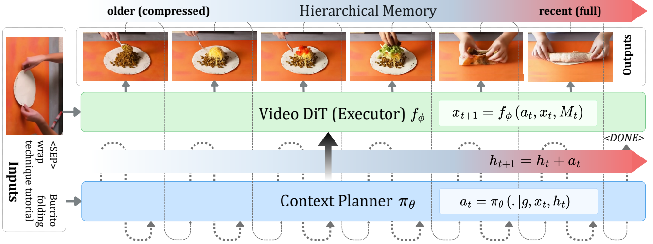
Figure 2: Overview of WorldGuide. Given the initial image x_0 , task goal g , and the latest K=3 clip-action pairs h_t , the ContextPlanner \pi_\theta predicts the next atomic action a_t or DONE. The Executor f_\phi renders a_t into the next clip x_{t+1} from the current visual state x_t and hierarchical memory M_t , which progressively compresses older latent frames. Each new clip x_{t+1} becomes the next visual state, is paired with a_t in the history h_{t+1} , and updates the memory M_{t+1} , and the loop continues until DONE is predicted or the step budget is reached. Notation follows Eq. 1.
