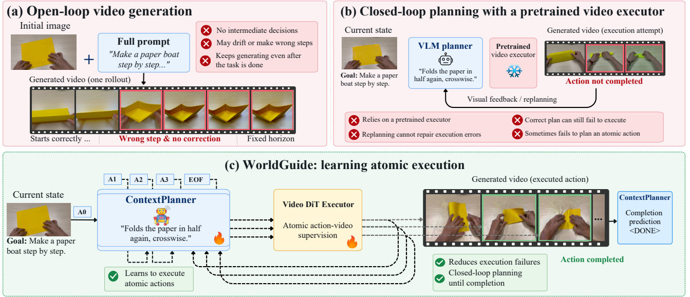
Figure 1: From open-loop synthesis to learned procedural execution. (a) Open-loop generation follows a fixed prompt with no intermediate decisions, so it can drift into a wrong step and keep generating after the task is done. (b) A planner can inspect outcomes and replan, but with a frozen pretrained executor, a correct instruction can still fail to execute. (c) WorldGuide trains the ContextPlanner and Executor on the same demonstrations, the Executor conditioned on the planner’s action embeddings. Thus, generated outcomes guide the next action and the decision to stop.
