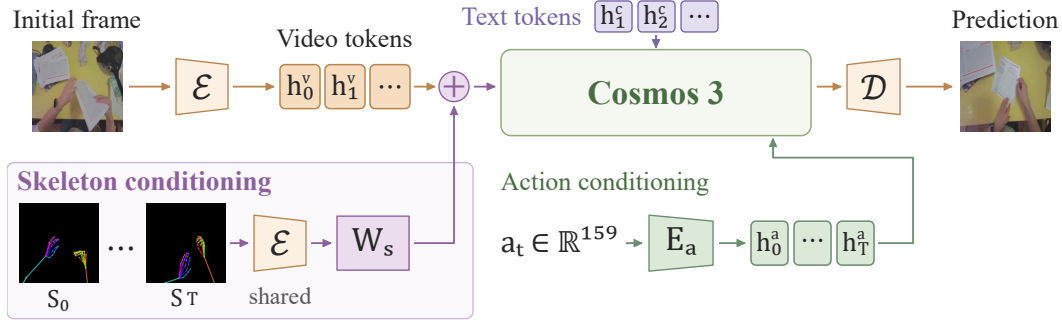
Figure 2: Cosmos 3 with skeleton conditioning. The projected skeleton sequence S_{0:T} , shown in bottom left, is encoded by the same frozen VAE \mathcal{E} as the video, and its latent patches are projected through a zero-initialized W_s and added to the corresponding video embeddings. The skeleton is derived from the camera intrinsics to better align agent’s actions with the visual token grid.
