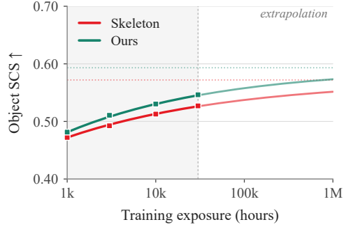
Figure 5: A higher object ceiling. Object fidelity across the data ladder, with and without dynamic-region supervision. Ours exceeds the skeleton baseline at every budget, and converges to a higher limit.
