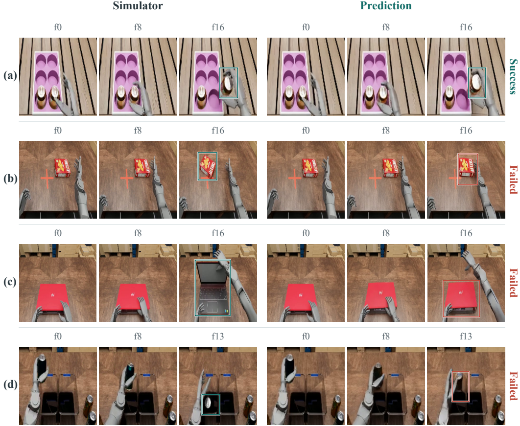
Figure 10: One successful humanoid rollout and three object interaction failures. Each row shows one example, with simulator’s frames on the left and the corresponding predictions of our world model on the right. (a) Both rollouts unload the can within the shown window. (b) In the simulator the box turns, while in the world model it stays in place. (c) In the simulator the laptop opens, while the world model leaves it closed. (d) In the simulator the can drops in the bin, while in the world model’s predictions it remains stuck near the bin’s edge. Frame indices are aligned across each pair, with a common crop throughout. Success labels indicate whether the world model’s prediction matches the simulator’s object response. Best viewed on the project website.
