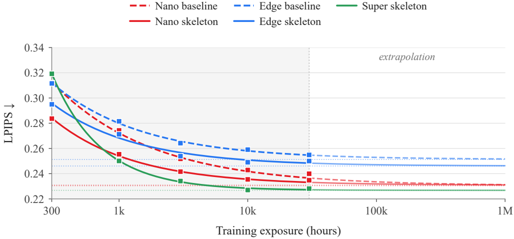
Figure 11: Perceptual quality across the data-scaling ladder. LPIPS (lower is better) versus training exposure. Further scaling of ego-centric data is unlikely to improve the perceptual quality of the model’s predictions either.
