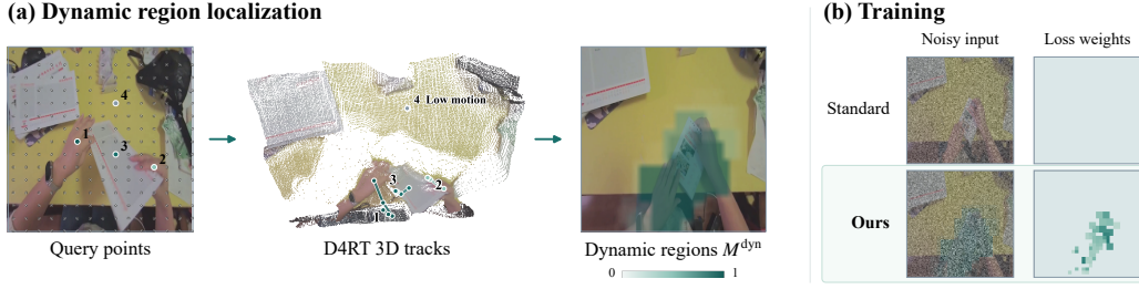
Figure 12: Dynamic-region supervision. (a) D4RT tracks queried points in 3D to separate scene motion from camera motion. We combine 3D motion, tracking reliability, and a soft spatial prior around the hands to obtain the dynamic region map M^{\text{dyn}} . (b) Dynamic-region supervision combines dynamic noise scheduling and loss reweighting in selected regions.
