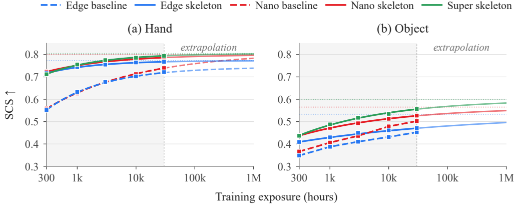
Figure 4: Scaling reaches the agent’s limit, not the object’s. SCS for the agent (left) and manipulated objects (right) versus training data, with and without skeleton conditioning. Skeleton conditioning reaches the agent’s limit with far less data, while object fidelity converges far below.
