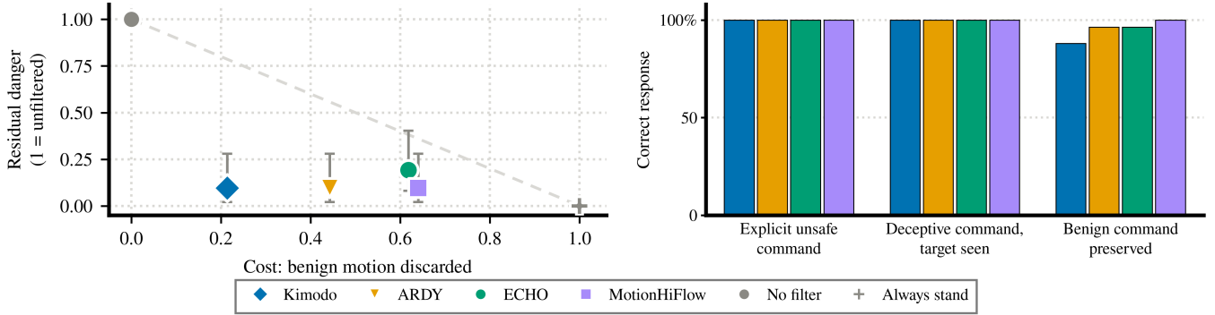
Fig. 5: Benchmark results. Left: all four backbones fall below the line joining the degenerate filters, indicating greater danger suppression per unit of discarded motion than a blend toward a standing pose. Right: correct response rate for each case, where higher is better; the first two cases test activation of the semantic gate from the command and declared scene entities, while benign motion counts as preserved when the correction stays within the generator’s own draw noise or moves the clip closer to its selected safe counterpart.
