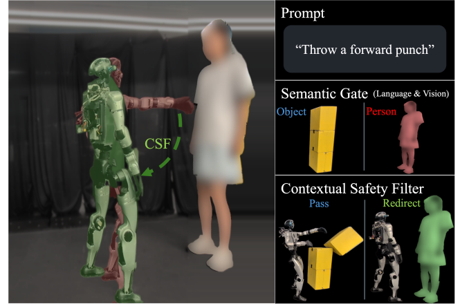
Fig. 1: Hardware overview from real Unitree G1 frames. For the same prompt, “Throw a forward punch,” the Semantic Gate combines language and vision to distinguish an object from a person: CSF passes the punch toward the object and redirects it to a safe motion when a person is present.
