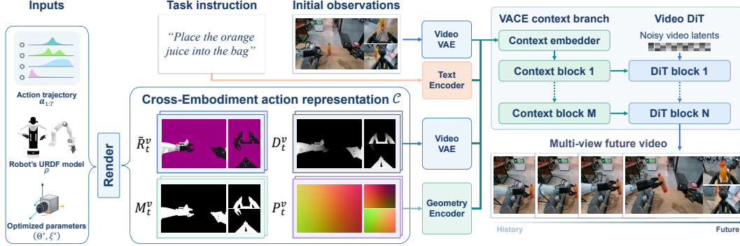
Figure 3: Unified multi-view world model. Robot renderings, gripper openings, and camera rays condition the video DiT through a VACE branch to predict multi-view future videos.
