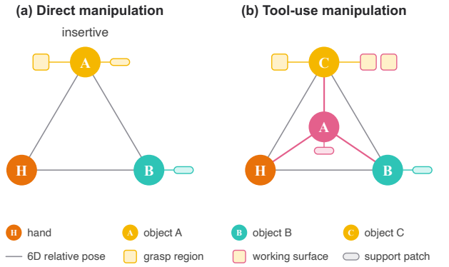
Figure 9: Scene-graph-grounded observation. The policy observation is constructed from scene-graph nodes and their relative 6D-pose edges for (a) direct and (b) tool-use manipulation.
