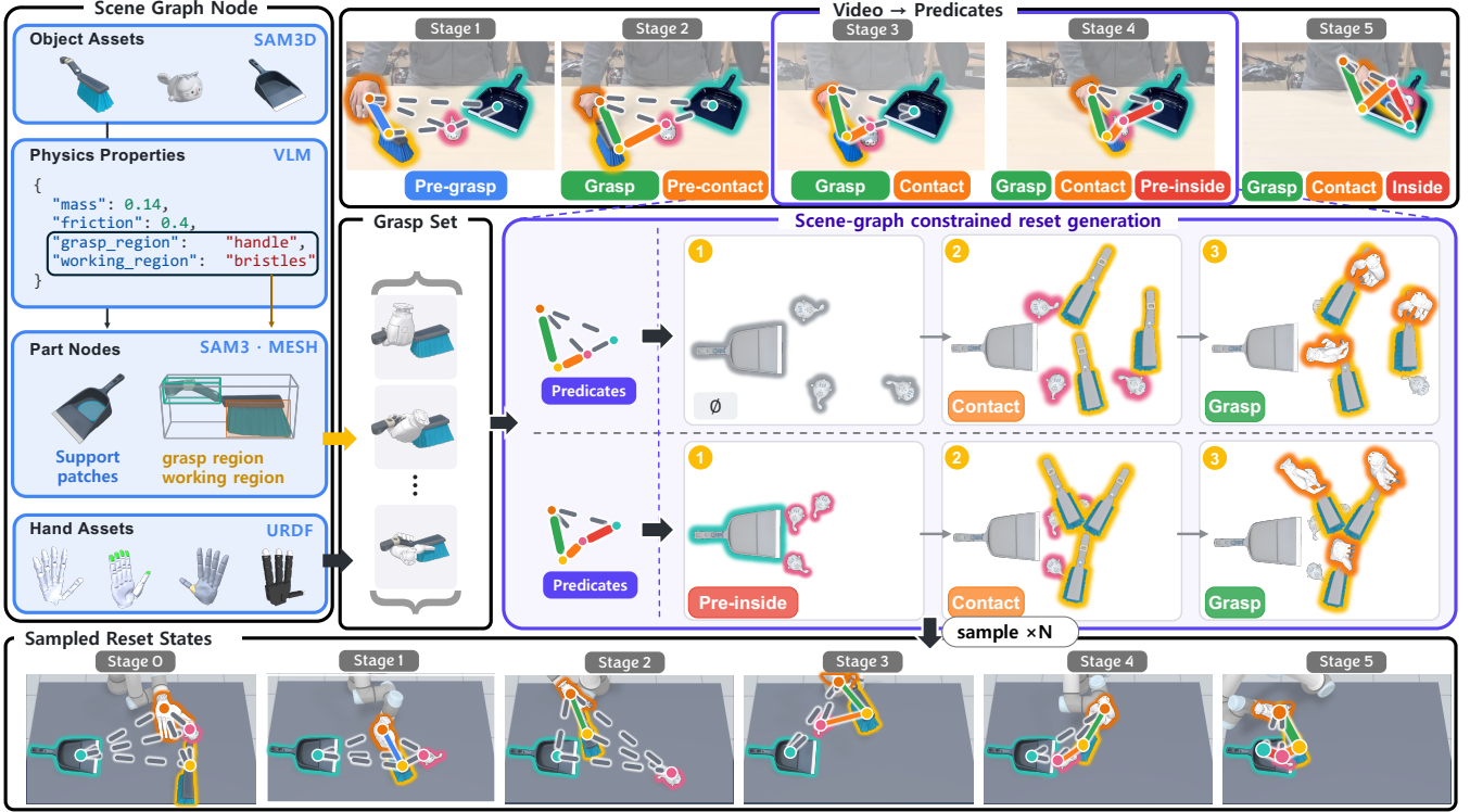
Figure 10: Scene-graph-constrained reset generation. Given the stage-wise scene graph and the assets, we instantiate each task stage as diverse reset states. The object and hand assets provide geometry and physical properties, while functional part nodes identify regions such as grasp and working regions. Together, these are used to construct a grasp set, restricted to the specified grasp region when available. For each stage, predicates in the scene-graph act as generative constraints: geometric predicates determine where related entities can be sampled, while the grasp predicate samples a valid hand–object configuration from the grasp set. Repeating this process produces diverse simulation reset states that satisfy the relations specified by each stage graph.
