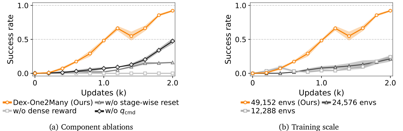
Figure 7: Ablation studies. (a) Removing each component. (b) Varying the number of environments.
