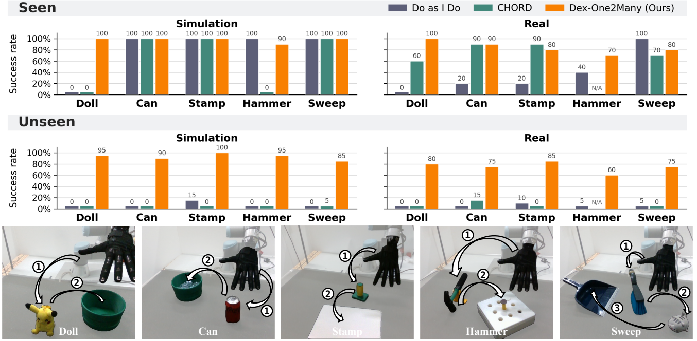
Figure 4: Generalization beyond the human video in simulation and the real world. Success rates are reported for configurations shown in the input human video ( Seen , top) and configurations with different initial and goal poses not shown in the video ( Unseen , bottom), in both simulation and the real world. The bottom row illustrates the five evaluated tasks; N/A denotes an experiment unavailable due to a hardware failure.
