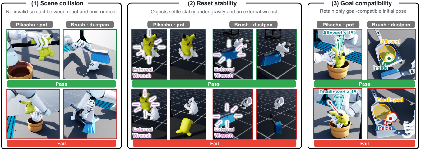
Figure 11: Physical verification of reset candidates in the Sweep task. (1) and (2) (top: pass, bottom: fail), and (3) is enforced over grasp types. (1) Scene collision : the robot makes no invalid contact with the table or other objects; the failing candidate collides with the dustpan. (2) Reset stability : objects settle under gravity and the grasped object stays in the hand under external wrenches; the failing grasp drops the brush. (3) Goal compatibility : the goal relation remains attainable with the candidate grasp; the failing candidate cannot bring the toy cat inside the allowed region of the dustpan.
