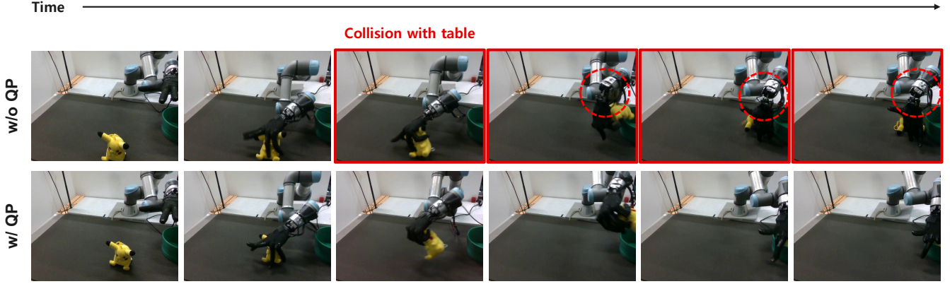
Figure 12: QP constraints address a hardware-specific sim-to-real gap. Hand–table contact is benign in simulation because coupler disengagement is not modeled, but the same contact can disengage the Wuji 1 hand coupler on the physical robot. Without the QP low-level controller (top), the learned policy encounters this failure mode. With the QP controller (bottom), a hand–table clearance constraint prevents the collision without retraining the task-space policy.
