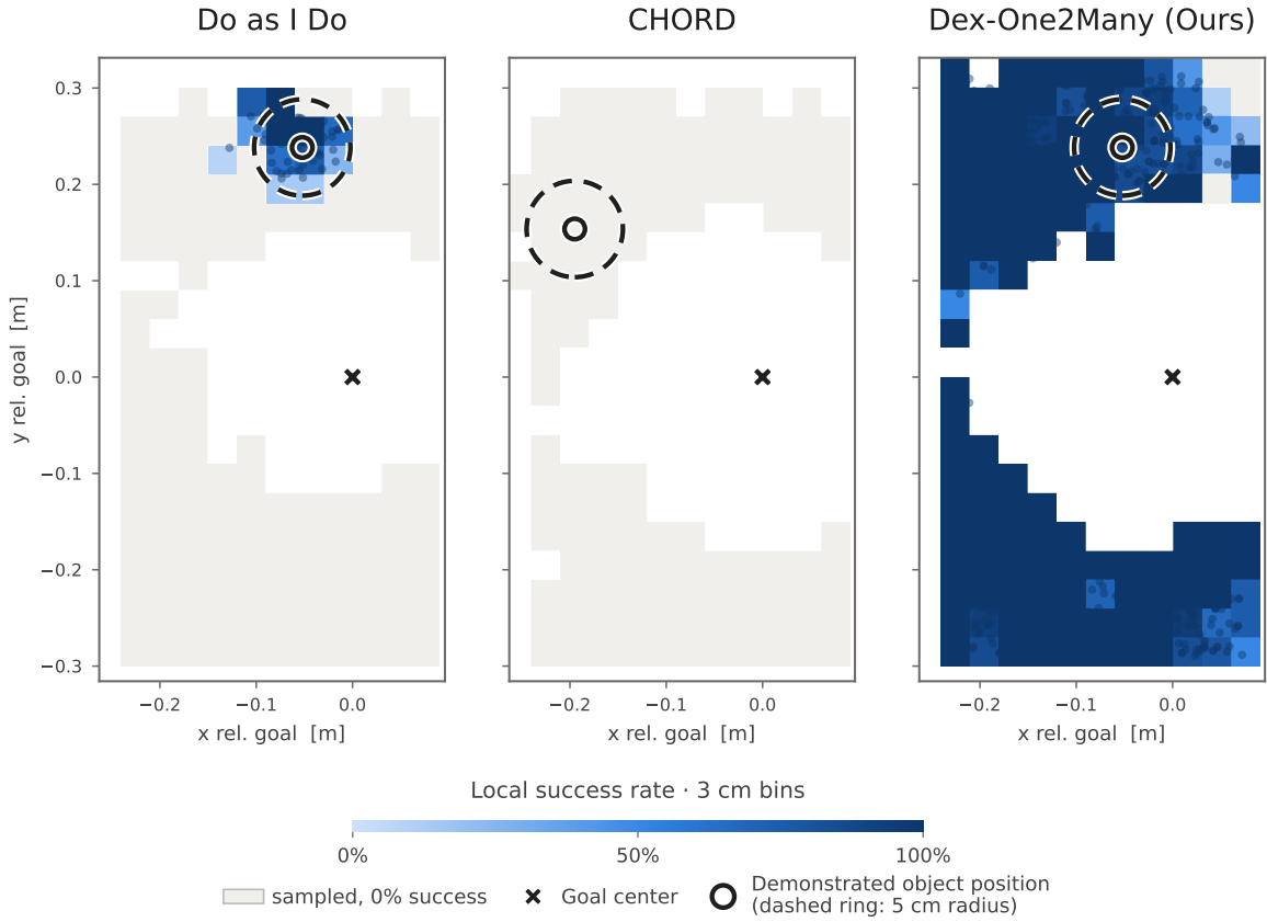
Figure 16: Generalization to unseen initial object positions on the Hammer task. With the goal fixed, Dex-One2Many succeeds over a substantially broader range of initial positions than the baselines.
