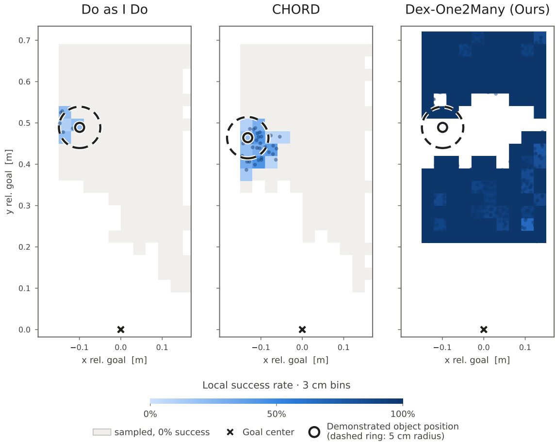
Figure 17: Generalization to unseen initial object positions on the Sweep task. With the goal fixed, Dex-One2Many succeeds over a substantially broader range of initial positions than the baselines.
