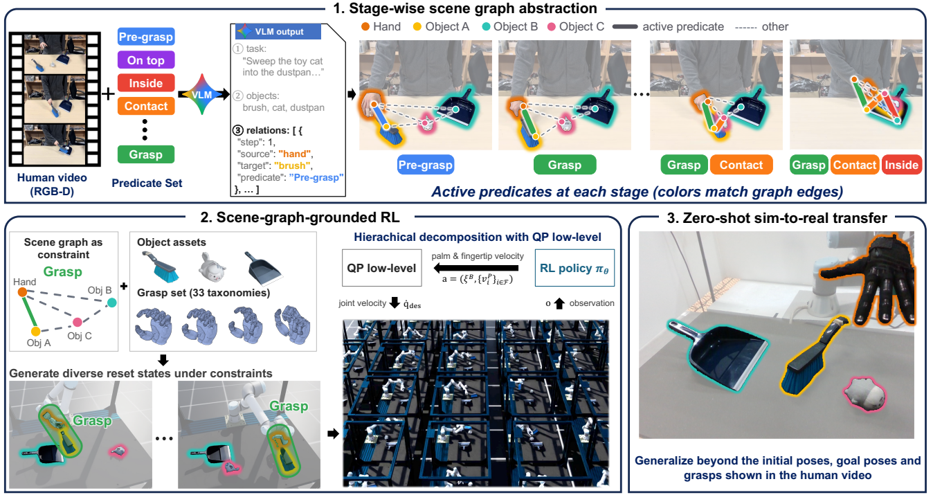
Figure 2: Overview of Dex-One2Many. (1) From a single human video, a VLM extracts a stage-wise scene graph of object relations. (2) Each stage graph constrains the sampling of object poses and synthesized grasps, yielding verified reset states for every stage. An RL policy trained from these resets with predicate-derived rewards acts in task space through a QP controller. (3) The policy transfers zero-shot to unseen initial poses, goal poses, and grasps on real hardware.
