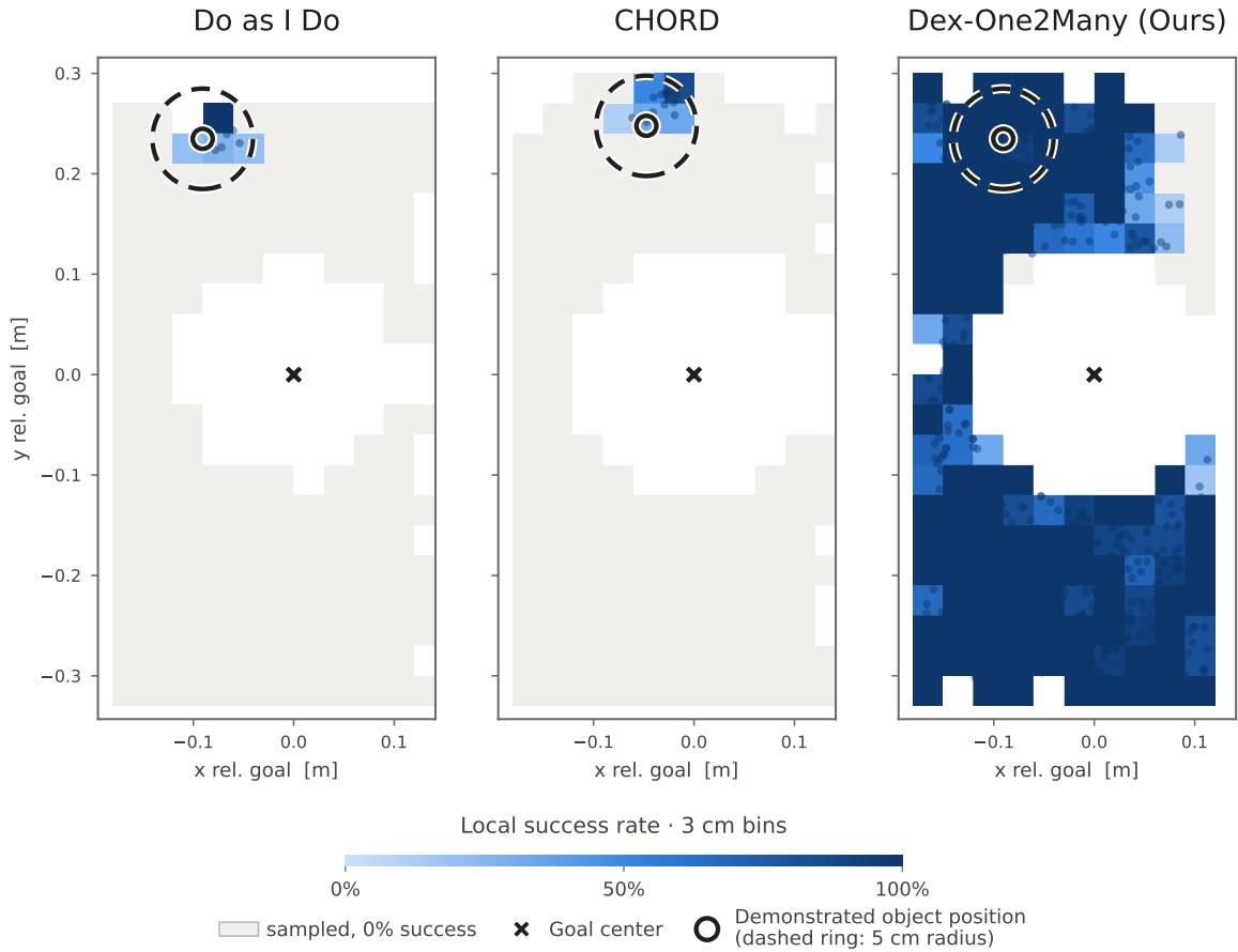
Figure 14: Generalization to unseen initial object positions on the Can task. With the goal fixed, Dex-One2Many succeeds over a substantially broader range of initial positions than the baselines.
