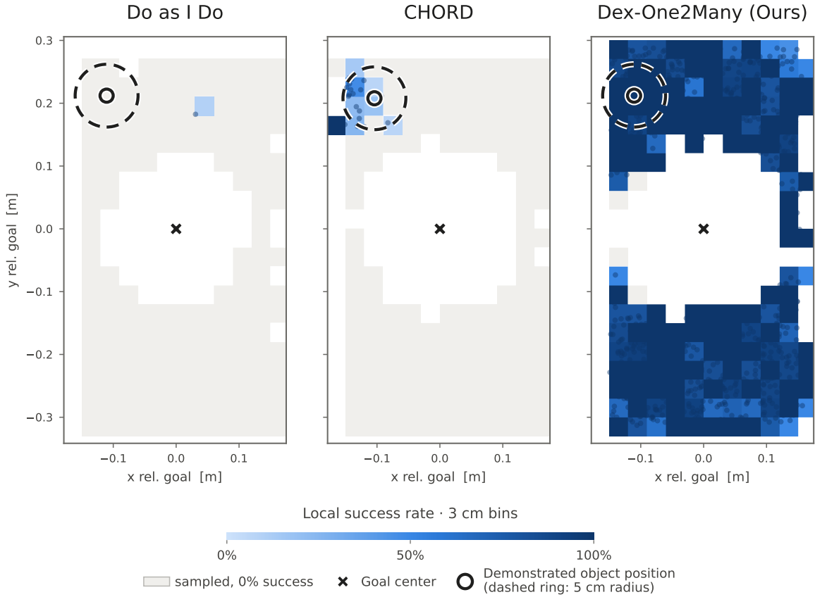
Figure 13: Generalization to unseen initial object positions on the Doll task. With the goal fixed, Dex-One2Many succeeds over a substantially broader range of initial positions than the baselines.
