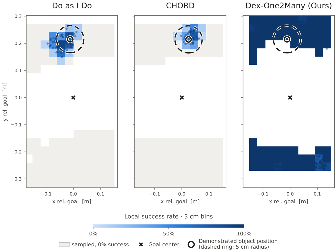
Figure 15: Generalization to unseen initial object positions on the Stamp task. With the goal fixed, Dex-One2Many succeeds over a substantially broader range of initial positions than the baselines.
