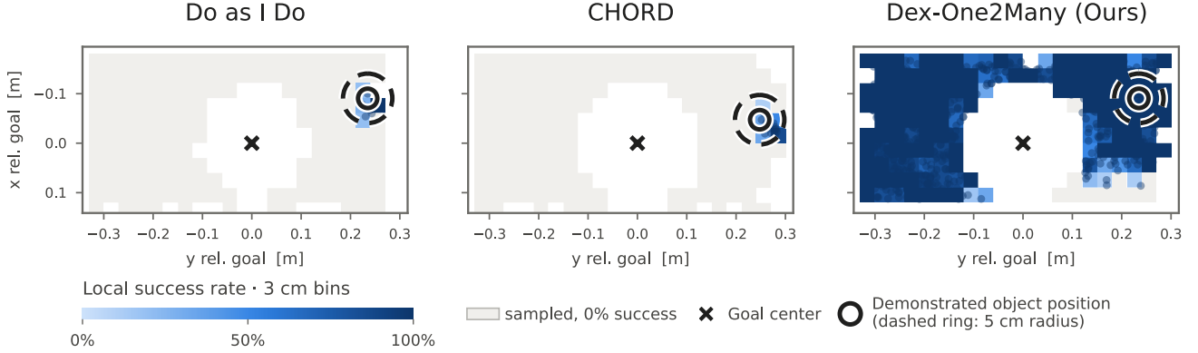
Figure 5: Generalization to unseen initial object positions on the Can task. In simulation with the goal fixed, Dex-One2Many succeeds across a broader range of initial positions than the baselines.
