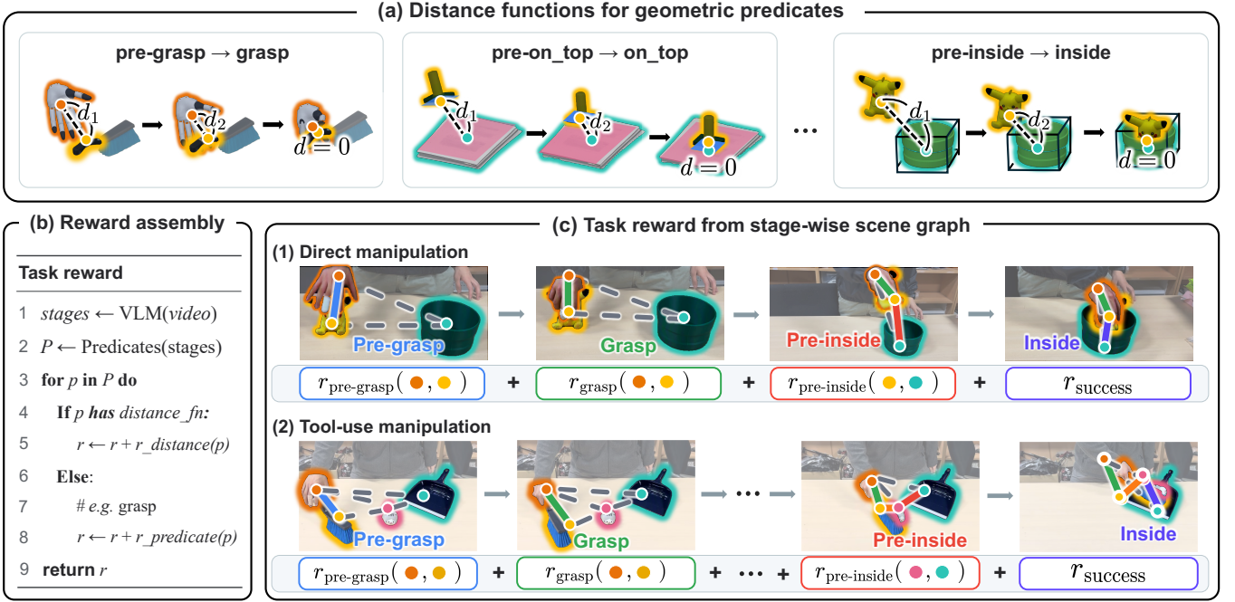
Figure 3: Using scene-graph predicates for policy learning. (a) Predicates that can be expressed geometrically are mapped to Cartesian-space distance functions. (b) The predicates in a stage-wise scene graph determine which reward terms are assembled into the task reward. (c) The same assembly rule is instantiated for direct and tool-use manipulation from their respective scene graphs.
