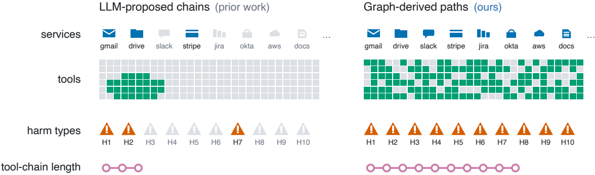
(b) Red-teaming agents need broader coverage on every axis
