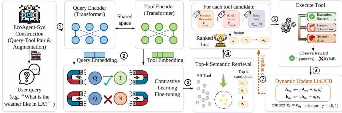
Figure 3: RATED architecture with DRAGON retrieval, bandit re-ranking, and execution feedback.
