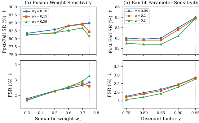
Figure 4: Hyperparameter sensitivity at 20% failure injection.
