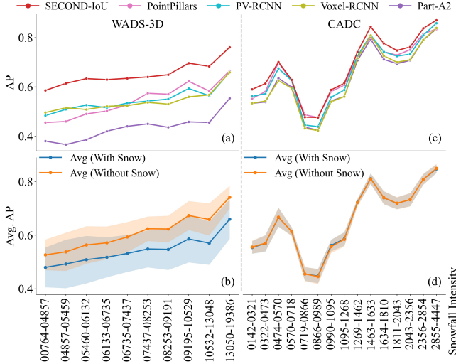
Figure 4: Impact of snowfall intensity on object detection performance in WADS-3D (left) and CADC (right). Top row (a,c): AP of five individual models under snowy conditions across increasing intensity. Bottom row (b,d): Ablation study, comparing the mean AP of all models with snow (blue) vs. without snow (orange) across the same intensity bins. Shaded regions indicate standard deviation.
