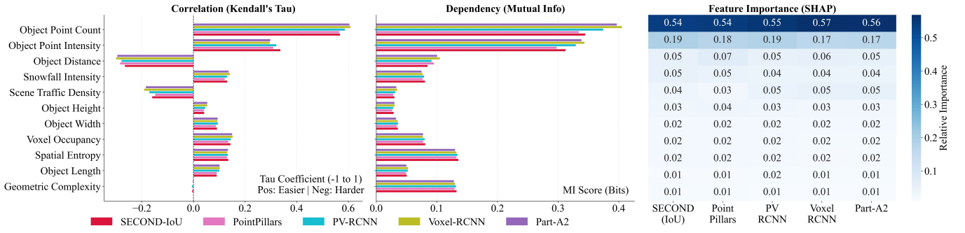
Figure 8: Kendall’s Tau correlation, Dependency (MI), and Feature importance (SHAP) for recall analysis on CADC.
