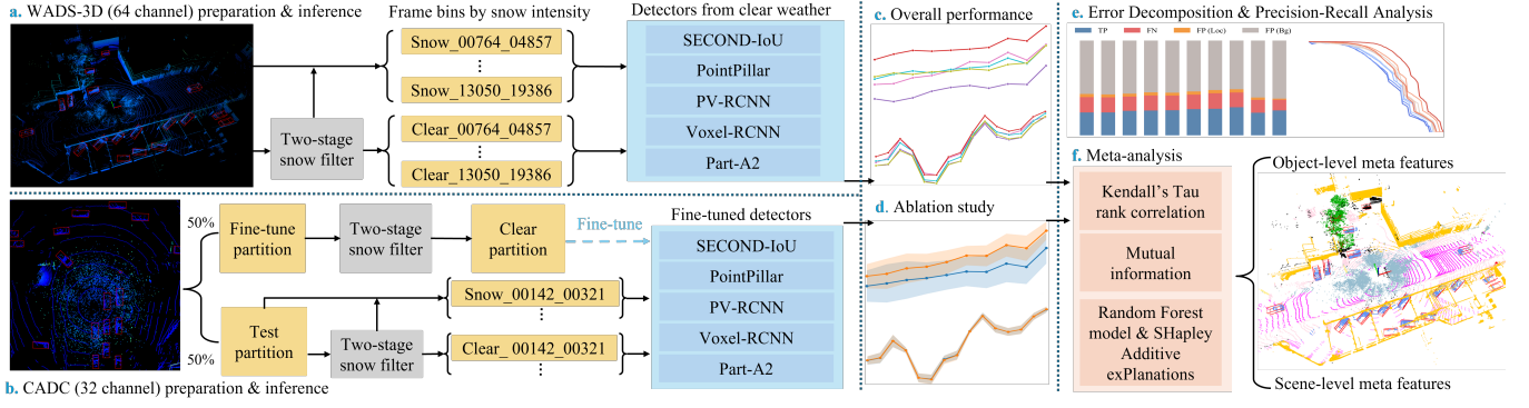
Figure 3: Lidar-only 3D object detection pipeline, including the following sequential stages: (a) WADS-3D preparation: We binned the lidar frames using a two-stage snow filter, generating snow-filtered bins and original snow bins. We then directly applied five KITTI-trained detectors (which use a 64-channel LiDAR setting) to these groups. (b) CADC fine-tuning: We split the CADC dataset 50:50 for fine-tuning and testing, respectively. We first fine-tuned the models for 32-channel capability and then used the fine-tuned detectors for evaluation. (c) Overall performance: We aggregated and evaluated the detection results inferred by the different detectors on both datasets. (d) Ablation study: We used ablation studies to analyze the influence of varying falling snow intensities. (e) Error decomposition and precision-recall analysis. (f) A three-stage meta-information analysis is carried out on both datasets to identify key influencing meta-features at both the object and scene levels.
