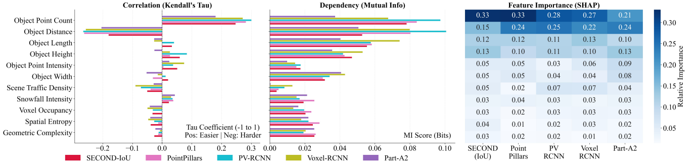
Figure 7: Kendall’s Tau correlation, Dependency (MI), and Feature importance (SHAP) for recall analysis on WADS-3D.
