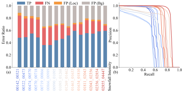
Figure 6: Normalized error distribution and PR-curve across varying snowfall intensities on CADC.
