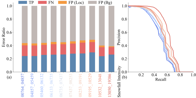
Figure 5: Normalized error distribution and PR-curve across varying snowfall intensities on WADS-3D.
