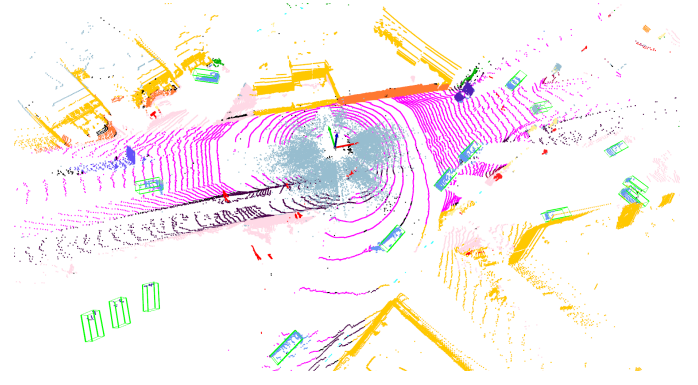
Figure 1: A labeled frame from WADS-3D, with points colored according to the SemanticKITTI style. Cars are indicated by green bounding boxes.
