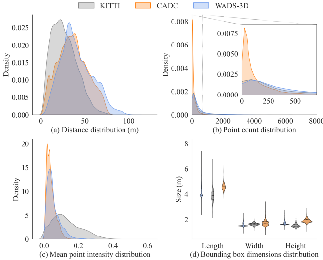
Figure 2: Key object attributes comparison among the KITTI, CADC, and WADS-3D datasets. (a) Car distance distribution, showing WADS-3D and CADC observe vehicles at greater average distances. (b) LiDAR points-per-car distribution, highlighting a higher point count in WADS-3D, followed by KITTI and CADC; the lower count in CADC is attributable to its 32-channel lidar. (c) Mean LiDAR intensity distribution, indicating lower intensity values for the snowy CADC and WADS-3D datasets. (d) Car dimensions distribution.
