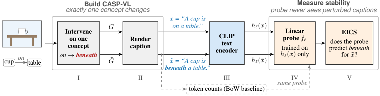
Figure 1: EICS asks whether a representation follows a one-concept change in its input. (I) We edit one concept in a Visual Genome scene graph G , giving \tilde{G} . (II) Both graphs are rendered as captions x and \tilde{x} from one template. (III) The text encoder maps each caption to a hidden state. (IV) A linear probe trained only on original captions (V) is tested on the perturbed ones: EICS is how often it predicts the new label, minus chance. The same probe on token counts (dashed) gives the BoW lexical baseline.
