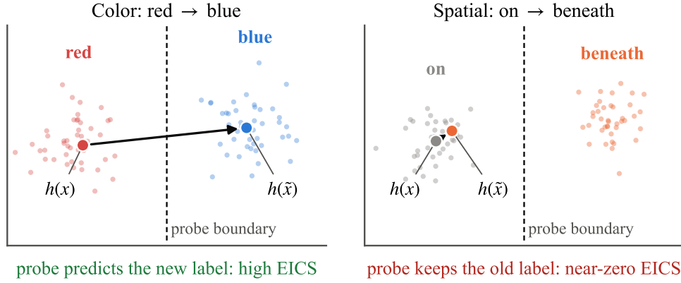
Figure 2: A color flip moves the representation across the probe’s decision boundary; a spatial flip does not. Schematic. Left: flipping “red” to “blue” moves the representation into the blue cluster, so a probe trained on original captions predicts the new label (high EICS). Right: flipping “on” to “beneath” leaves the representation inside the “on” cluster, so the probe still predicts the old label (near-zero EICS).
