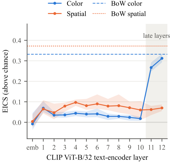
Figure 3: Color becomes decodable in the last two layers; spatial relations stay far below the lexical baseline at every layer. EICS by layer for CLIP ViT-B/32 (12 color classes, 16 relation classes), averaged over five image-grouped splits; bands span the lowest and highest split. Dashed and dotted lines: the BoW baseline for each concept, averaged over the same splits.
