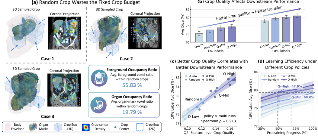
Figure 2: Crop quality matters for 3D medical representation learning. (a) Random cropping frequently spends the fixed crop budget on structure-sparse regions. (b) Policies defined by a semantic quality axis Q_1 yield a monotonic change in downstream Dice. (c) This trend remains under an orthogonal feature-level proxy Q_2 . (d) Better crop quality further improves learning efficiency.
