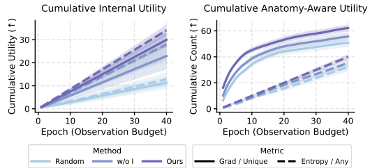
Figure 5: Informativeness analysis. Left: cumulative internal utility, measured by gradient- and entropy-based metrics. Right: cumulative anatomy-aware utility measured by the number of distinct organs observed and any-organ hits.
