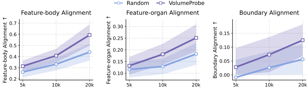
Figure 12: Quantitative analysis of structure-aligned feature responses. We evaluate Random and VolumeProbe at 5k, 10k, and 20k early pretraining iterations using feature responses extracted from the same encoder stage. We report feature-body alignment, feature-organ alignment, and boundary alignment, with shaded regions indicating standard deviation across sampled sub-volumes. VolumeProbe consistently achieves higher alignment scores than Random , supporting the qualitative feature-map observations in Fig. 8(c).
