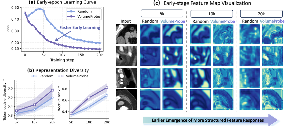
Figure 8: Learning relevance of VolumeProbe. (a) Early-epoch learning curves, where VolumeProbe shows faster and more stable loss reduction. (b) Early representation diversity measured by token-level cosine diversity and effective rank. (c) Feature-map visualization, where VolumeProbe produces more structure-aligned representations.
