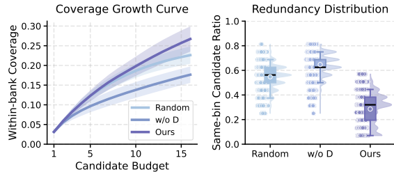
Figure 7: Diversity analysis. Left : within-bank coverage as candidate budget increases. VolumeProbe consistently achieves broader support. Right : same-bin candidate ratio measuring local redundancy. Our approach yields the lowest redundancy.
