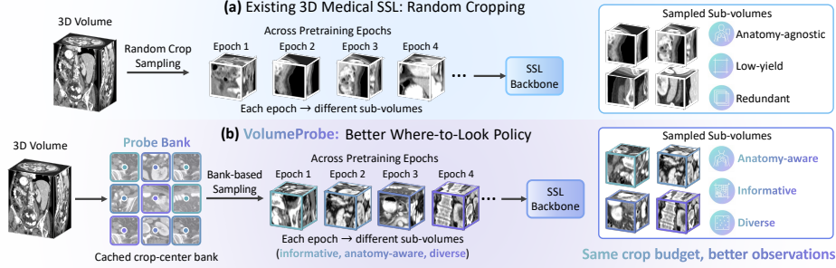
Figure 1: VolumeProbe reallocates the fixed crop budget toward better observations . (a) Random cropping in 3D medical SSL often samples low-yield, anatomy-agnostic, and redundant sub-volumes. (b) VolumeProbe builds a cached probe bank guided by anatomy-awareness, informativeness, and diversity, and samples higher-quality sub-volumes across epochs while keeping the SSL backbone and training objective unchanged.
