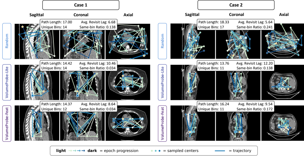
Figure 11: Cross-epoch trajectory analysis. We visualize sampled crop centers across epochs for two representative cases under Random , VolumeProbe-Lite , and VolumeProbe-Feat on sagittal, coronal, and axial views. The light-to-dark trajectory denotes epoch progression, and the inset reports path length, unique bins, average revisit lag, and same-bin ratio.
