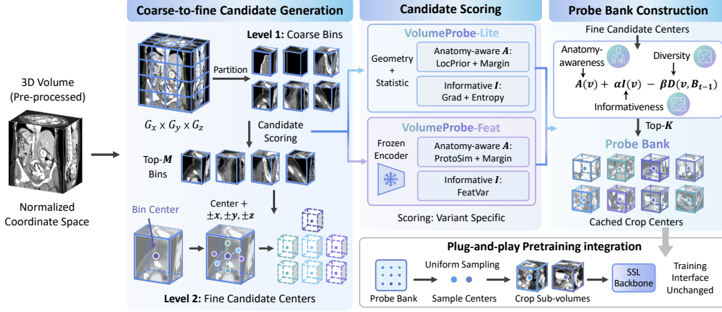
Figure 3: Overview of VolumeProbe. VolumeProbe constructs an offline coarse-to-fine probe bank of normalized 3D crop centers guided by anatomy-awareness, informativeness, and diversity. Pretraining then uniformly samples fixed-size sub-volumes from this cached bank without changing the SSL backbone or objective.
