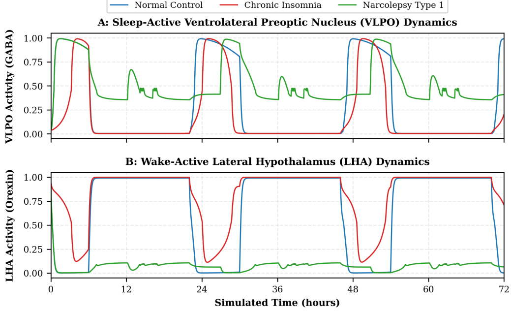
Figure 3: Subcortical Saper reciprocal flip-flop switch dynamics. (A) Sleep-active VLPO GABAergic firing rate V(t) . (B) Wake-active LHA orexin/monoaminergic firing rate A(t) . The normal control displays sharp, bistable transitions with pronounced hysteresis. In contrast, narcolepsy type 1 exhibits crippled LHA tone ( \Omega_{\text{tone}} = 0.05 ), inducing state instability, nocturnal sleep fragmentation, and involuntary daytime transitions.
