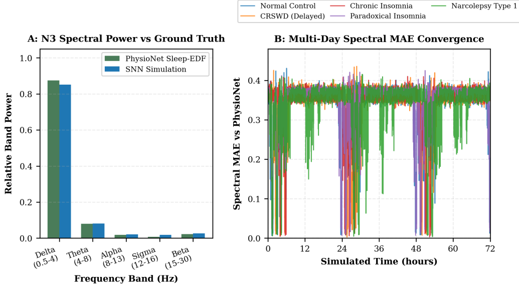
Figure 5: Empirical validation against human PSG from the PhysioNet Sleep-EDF Database (SC4001EO-PSG.edf). (A) Relative spectral band power distribution during stage N3 slow-wave sleep comparing empirical human EEG (channel C3-A2) against the synthetic LFP generated by the recurrent LIF network. (B) Continuous 72-hour Mean Absolute Error (MAE) trajectories across the five clinical cohorts, converging within MAE \approx 0.33–0.35.
