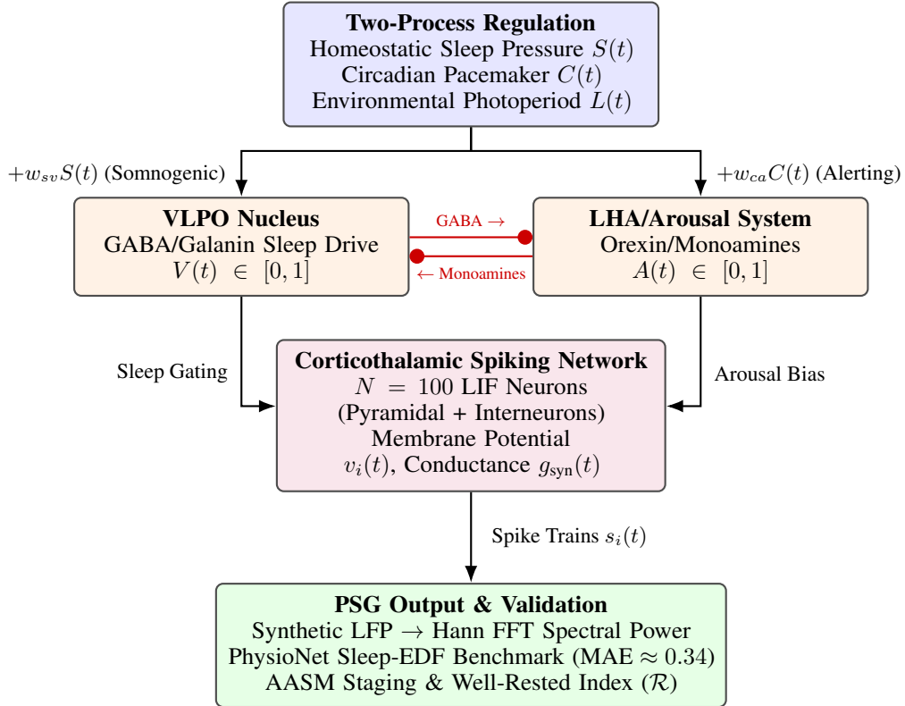
Figure 1: Architectural topology of the DyssomniaNN framework. Borbély’s two-process regulators ( S(t) and C(t) ) drive the reciprocal hypothalamic flip-flop switch (VLPO \leftrightarrow LHA), where +w_{sv}S(t) represents homeostatic somnogenic excitation of the VLPO and +w_{ca}C(t) represents circadian alerting excitation of the LHA. The resulting subcortical arousal level gates the corticothalamic LIF network, whose synthetic LFP is evaluated against empirical PSG spectra from the PhysioNet Sleep-EDF database.
