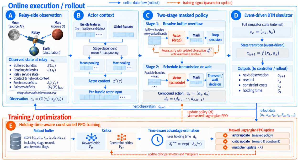
Fig. 2. Masked Lagrangian PPO architecture for event-driven relay control.
