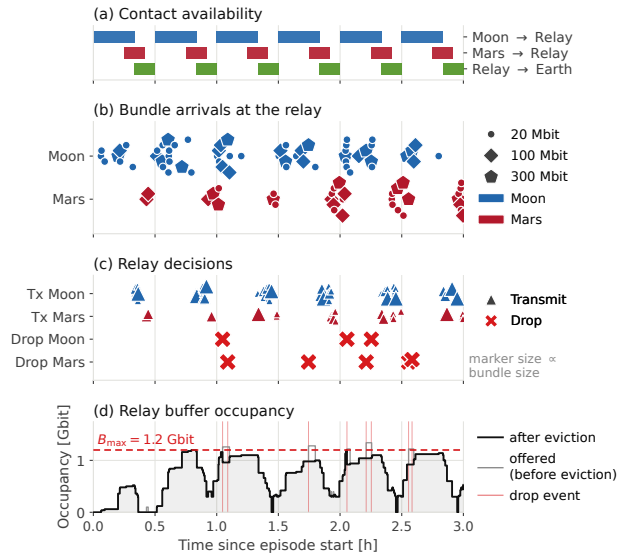
Fig. 3. Relay operation under the PPO policy.
