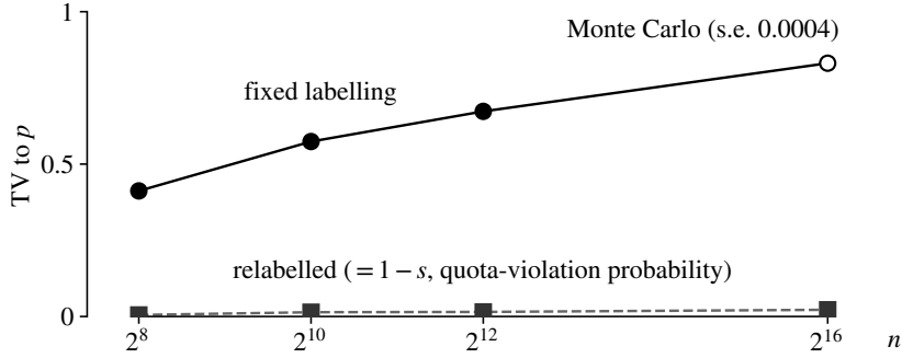
Figure 5: The mechanism at finite n ( \varepsilon = \ln 2 ; finite computation, Table 5): total variation to p of the K = \lceil 2 \ln(2/\delta) \rceil = 3 ladder of Theorem 2(b)’s proof ( \delta = \frac{1}{2} ; the Hoeffding–Ville choice, where the stated bound takes K_\delta = 2 ; Table 5 lists its blocks) under the fixed labelling (circles) and under its relabelling (squares; = 1 - s , the quota-violation probability). Filled: computed; open: a seeded Monte Carlo estimate (standard error 0.0004). The least lengths of the same table are plotted in Figure 2.
