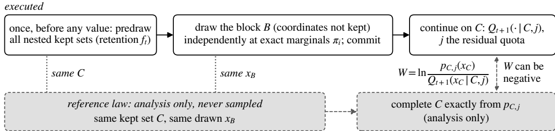
Figure 4: One level of the bounded-weight sampler (top, executed) and of the reference law (bottom, analysis only). Both share the kept set C and the block values x_B ; W compares the two completions of C ( W = 0 if j is infeasible).
