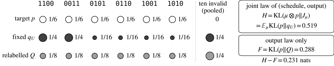
Figure 1: The four-bit example. Columns: the six valid strings (two ones) and, pooled, the ten invalid ones; disc areas are unconditional probabilities, and nothing is renormalized. The example implies no rate.
