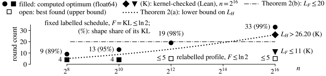
Figure 2: Balanced slice, \varepsilon = \ln 2 : round counts of one fixed labelled schedule (circles) and one relabelled profile (squares). Each has one length per run, so circles and squares bound L_H and L_F from above; open squares (best-found witnesses) and the kernel-checked L_F \leq 11 at n = 2^{16} are upper bounds not shown optimal. No rate is fitted.
