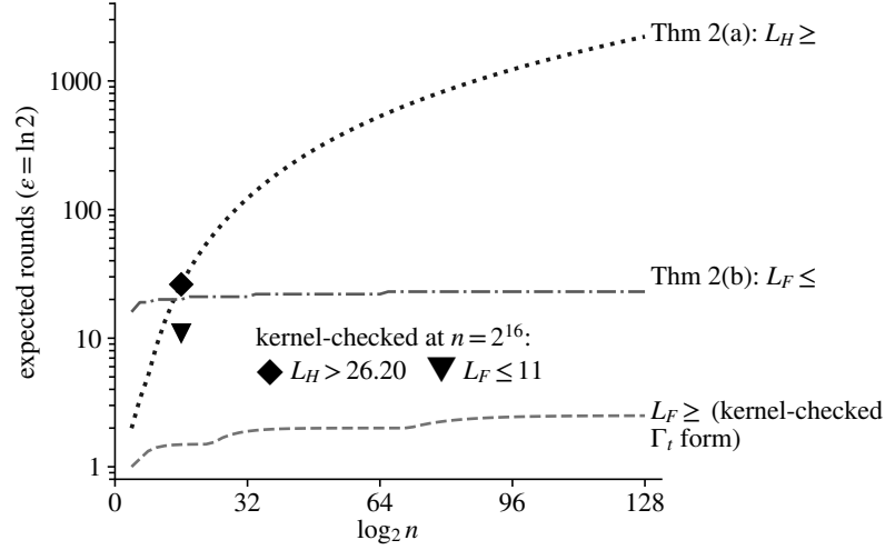
Figure 6: Proved bounds as functions of n at \varepsilon = \ln 2 and the kernel-checked finite certificates at n = 2^{16} . Curves are formula evaluations, not measurements.
