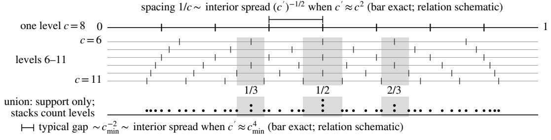
Figure 3: Exact grid points and bars; relations schematic. Top: level c = 8 ; middle: levels 6–11; bottom: their union, with gaps of order c_{\min}^{-2} away from small denominators (shaded: larger gaps near 1/3, 1/2, 2/3 ; not the converse's set S^* ). Dots: support, not probability.
