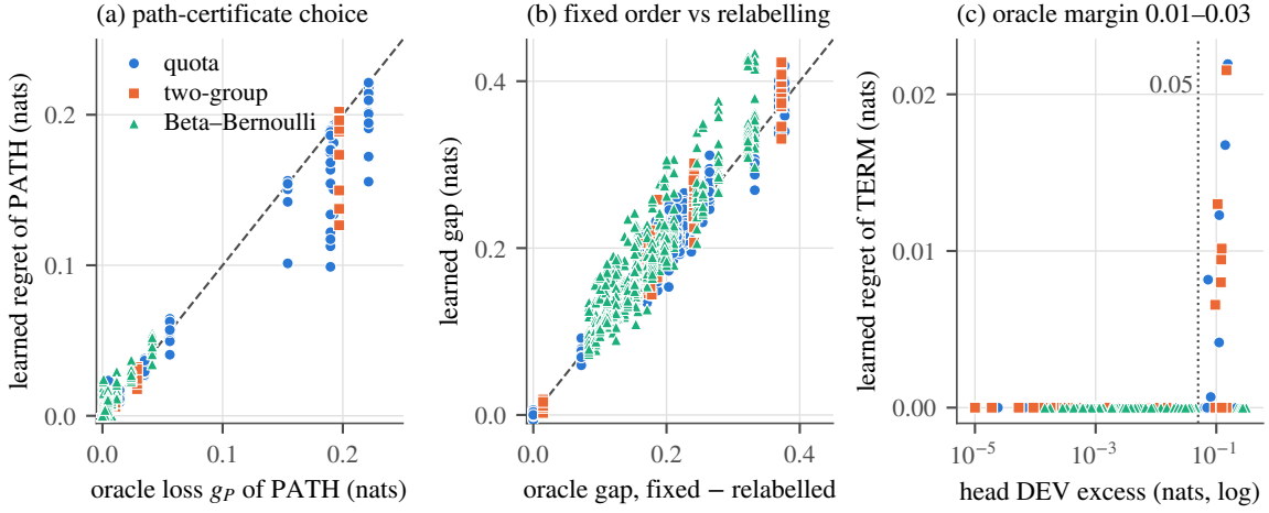
Figure 7: Controlled test with learned conditionals (144 fresh trajectories, 48 independent clusters, six held-out regimes and fresh seeds on two discovery targets; output KL of the complete output law, computed in float64 by dynamic programming over revealed sets (no sampling), n \leq 16 ; predictions frozen before evaluation). (a) Learned regret of the path-optimal profile PATH versus its oracle loss g_P (identity dashed). (b) Learned versus oracle gap between a fixed labelled order and its relabelling. (c) Learned regret of the exact-oracle terminal-optimal profile TERM against the head’s development-loss excess (“DEV excess”), for cells with oracle margin 0.01–0.03 and the EARLY, ES and END checkpoints of each run (descriptive, not a frozen pass/fail item; dotted line at 0.05, the top boundary of the freeze’s descriptive head-error bands \leq 0.02 , 0.02-0.05 and > 0.05 ; DEV excess, which can be negative, is drawn clipped below at 10^{-5} ). Controlled prediction only.
