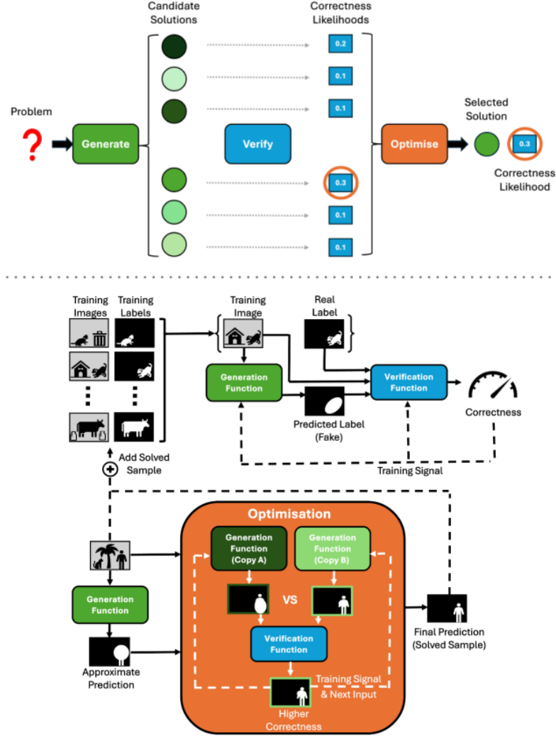
Fig. 2: Overview of GenVerOpt (top: conceptual summary; bottom: details of one implementation of GenVerOpt for the dummy task of human segmentation on natural images).
