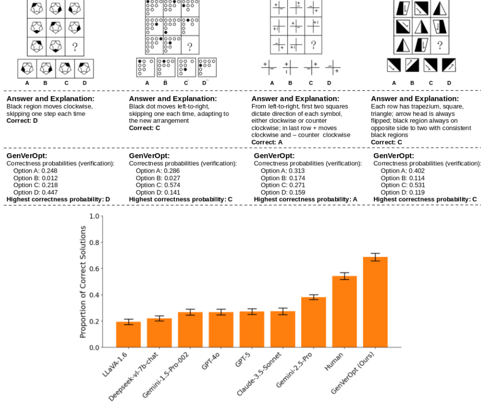
Fig. 3: IQ test puzzles solved by GenVerOpt and a comparison with humans and commonly used AI models. Open-source models LLaVA and Deepseek were fine-tuned using low-rank adaptation on the dataset before inference and closed-source models were primed using four-shot prompting with examples randomly selected from the datasets and performance averaged across 8 runs. Task-specific models were trained from scratch on the same data as GenVerOpt.
