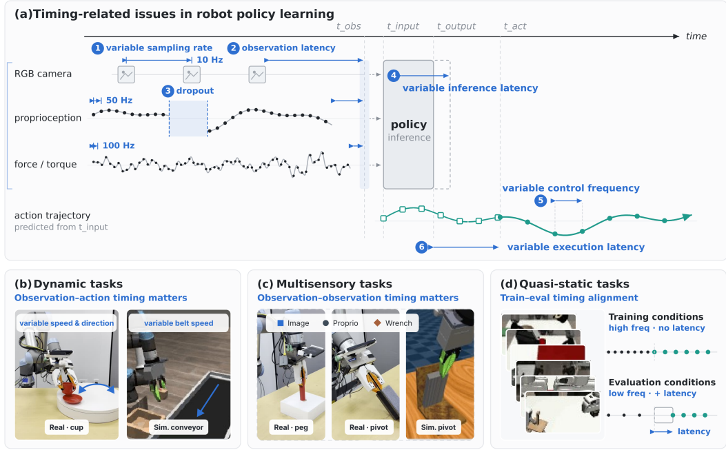
Figure 1: Timing-related issues in robot policy learning. (a) Real robot systems exhibit multiple sources of temporal variation, including variable sensor sampling rate, observation latency and dropout, inference latency, control frequency, and execution latency. These timing effects matter differently across tasks. (b) In dynamic tasks, the key temporal relationship is between when an observation is captured and when an action takes effect . (c) In multisensory tasks, the key temporal relationship is between when different observations are captured . (d) Even in quasi-static tasks, differences between data-collection and deployment timing can create temporal mismatch. Standard fixed-rate policy representations obscure these distinctions by treating sequence position as a proxy for time.
