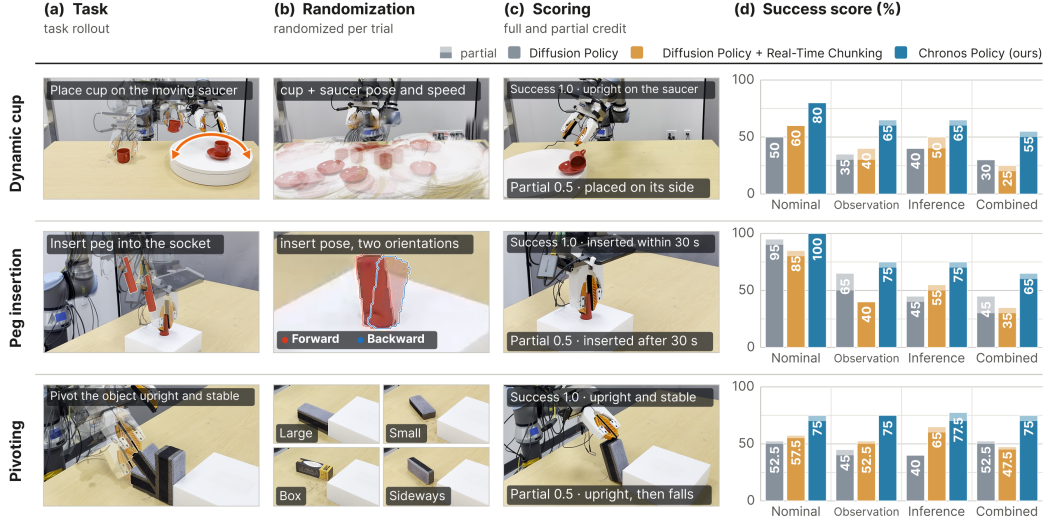
Figure 5: Real-world evaluation under timing variation. We compare Diffusion Policy, Diffusion Policy with RTC, and Chronos Policy on Dynamic Cup, Peg Insertion, and Pivoting under nominal, observation, inference, and combined timing conditions. Lighter bar segments indicate partial success.
