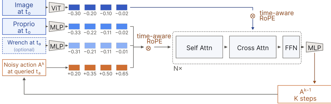
Figure 6: Architecture of Chronos Policy. Proprioceptive, optional force/torque, and noisy action tokens interact through self-attention and attend to image features through cross-attention. Time-aware RoPE encodes observation capture times and queried action times in attention. The transformer iteratively denoises the action chunk.
