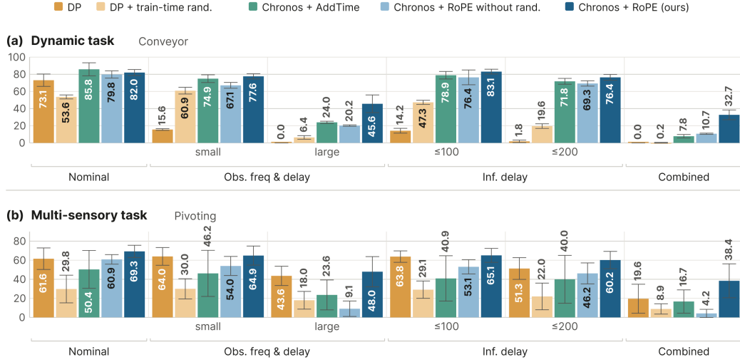
Figure 3: Simulation ablation of Chronos Policy design. We compare temporal randomization, additive time encoding, and time-aware RoPE to identify an effective recipe for time awareness. Temporal randomization is most effective when paired with explicit timestamps, while time-aware RoPE provides the strongest robustness across Conveyor and Pivoting.
