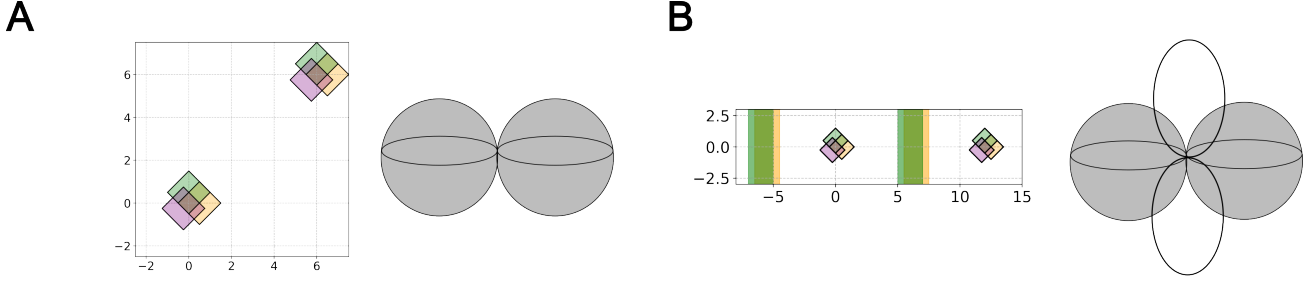
Figure 2. A. An example of the wedge of two spheres that arises through the Helly-arrangement living within [-1.5, 1.5]^2 and [4.5, 7.5]^2 . B. An example of the wedge of two spheres and two circles along with an arrangement that defines it. The four sets are defined strictly within [-7.5, -4.5] \times (-\infty, \infty) , [-1.5, 1.5]^2 , [4.5, 7.5] \times (-\infty, \infty) and [10.5, 13.5] \times [-1.5, 1.5] respectively. Notice that the configurations generating the circles span the whole y direction, thus it is important to always choose the shifts on the x axis, otherwise two circles might end up intersecting in more places than the origin.
