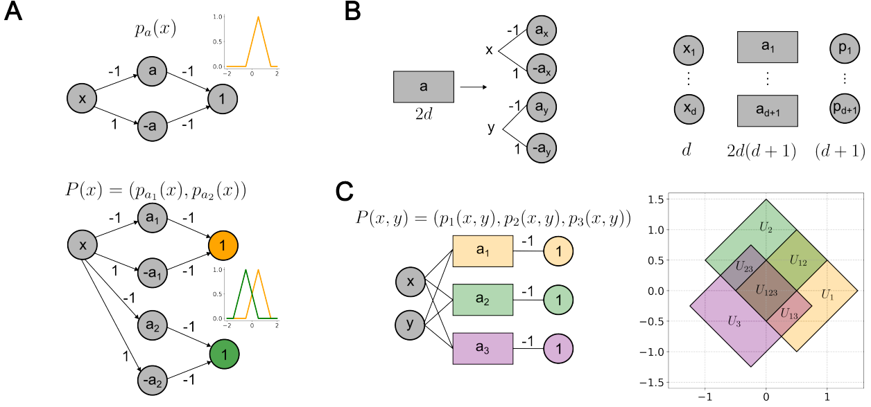
Figure 1. An illustration of how hat functions can be expressed by a neural network.
