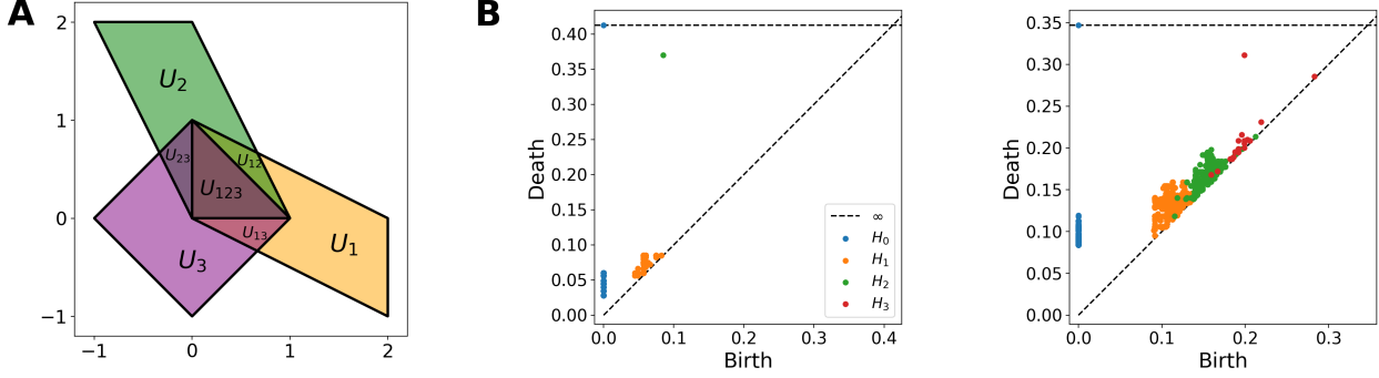
Figure 3. A. The active regions of the functions defining the proposed construction. B. The birth-death diagrams for the bottom four homology groups of S^2 (left) and S^3 (right).
