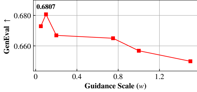
Figure 16: PAG. Six-point weight sweep.
