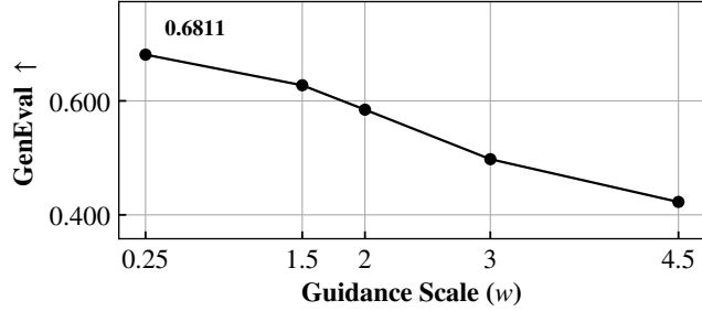
Figure 18: S 2 . Five-point weight sweep.
