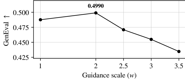
Figure 21: S 2 . Five-point weight sweep.
