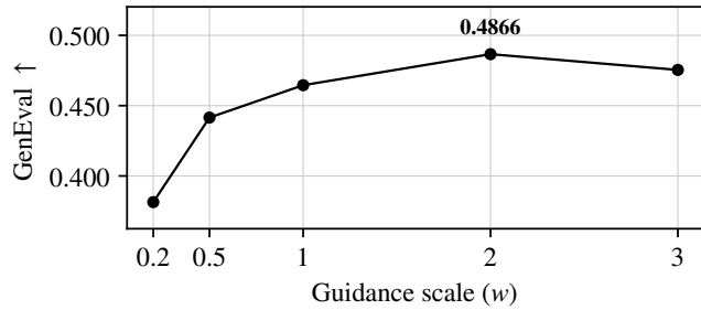
Figure 15: S^2 . Five-point weight sweep.
