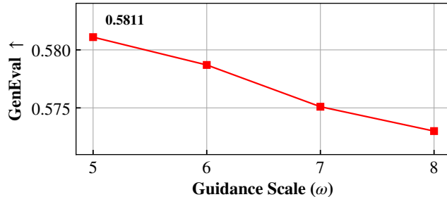
Figure 9: SD3M without CFG / GenEval guidance-scale sweep.
