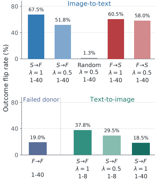
Figure 4: Message transplantation and controls. S/F denote successful/failed trajectories; arrows point from donor to recipient. Labels show donor mixing weight \lambda and transplant steps. Full results: Table 21.
