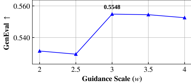
Figure 20: SEG. Five-point weight sweep.
