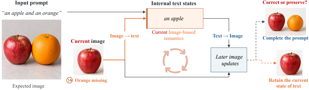
Figure 2: Image-to-text feedback. The current image writes into internal text states through B_{i \rightarrow t} , which later blocks read to update the image. If the image misses an object, does this feedback help recover it or preserve the incomplete scene? Text labels and AI-generated fruit images illustrate schematic states and possible outcomes; the input prompt stays fixed.
