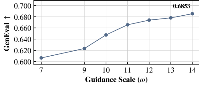
Figure 10: FLUX without CFG / GenEval guidance-scale sweep.
