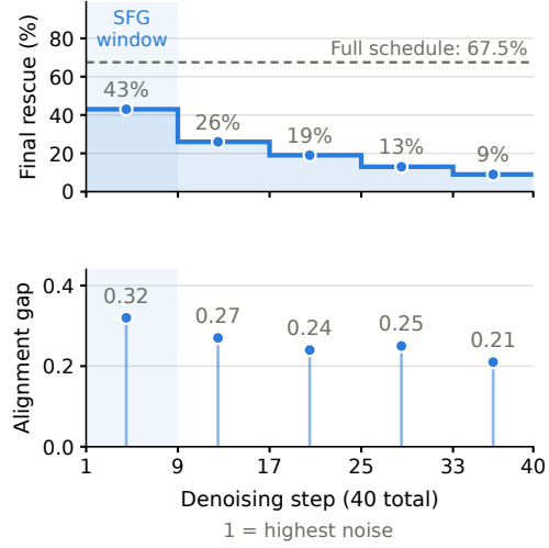
Figure 5: Timing and alignment on 400 pairs across SD3.5M and FLUX. Top: rescue by transplant window; steps 1–8 of 40 recover about two-thirds of the full-schedule effect. Bottom: cosine gap over random, averaged within pairs, then within models, with equal model weights. Shading marks steps 1–8.
