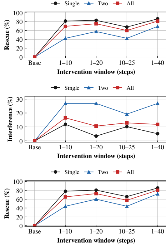
Figure 22: Top to bottom: failure rescue, success disruption, and warned-failure rescue.
