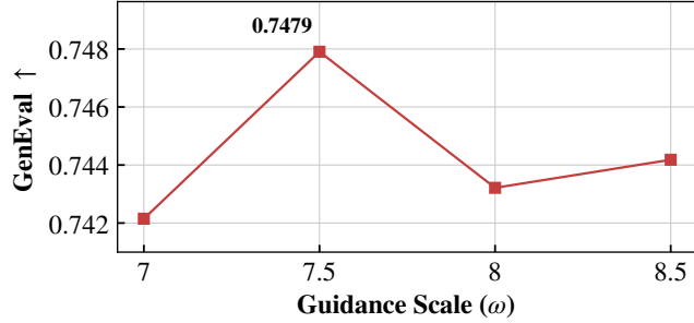
Figure 11: FLUX with CFG / GenEval guidance-scale sweep.
