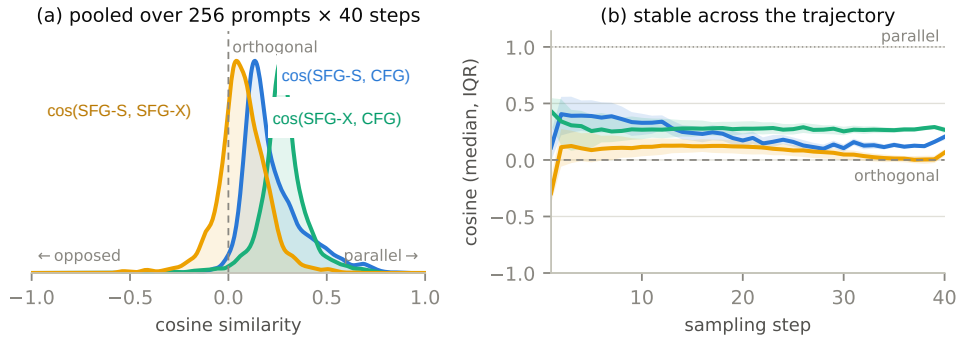
Figure 8: Complementary directions. SFG-X and SFG-S corrections have low cosine similarity with CFG and with each other, both over prompts and through sampling.
