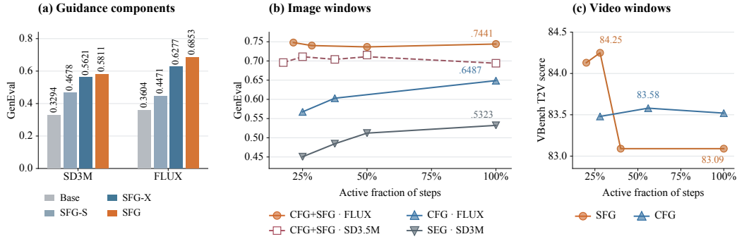
Figure 7: Guidance components and guidance windows. (a) GenEval at the Table 1 operating points. (b) Both FLUX curves use 28 steps; SD3.5M CFG+SFG and SD3M SEG use 40. FLUX CFG returns to scale 1 outside its guidance window. (c) HunyuanVideo T2V scores with 25 total sampling steps. SFG is active for the first 5, 7, 10, or 25 steps; CFG is active for the first 7, 14, or 25 steps. Guidance is disabled after the selected prefix.
