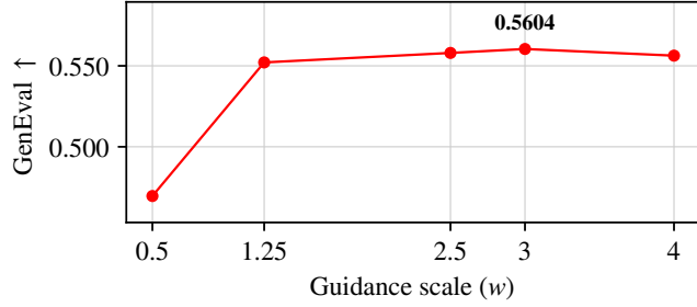
Figure 13: PAG . Five-point weight sweep.
