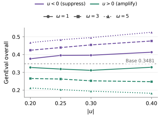
Figure 6: Validation of the SFG-X guidance direction. GenEval on SD3.5M ( \text{cfg} = 1 ), comparing SFG-X ( u < 0 ) with the opposite-sign branch ( u > 0 ) at matched |u| and \omega . Suppression/amplification labels denote the net guidance effect. Base marks the unguided score.
