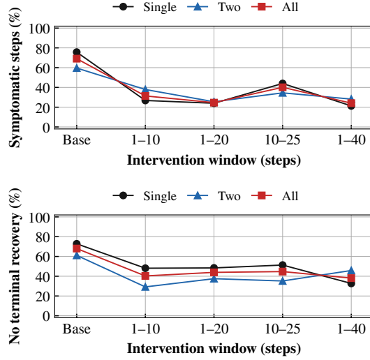
Figure 23: Top to bottom: symptom persistence and no terminal recovery.
