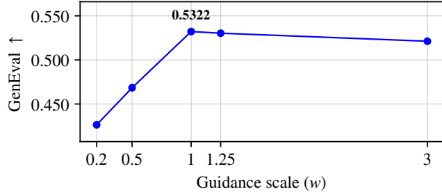
Figure 14: SEG . Five-point weight sweep.
