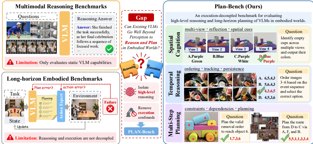
Figure 1: Overview of Plan-Bench. The left illustrates the limitations of existing benchmarks, which either evaluate static VLM capabilities or couple high-level reasoning with low-level execution. The right presents the composition of Plan-Bench, which evaluates execution-decoupled high-level reasoning and planning across Spatial Cognition, Temporal Reasoning, and Multi-Step Planning.
