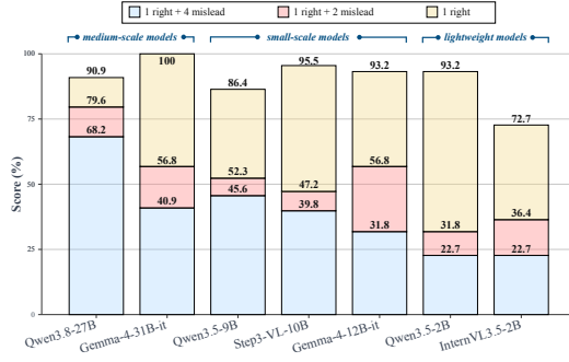
Figure 5: Robustness to Increasing Misleading Views across Model Scales.
