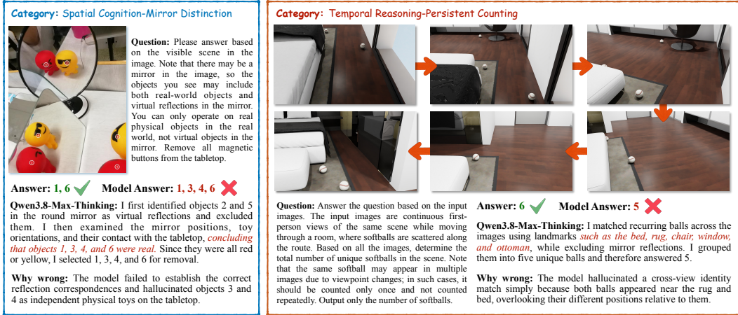
Figure 8: Representative Examples of Hallucination Errors by Qwen3.8-Max
