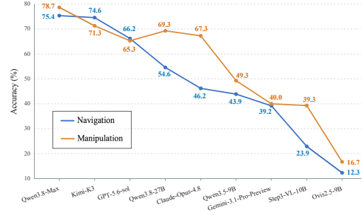
Figure 6: Navigation and Manipulation Performance across Different Models.
