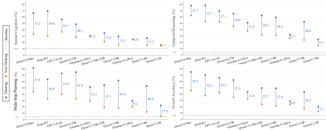
Figure 7: Comparison between Thinking and Non-Thinking modes on Plan-Bench across Spatial Cognition, Temporal Reasoning, Multi-Step Planning, and overall accuracy. Blue and orange markers denote Thinking and Non-Thinking results, while the annotated values indicate their gaps.
