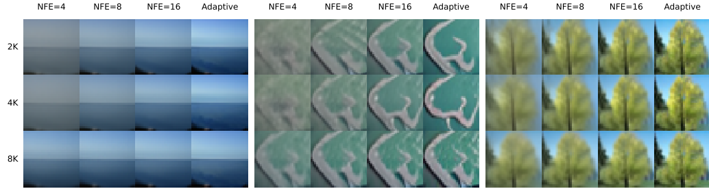
Figure 3: Generated images from initial noise. Rows correspond to minibatch sizes of 2K, 4K, and 8K, while columns compare Euler sampling at NFE 4, 8, and 16 with adaptive Dopri5. Smaller coupling minibatches tend to produce darker, less vivid images, whereas larger minibatches yield brighter samples with more vibrant colors, particularly at low NFEs.
