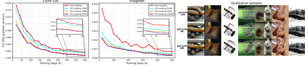
Figure 2: Full SGD gradient variance and qualitative samples. Variance during training on CIFAR-100 ( left ) and ImageNet ( middle ) under different minibatch size, with insets highlighting late-stage behavior. Samples from OT-CFM and EOT-CFM from 128 to 10K, generated at NFE 100. ( right ).
