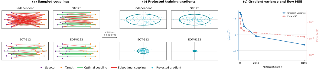
Figure 4: Results on a synthetic ring task over independent random coupling, OT-CFM using the minibatch size of 128, and EOT-CFM with contexts up to 8192. From left to right, each panel corresponds the flow couplings, the projected training gradients, and the final gradient variance and generation quality under different context size. All the training setup follows from Figure 1.
