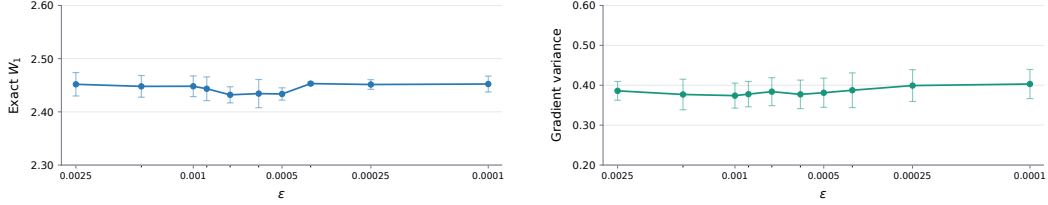
Figure 5: Ablation over \epsilon on the PBMC dataset with an 8K entropic OT context, with the exact W_1 error of generated samples (left) and training gradient variance (right) shown. We sweep \epsilon from \{0.0025, 0.0015, 0.001, 0.0009, 0.00075, 0.0006, 0.0005, 0.0004, 0.00025, 0.0001\} .
