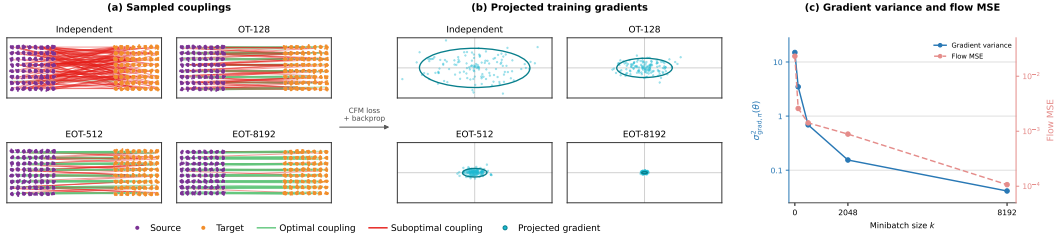
Figure 1: Results on a synthetic multimodal task over independent random coupling, OT-CFM using the minibatch size of 128, and EOT-CFM with contexts up to 8192. (a) Source-target pairings, with green and red lines indicating optimal and suboptimal couplings, respectively. Larger minibatches produce more optimal assignments for subsequent flow training. (b) Stochastic gradients evaluated at a trained flow model with regression batch size 128 and projected onto common two-dimensional axes; ellipses summarize their spread. (c) Full gradient variance (left axis) and final flow-generation MSE (right axis) averaged over three training seeds, scaling along the OT minibatch size, where k = 0 denotes independent coupling. Scaling the minibatch size consistently reduces both gradient variance and MSE error, yielding more stable training and better flow generation.
