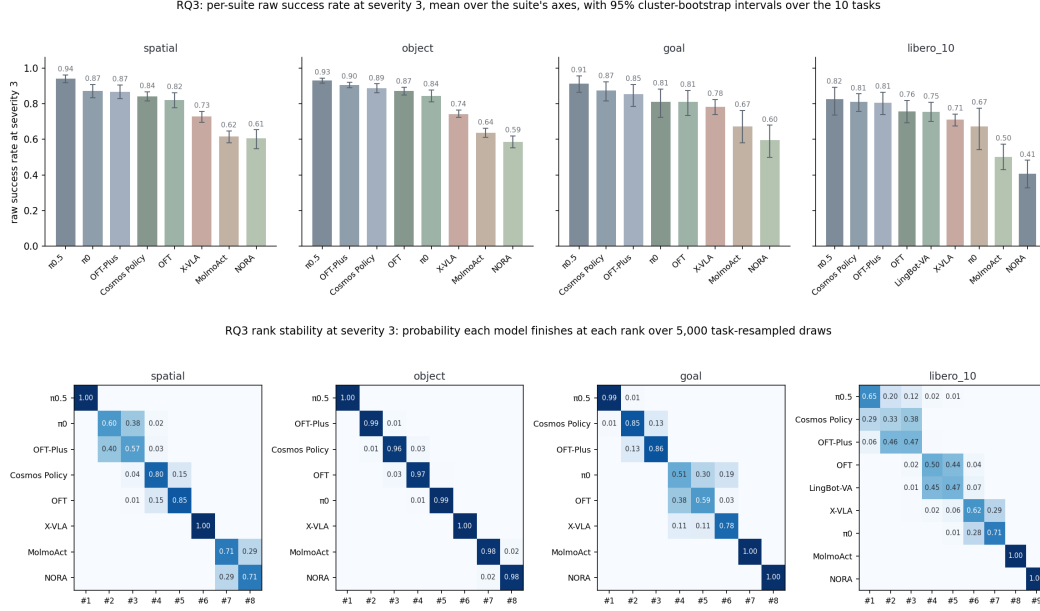
Figure 7: Per-suite success with intervals (top) and rank stability (bottom) at severity 3. Top: raw success rate per suite, mean over the suite’s axes, with 95 percent intervals from a cluster bootstrap over the 10 tasks, the same task resamples for every model. Bottom: as Fig. 4.
