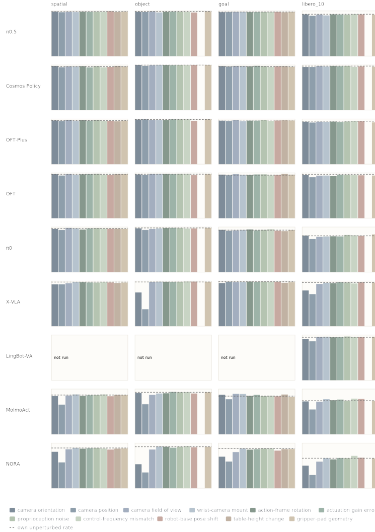
Figure 11: Full results grid, severity 1. Rows are models, columns the four suites, 11 bars per panel in a fixed axis order. The dashed line is that model’s own unperturbed rate on that suite, so a bar reaching the line means the perturbation cost nothing. The numbers are in Tables 8 to 12. This figure plots Table 8; Figs. 12 to 15 plot Tables 9 to 12 for severities 2 to 5.
