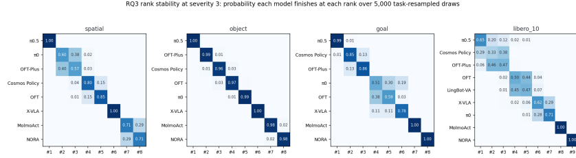
Figure 4: Rank stability at severity 3 . Probability that each model lands at each rank over 5,000 task-resampled draws, paired across models.
