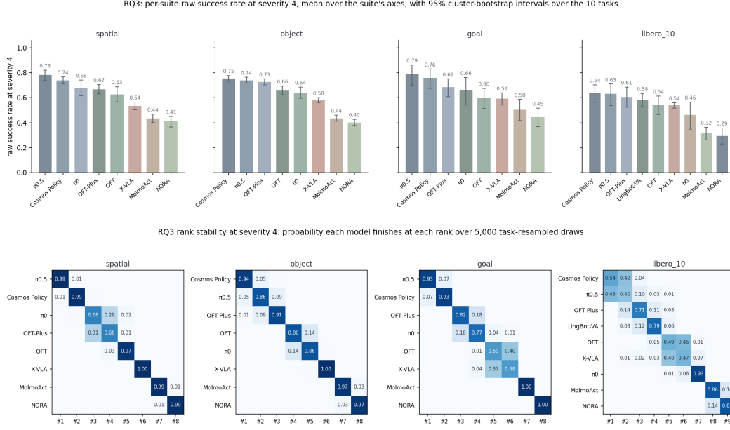
Figure 8: Per-suite success with intervals (top) and rank stability (bottom) at severity 4 , as in Fig. 7. Cosmos Policy takes the object and LIBERO-10 suites.
