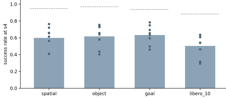
RQ4: raw success rate on the 10 shared axes at severity level 4; dots = the 8 models; dashed = suite pooled nominal
