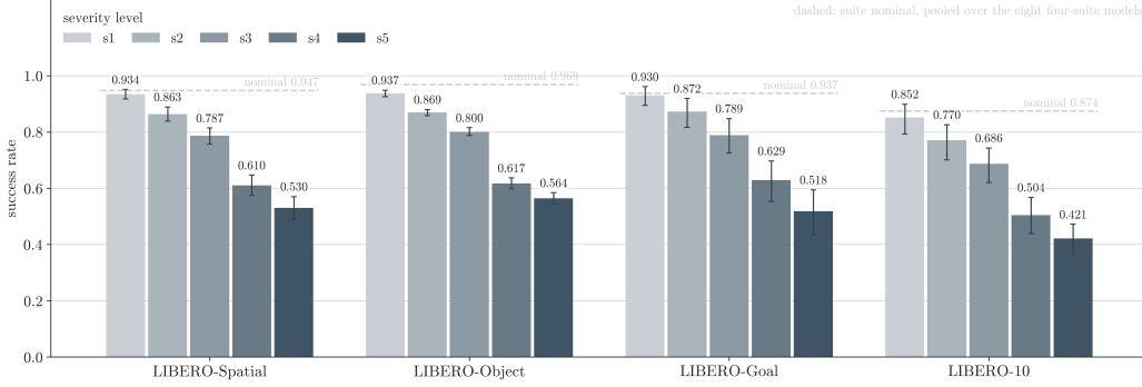
Figure 3: Success rate by suite and severity level , level 1 light to level 5 dark, pooled over the eight four-suite models; the dashed line is each suite’s pooled nominal.
