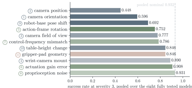
Figure 2: Success rate by axis at severity 3 , pooled over the eight fully tested models (excluding LingBot-VA); dashed line, pooled nominal; observable axes blue, latent axes green, the weakly observable axis orange, with the axis numbers of Fig. 1.
