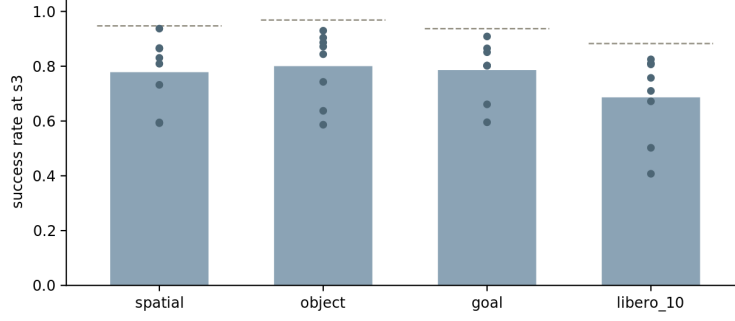
RQ4: raw success rate on the 10 shared axes at severity level 3; dots = the 8 models; dashed = suite pooled nominal
