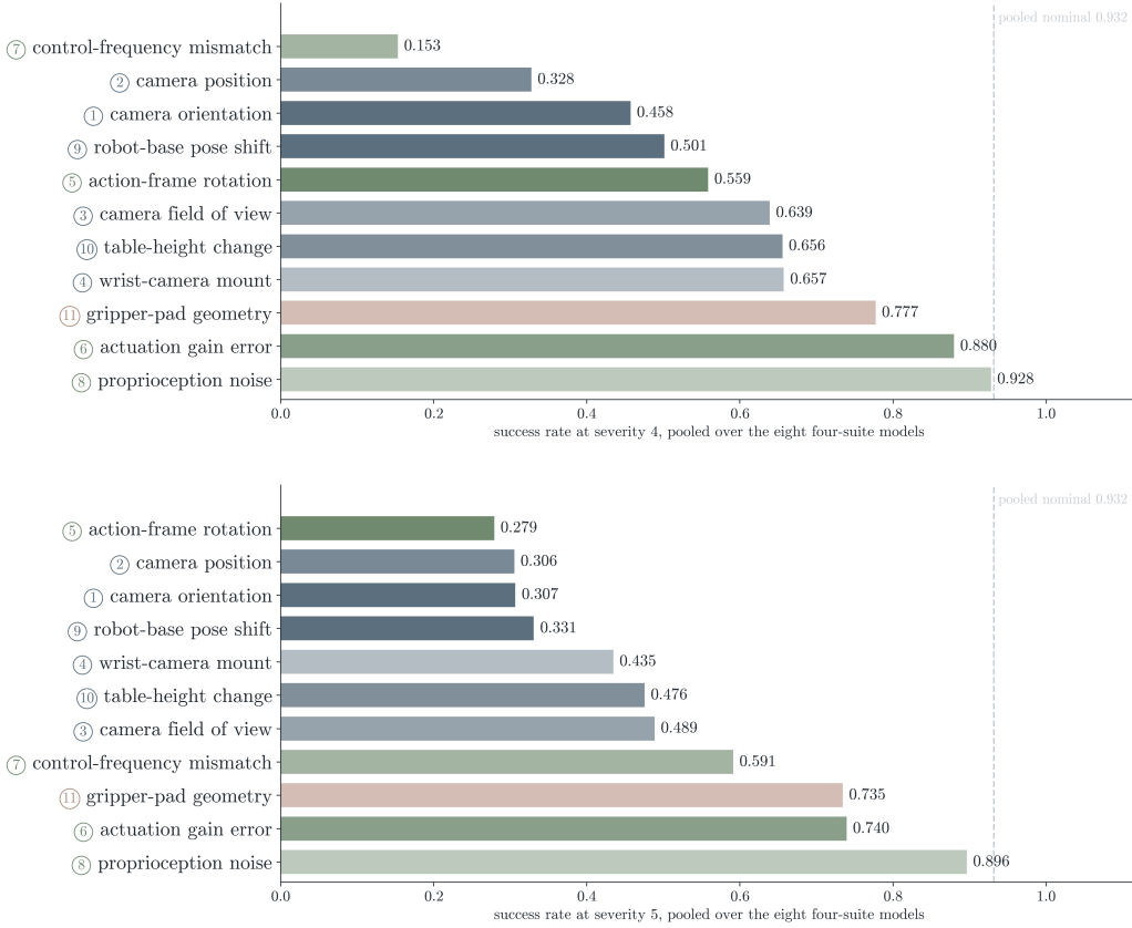
Figure 6: Success rate by axis at severities 4 (top) and 5 (bottom), pooled over the eight four-suite models; dashed line is the pooled nominal; colors as in Fig. 2.
