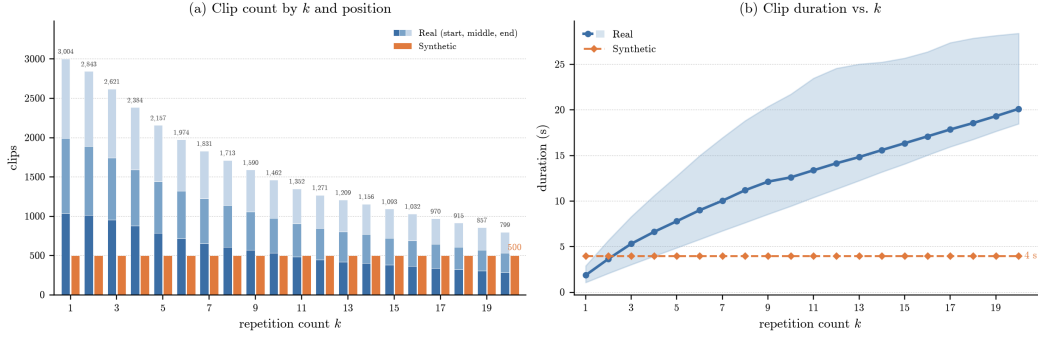
Figure 2: RepProbe statistics. (a) Clips per repetition count k . RepProbe-Real (blue, stacked by clip position: start, middle, end) is skewed toward small counts because fewer source videos contain many repetitions; RepProbe-Synthetic (orange) is balanced at 500 clips per count. (b) Clip duration versus k . Real clip duration grows with k (line: median; shaded band: spread across clips), whereas every synthetic clip lasts 4 s regardless of k .
