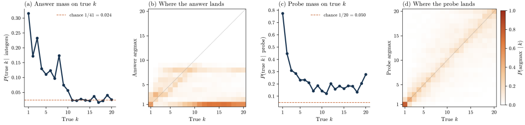
Figure 4: The count is recoverable by a probe but not by the model’s answer (Cosmos-Reason2, RepProbe-Real). (a) The answer’s probability on the true k falls to chance by k \approx 11 ; (b) its argmax collapses onto a few small numbers. (c) The probe keeps far more mass on the true k ; (d) its argmax tracks k across the full range.
