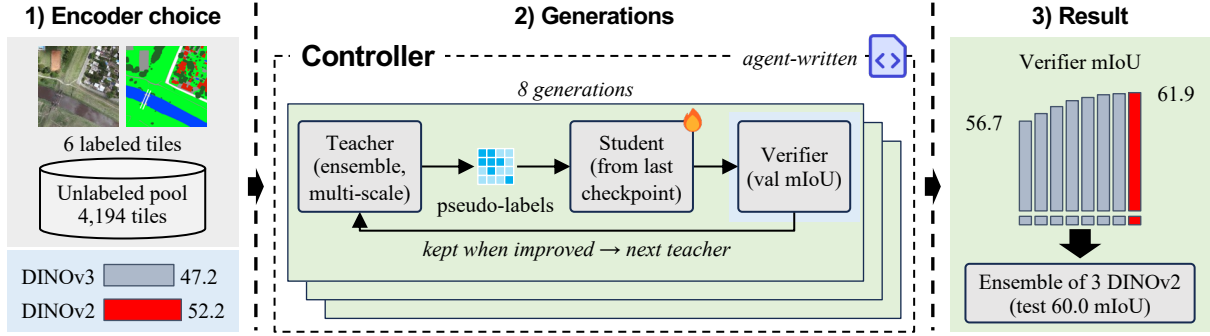
Figure 2: Lineage of the six-label OpenEarthMap run. The agent compares encoders on the verifier, pseudo-labels the unlabeled pool with its best model, and runs eight generations in which the best verified pipeline teaches a student that continues from the previous generation. In the later generations, controller scripts written by the agent select the teacher from the verifier log and start the next generation. The final three-network ensemble scores 60.0 mIoU on the hidden test set.
