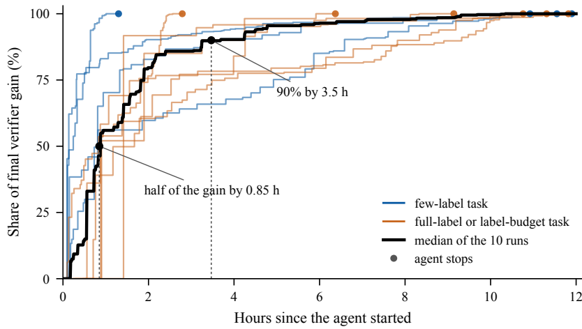
Figure 3: Progress within a run. Share of the final verifier gain reached over time in the 10 runs of GPT-6-Astra for which trajectories are available, where the gain is measured from the first to the best verifier score of a run. A dot marks the time at which the agent ends the run, and the black line is the median over runs.
