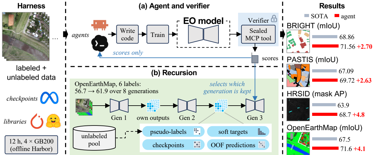
Figure 1: RSI4EO casts any EO task as a harness and a verifier. The harness defines what the agent may use and the verifier defines what counts as success. (a) A general-purpose coding agent writes and trains the EO model and receives only the scores of the sealed verifier. (b) Each generation of the model is built from the outputs of the previous one, and the verifier decides which generation is kept. The resulting models surpass the state of the art on four benchmarks (Table 2).
