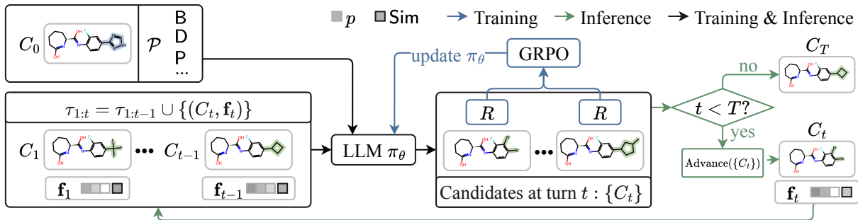
Figure 1: Overall figure of Multi-turn Feedback Guided (MFG) MOMO.
