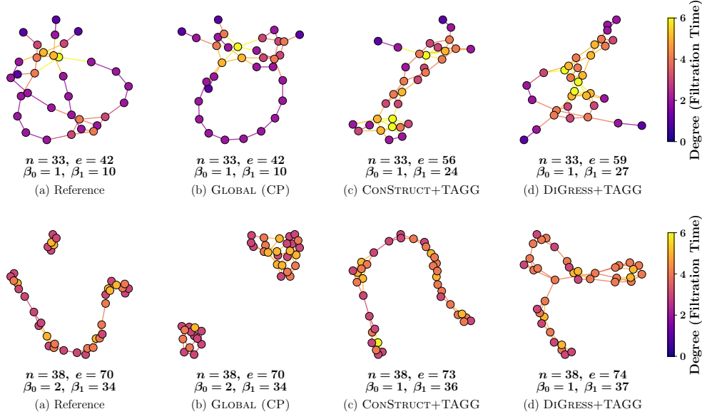
Figure 5: Two qualitative examples on ENZYMES test graphs (enzymes_87, top; enzymes_93, bottom). Left to right: reference, GLOBAL (CP), CONSTRUCT+TAGG, DIGRESS+TAGG. Node colour encodes degree. CP matches (n, |E|, \beta_0, \beta_1) exactly on both graphs; neural variants drift in edge count and cycle count.
