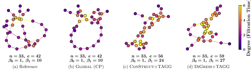
Figure 3: Qualitative example on an ENZYMES test graph. Node colour encodes degree. CP matches (n, |E|, \beta_0, \beta_1) exactly, while neural variants add excess cycles. More in Appendix H.6.
