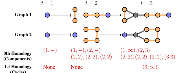
Figure 1: Two non-isomorphic graphs with identical degree-based persistence. Vertex color encodes degree; edges inherit the color of their max-degree endpoint.
