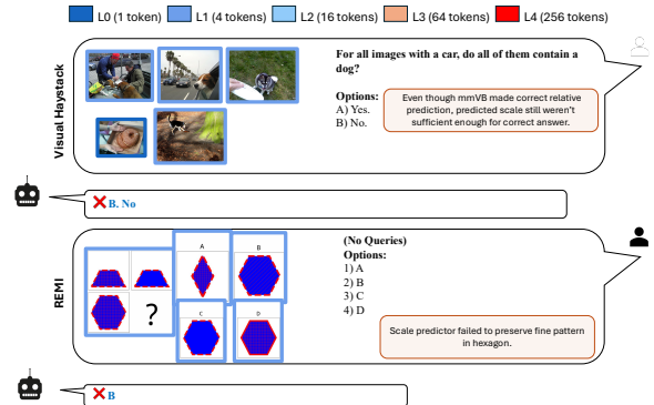
Figure 5: Limitations. Scale predictor may underestimate tokens needed to answer questions. May also fail when there’s no text query.
