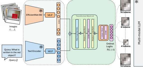
Figure 2: mmVB architecture. Frozen EfficientNet-B0 encodes N images, while frozen LLM embeddings encode the query through mean pooling and a 64-dimensional bottleneck. A two-layer, four-head Transformer processes all N+1 tokens, after which a shared MLP maps each image token to four ordinal logits.
