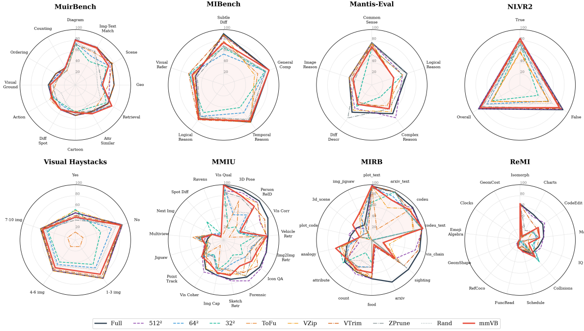
Figure 6: Per-task accuracy across eight benchmarks. Each subplot represents one benchmark. Solid lines show Full-res and mmVB; dashed lines show uniform resolutions; dash-dot lines show post-encoding baselines; and dotted lines show the distribution-matched random baseline. mmVB closely tracks Full-res while using 9.2\times fewer visual tokens (geometric mean across benchmarks).
