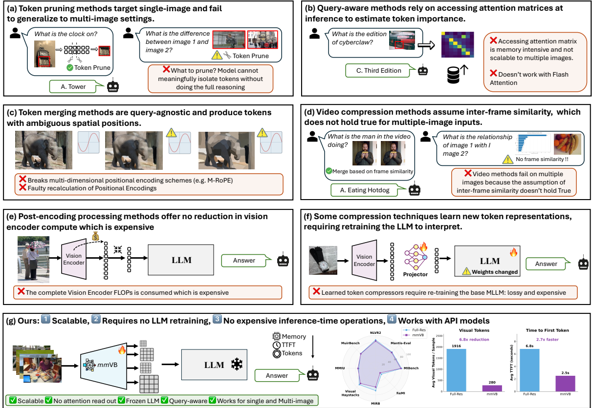
Figure 1: Introduction and Motivation. Existing multi-image methods scale poorly: dense attention breaks FlashAttention and excludes API-only models, token merging disrupts positional encodings and cross-image reasoning, and video-style compression assumes frame similarity. Our pre-encoding predictor instead assigns query-conditioned token budgets using only pixels, enabling compatibility with any MLLM, including closed models.
