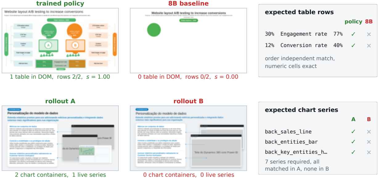
Figure D2 Table/Chart. Outlines mark the tables and charts found in the DOM. Top: the baseline emits no table. Bottom: two rollouts on a chart prompt, with and without live ECharts instances.
