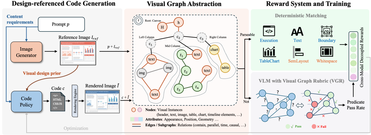
Figure 2 Overview of AesCode. Prompt requirements and reference design cues yield graph-based supervision. Conditioned on p and I_{\text{ref}} , the policy generates HTML/CSS code c , rendered as \hat{I} .
