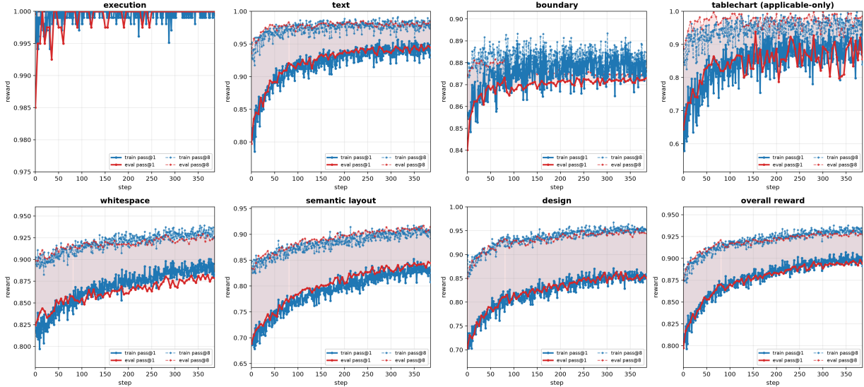
Figure C1 Per-channel training rewards under GDPO. Solid: single rollout; dashed: mean over eight rollouts; blue: training set; red: held-out set.
