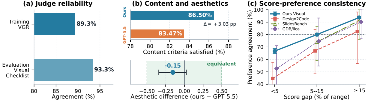
Figure 4 Human evaluation. (a) Agreement with training VGR and evaluation-checklist judgments. (b) Content satisfaction and aesthetic equivalence between AesCode-32B and GPT-5.5. (c) Agreement between metric rankings and human preference by normalized score gap.
