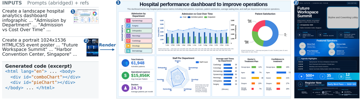
Figure 1 Information-rich infographics generated as code. Prompts specify content, while image-generator references offer visual design guidance. The examples show a landscape dashboard and portrait poster rendered from generated HTML/CSS.
