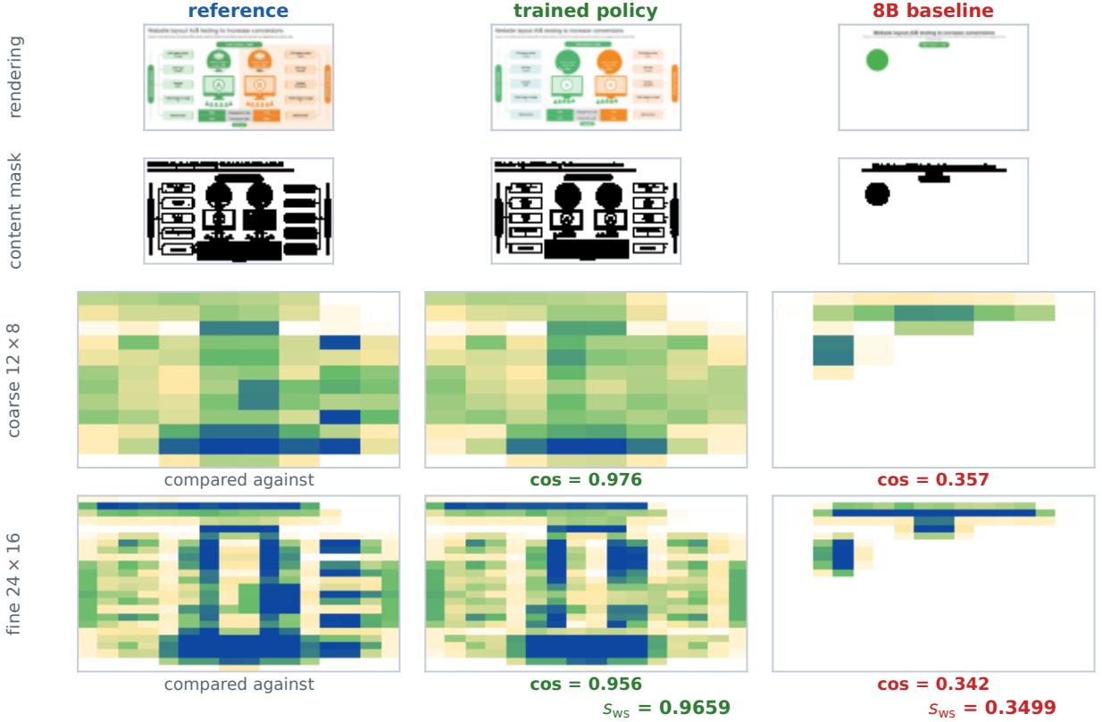
Figure D4 Whitespace. Rendering, content mask, and coarse and fine occupancy grids; s_{ws} averages the two grid cosines with the reference.
