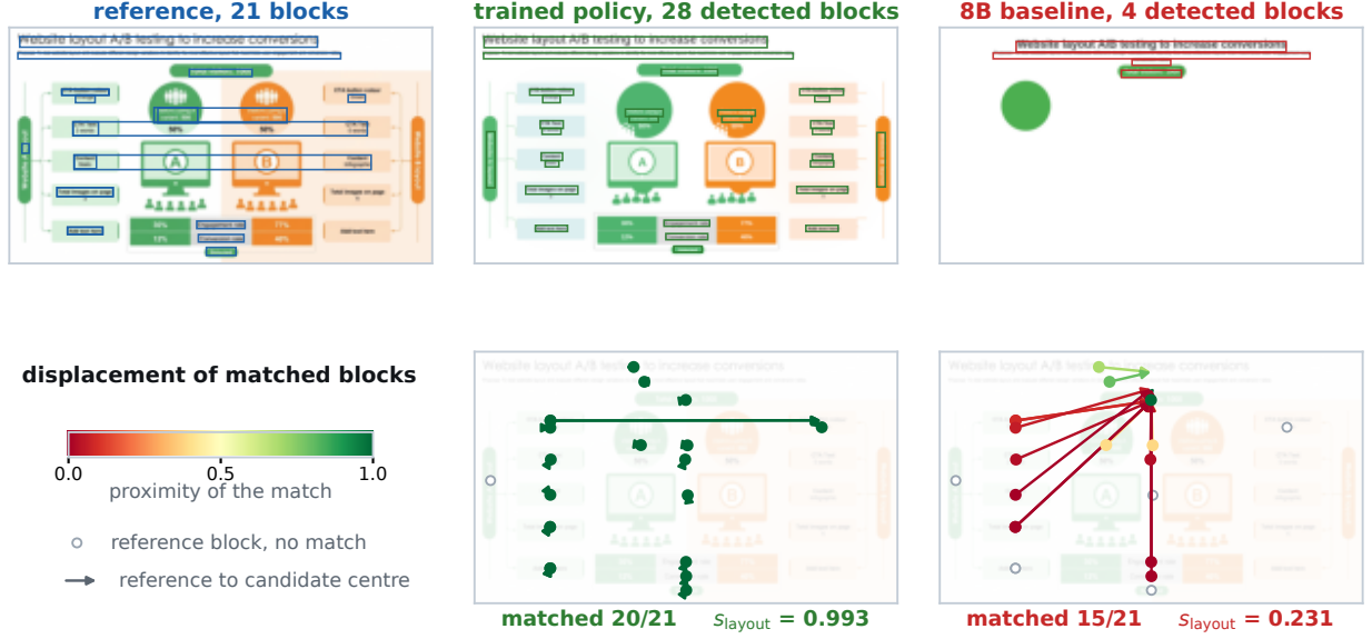
Figure D3 SemanticLayout. Top: OCR text blocks. Bottom: arrows from each reference block to its matched candidate block, coloured by proximity; hollow circles are unmatched reference blocks.
