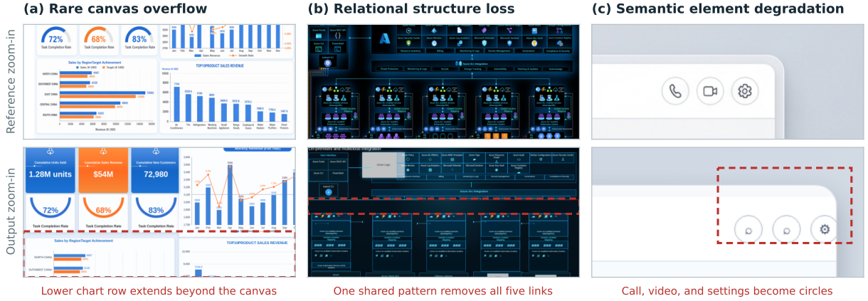
Figure 5 Residual failures of AesCode-32B. Reference and output zoom-ins show (a) canvas overflow, (b) lost relational structure, and (c) semantic element degradation. Dashed boxes mark affected regions; frequencies and additional cases appear in Section F.
