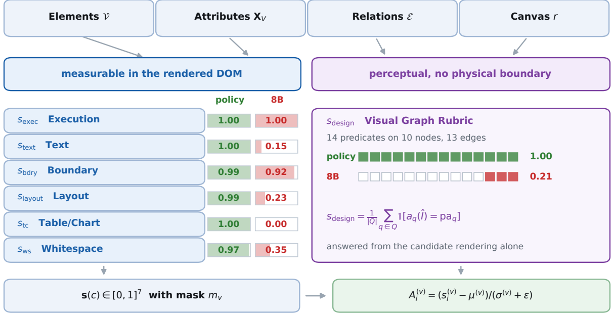
Figure D1 Reward channels. Six deterministic verifiers read the rendered DOM and screenshot. Execution : render success, decayed by uncaught JavaScript errors. Text : required strings found, weighted by overlap and in-canvas visibility. Boundary : in-canvas fraction of overflowing elements and aspect-ratio match. Layout : proximity of text blocks matched to the reference. Table/Chart : parsed table rows and ECharts series against the required data. Whitespace : cosine similarity of occupancy grids with the reference. VGR : pass rate of sample-specific yes/no predicates answered from the candidate render. Each channel is masked by applicability and normalized separately by GDPO. Values are from two rollouts on one prompt.
