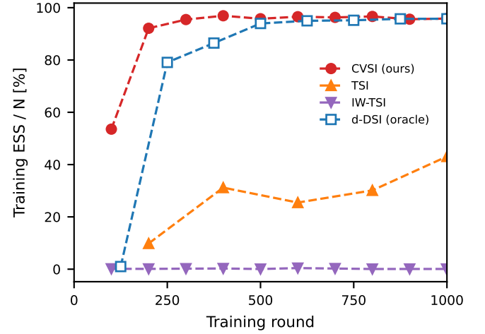
FIG. 5. Training dynamics of the ESS for N = 5000 samples.
