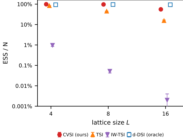
FIG. 2. ESS comparison of our data-free CVSI training (red circle), TSI (orange triangle) and IW-TSI (purple inverted triangle), as well as the oracle data-driven DSI (blue square), at criticality. Error bars show 1\sigma confidence intervals.
