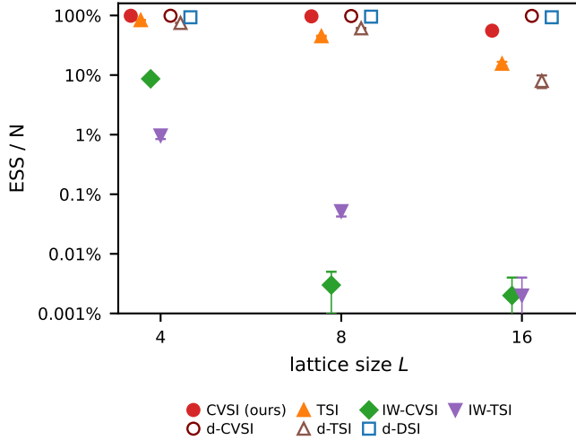
FIG. 6. ESS comparison of data-free and data-driven training.
