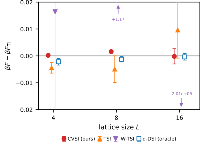
FIG. 3. Free-energy estimation error \beta F - \beta F_{\text{TI}} at criticality.
