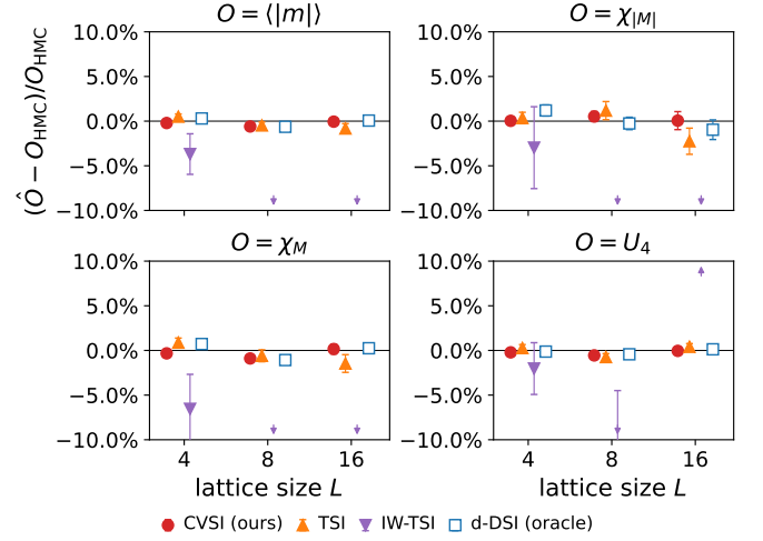
FIG. 4. Estimation errors for the mean absolute magnetization \langle|m|\rangle , the susceptibility of the absolute magnetization \chi_{|M|} , the magnetic susceptibility \chi_M , and the fourth-order Binder cumulant U_4 .
