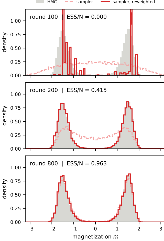
FIG. 8. Magnetization at L = 8 , broken phase, over the self-learning loop. Raw samples (light red) and reweighted (red) approach the HMC reference (grey).
