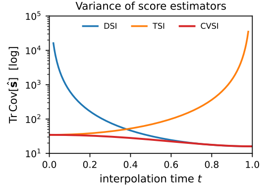
FIG. 1. Score estimator variance vs. diffusion time t ( L = 4 , symmetric). While DSI and TSI diverge at either end of the time interval, CVSI variance stays low.
