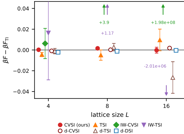
FIG. 7. Free-energy estimator errors \beta F - \beta F_{T1} .
