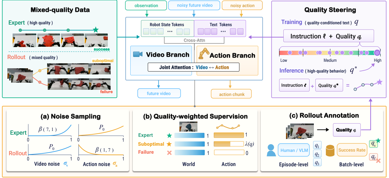
Figure 2: Overview of LoopWAM. LoopWAM is structured as a Mixture-of-Transformer (MoT) architecture, where bidirectional attention enables feature interaction between the video and action branches. Training combines quality-conditioned instructions, source-dependent noise sampling, and quality-weighted action supervision. Expert trajectories supervise both modalities, while lower-quality rollouts retain full world supervision and contribute to action imitation according to their quality. The trained model is deployed using the expert score q^* , and recorded experience returns to the next training round.
