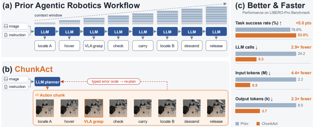
Figure 1: ChunkAct introduces action chunking to agentic robotics, improving both task success and efficiency. Top: prior methods invoke the LLM planner once per primitive, so the number of LLM calls and the context length grow with every step. Bottom: ChunkAct invokes the planner once to launch an action chunk, which executes autonomously and returns a typed error only upon failure. Right: ChunkAct gains both task success and efficiency.
