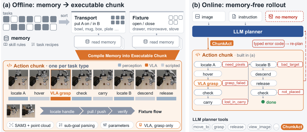
Figure 3: The two stages of ChunkAct. Left: offline, ChunkAct internalizes memory by compiling it into executable action chunks. Right: online, the LLM planner invokes ChunkAct via a single function call, which executes an entire action chunk autonomously and returns a typed error code to the planner only upon failure.
