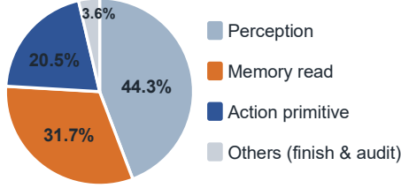
Figure 2: Distribution of LLM planner’s tool calls on LIBERO. Memory reads and perception dominate.
