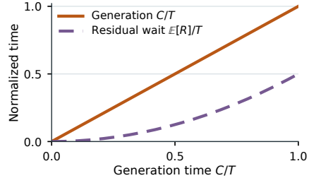
Figure 4: At fixed T , direct generation scales as C/T , while residual wait scales as \mathbb{E}[R]/T = (C/T)^2/2 under the stated periodic model.
