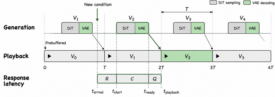
Figure 2: Generation speed alone does not determine response latency. In this periodic reference schedule, the highlighted update waits R for generation, takes C to produce deliverable output, and waits Q for playback. Each chunk is prepared for the next playback period; V_0 is prebuffered.
