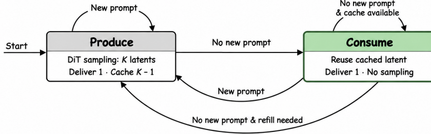
Figure 3: Speculative Sampling serving system and control. (a) Joint generation populates a prediction cache for fine-grained delivery and playback; playback progress guides refill. (b) The finite-state machine coordinates generation in Produce and prediction reuse in Consume, illustrated for q = 1 . Condition updates trigger feasible replanning without interrupting active generation; playback continues in both states.
