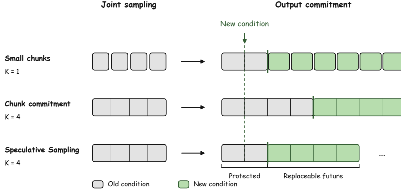
Figure 1: Fine-grained interaction without shrinking generation chunks. Our method preserves large-chunk joint sampling while allowing updates beyond the protected prefix, rather than only at chunk boundaries. Gray/green denote old/new conditions; the dashed line marks playback position at condition arrival, and thick green edges mark updated output. Positions represent video content, not computation time.
