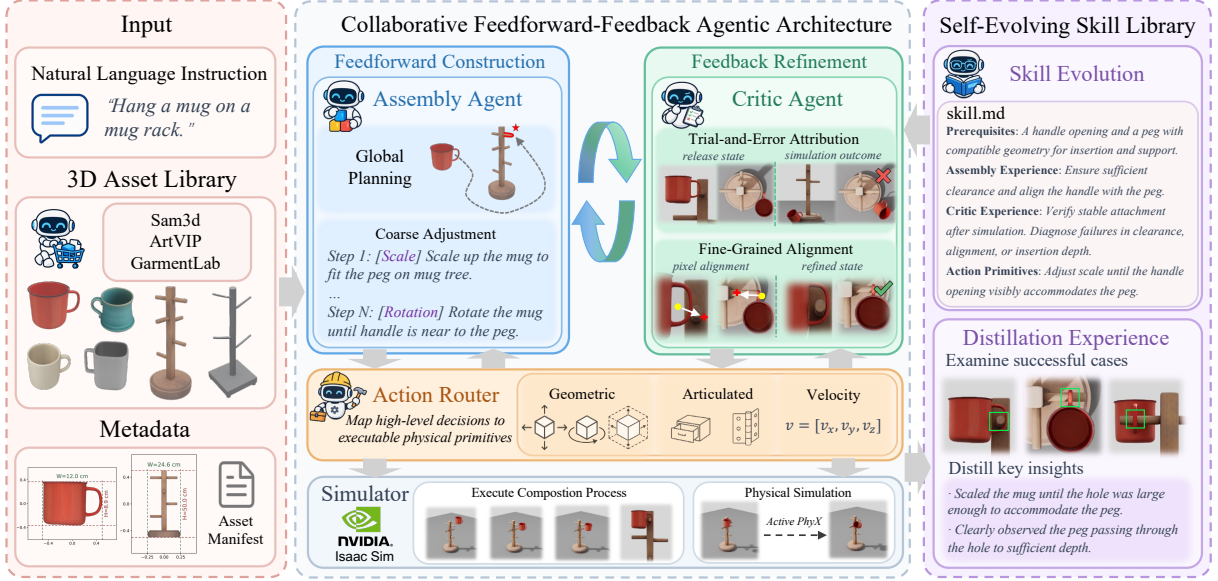
Figure 2. Overview of the PhySGA framework. Driven by a collaborative Feedforward-Feedback architecture, the Assembly Agent executes metric-grounded coarse adjustments, while the Critic Agent performs pixel-grounded fine-grained corrections via simulation feedback. Action Routers translate these semantic decisions into decoupled physical commands, and a Self-Evolving Skill Library distills successful interactions into reusable skills.
