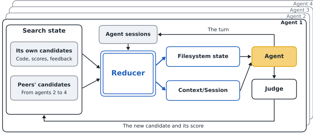
Figure 3: The harness. The reducer reads the agent’s search state and its sessions and decides what the agent sees and which session it continues. The agent then edits a candidate and the judge scores it. The harness records the new candidate with its score in the search state and the turn in the agent sessions. A team runs four such loops at once, each with its own state, and the candidates of an agent’s peers come from the other three loops.
