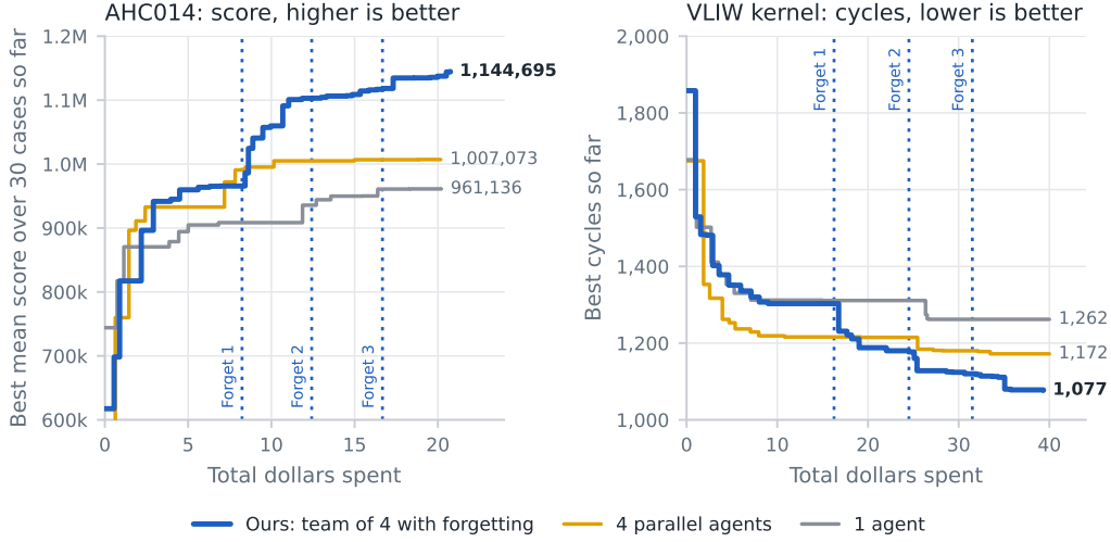
Figure 1: Best score so far against total money spent on AtCoder Heuristic Contest 014 and Anthropic’s VLIW kernel take-home, for the best replicate of each configuration. One autoresearch agent with the same session continued throughout and four parallel agents both plateau early. A team of four agents plateaus as well, until each dotted line, where every state and session is discarded, and the team restarts from the best candidate; each forget unblocks the plateau and the score climbs again. All three use the same configuration and have the same total money spent.
