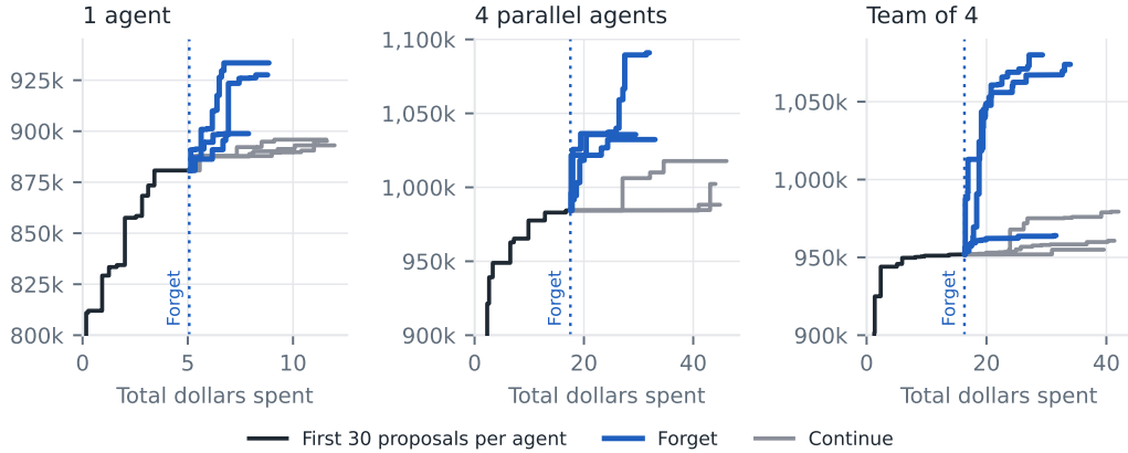
Figure 4: Continue or forget, from the same plateaued state. Best score so far on AHC014 against total money spent. The black line shows the first 30 proposals prefix for all runs. At the forget line, the next 30 proposals per agent either continue the same sessions or forget. Left to right, a single agent, four parallel agents and a team of four. Forgetting climbs higher on average and spends less than continuing the same sessions overall due to shorter context.
