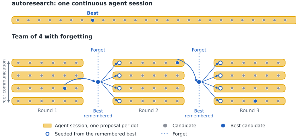
Figure 2: The core idea. Top, autoresearch, where one agent proposes candidates iteratively inside a single continuous session with the whole history in context. Running several such agents in parallel or letting them read one another’s candidates through peer communication still keeps every session, and all of these configurations plateau. Bottom, a team of four agents with communication and forgetting. At each forget line every session and search state are discarded, and only the best candidate so far is remembered, so all four agents of the next round start fresh from that single candidate.
