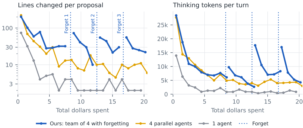
Figure 5: Every session narrows, and forgetting resets it. Inside the AtCoder Heuristic Contest 014 runs of Table 1, three replicates per configuration, pooled. Each point is the median over the proposals that finished within one dollar of a replicate’s spend; the team’s line breaks at each forget, where its sessions are discarded and it restarts from the best candidate.
