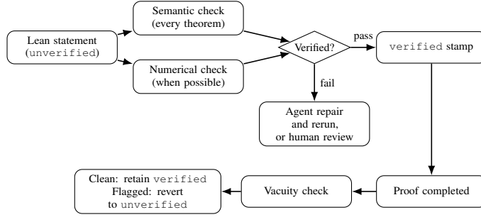
Figure 1: The verification workflow. A theorem is verified if it receives a semantic FAITHFUL and no numerical or vacuity FAIL .
