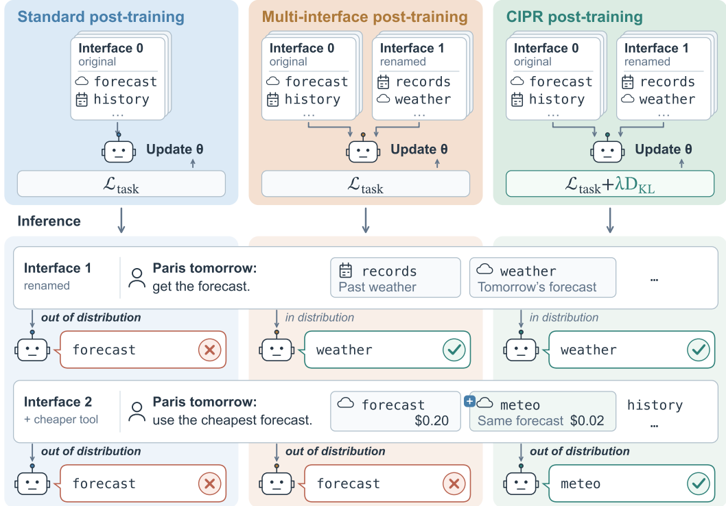
Figure 1: Interface robustness of a tool-using agent (schematic). In each column, we post-train an agent to fetch weather forecasts (top) and then test it at inference (bottom) on a renamed interface ( Interface 1 ) and on one with an added, cheaper forecast tool ( Interface 2 ). The label on each arrow into an agent says whether the test interface is in that agent’s training distribution. Standard post-training on one interface fails both. Multi-interface training handles the renaming, which it saw during training, but misses the new tool. CIPR, which also compares the policy across interfaces, chooses by description in both cases.
