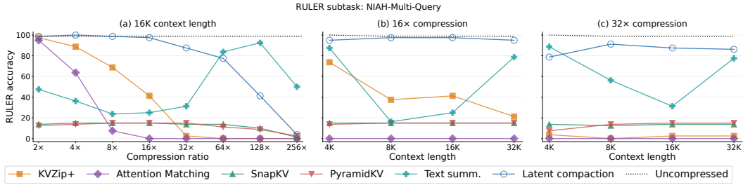
Figure 15: RULER NIAH-Multi-Query: accuracy versus compression ratio at 16K context (left), and versus context length at 16 \times (middle) and 32 \times compression (right).
