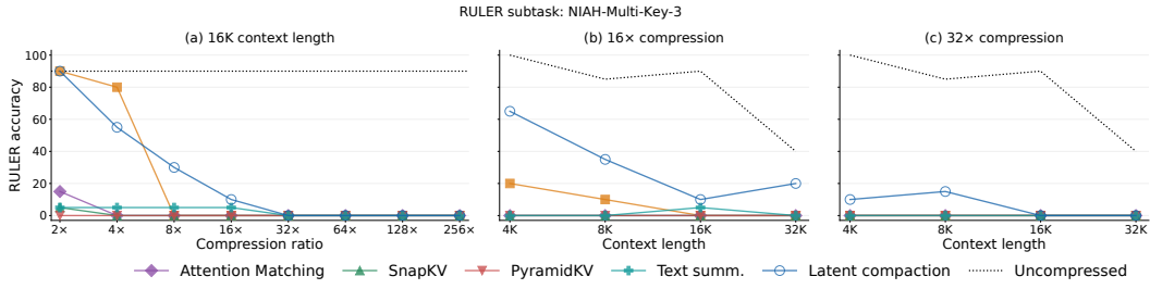
Figure 14: RULER NIAH-Multi-Key-3: accuracy versus compression ratio at 16K context (left), and versus context length at 16 \times (middle) and 32 \times compression (right).
