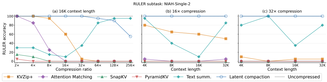
Figure 10: RULER NIAH-Single-2: accuracy versus compression ratio at 16K context (left), and versus context length at 16\times (middle) and 32\times compression (right).
