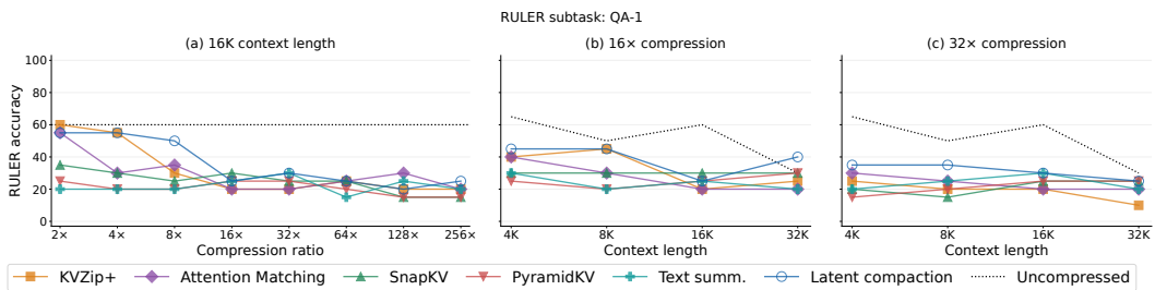
Figure 20: RULER QA-1: accuracy versus compression ratio at 16K context (left), and versus context length at 16 \times (middle) and 32 \times compression (right).
