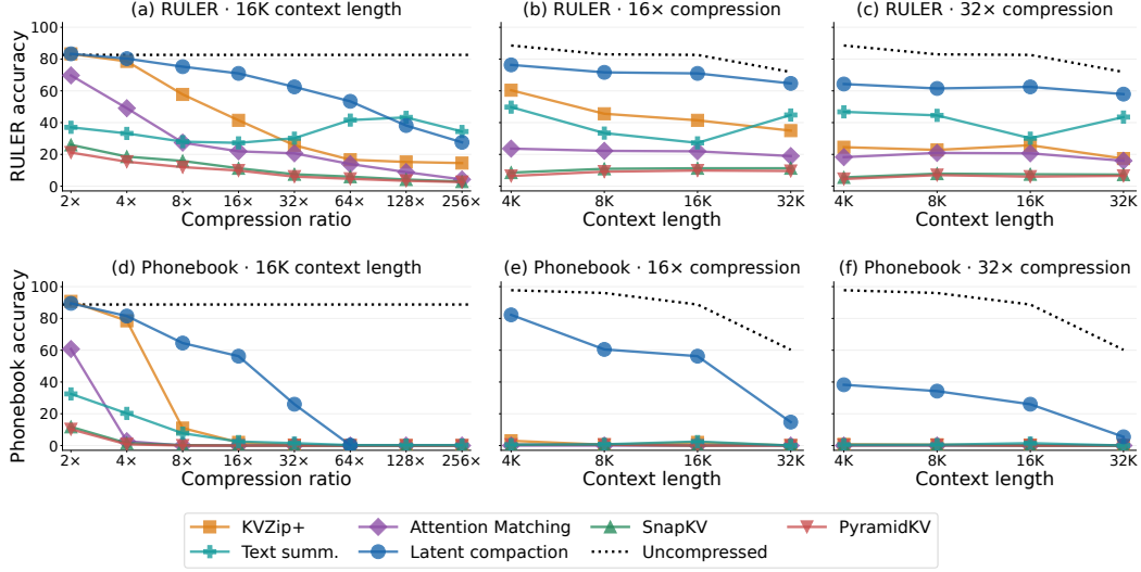
Figure 1: Latent Compaction and baselines across compression ratios and context lengths on RULER and Phonebook Lookup with Qwen3-1.7B.
