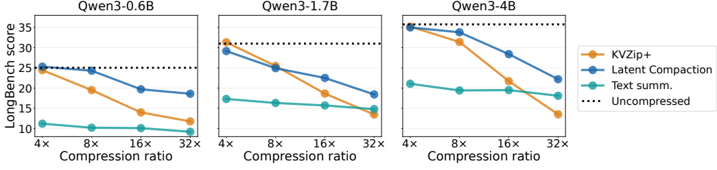
Figure 3: Comparison of compression methods on LongBench.
