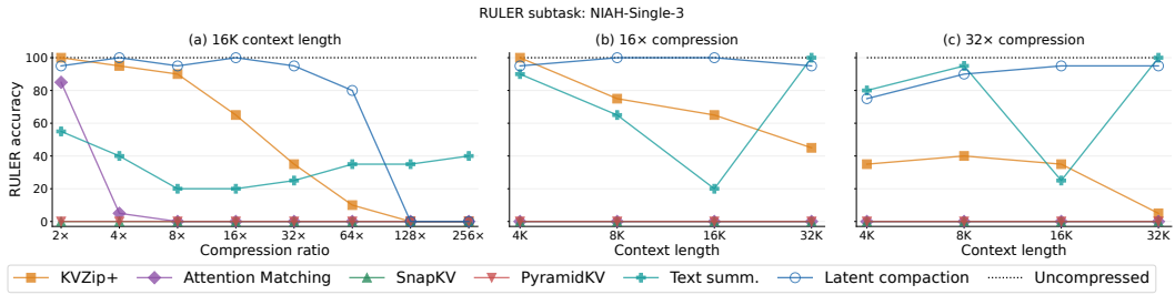
Figure 11: RULER NIAH-Single-3: accuracy versus compression ratio at 16K context (left), and versus context length at 16\times (middle) and 32\times compression (right).
