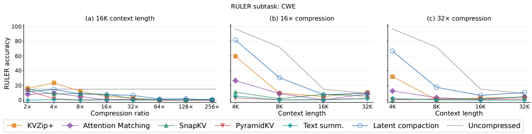
Figure 18: RULER CWE: accuracy versus compression ratio at 16K context (left), and versus context length at 16 \times (middle) and 32 \times compression (right).
