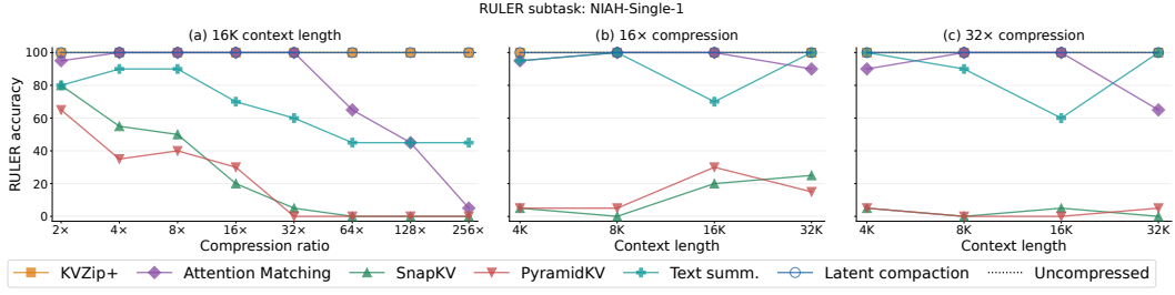
Figure 9: RULER NIAH-Single-1: accuracy versus compression ratio at 16K context (left), and versus context length at 16\times (middle) and 32\times compression (right).
