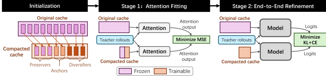
Figure 2: Latent Compaction training pipeline. Preservers, anchors, and diversifiers are initialized from the original cache. Stage 1 freezes preservers and fits anchors and diversifiers to full-cache attention outputs. Stage 2 refines all entries through end-to-end distillation.
