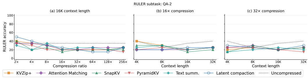
Figure 21: RULER QA-2: accuracy versus compression ratio at 16K context (left), and versus context length at 16 \times (middle) and 32 \times compression (right).
