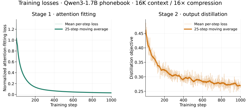
Figure 7: Qwen3-1.7B training losses on 16K Phonebook Lookup at 16× compression. Stage 1 shows the normalized attention-fitting objective (Equation 8); stage 2 shows grouped KL and next-token cross-entropy (Equation 10). Each stage runs for 1,000 updates. Thin lines show per-step means; thick lines show 25-step moving averages.
