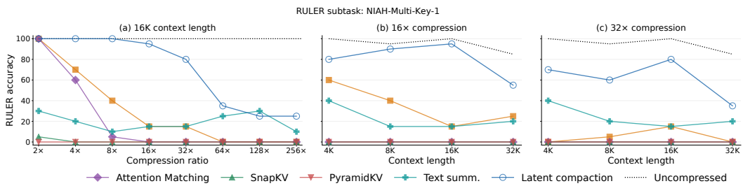
Figure 12: RULER NIAH-Multi-Key-1: accuracy versus compression ratio at 16K context (left), and versus context length at 16\times (middle) and 32\times compression (right).
