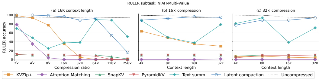
Figure 16: RULER NIAH-Multi-Value: accuracy versus compression ratio at 16K context (left), and versus context length at 16 \times (middle) and 32 \times compression (right).
