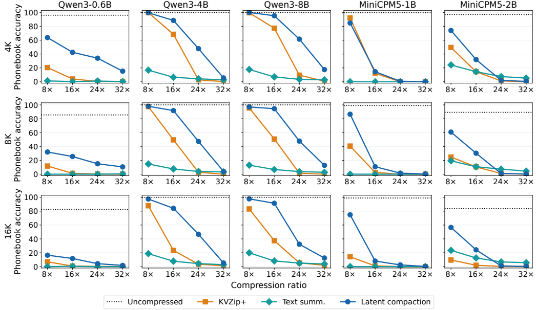
Figure 4: Phonebook Lookup results for additional Qwen3 model sizes and MiniCPM5 models. Each model uses its own document-specific cache optimization.
