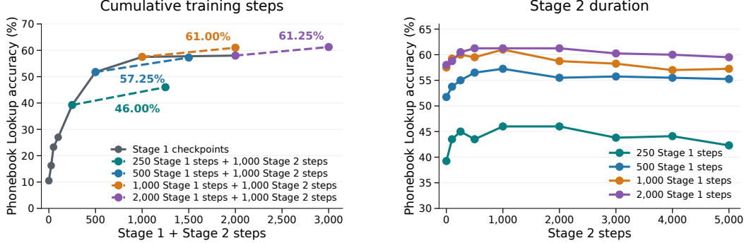
Figure 6: Phonebook Lookup accuracy of Latent Compaction of varying training durations. For clarity, dotted lines only show the accuracy at step 0 and step 1,000 of stage 2.
