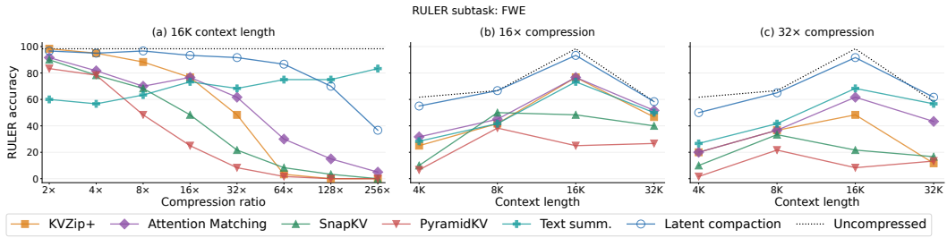
Figure 19: RULER FWE: accuracy versus compression ratio at 16K context (left), and versus context length at 16 \times (middle) and 32 \times compression (right).
