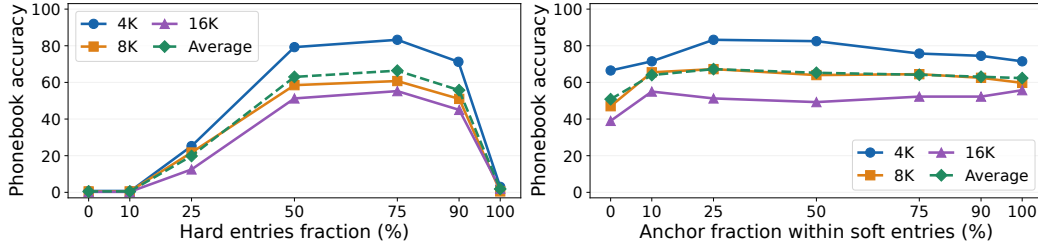
Figure 5: Phonebook Lookup (4K, 8K, and 16K context lengths) accuracy of Latent Compaction at 16\times compression ratio with different fractions of slots allocated to preservers, and different anchor fractions within the combined anchor and diversifier budget.
