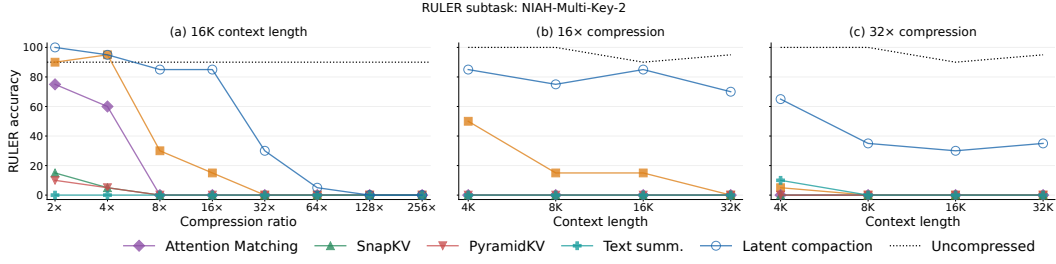
Figure 13: RULER NIAH-Multi-Key-2: accuracy versus compression ratio at 16K context (left), and versus context length at 16 \times (middle) and 32 \times compression (right).
