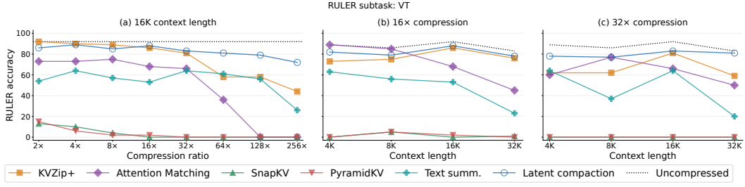
Figure 17: RULER VT: accuracy versus compression ratio at 16K context (left), and versus context length at 16 \times (middle) and 32 \times compression (right).
