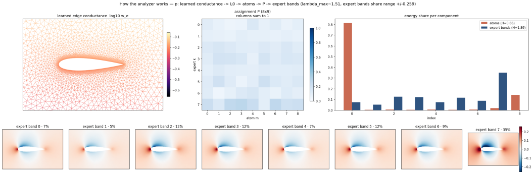
Figure S4: The analyzer and assignment for the illustrated case. Edge conductance w_e ; the 8 \times 9 assignment P (eq. (15)); the eight assigned targets on a shared symmetric colour range; and normalized squared component norms before and after assignment. Global Xavier initialization overwrites the constructor’s preferred assignment logits.
