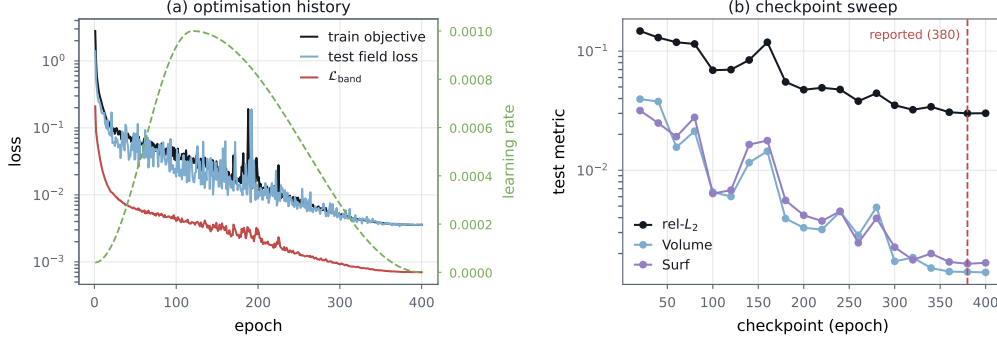
Figure S1: Training the reported model. (a) Training objective, test-set field loss, and auxiliary band loss, with the learning rate on the right axis. The training objective includes auxiliary terms absent from the test-set field loss. (b) The 20-checkpoint test sweep, with the selected checkpoint marked. Selection uses the unrounded mean relative L_2 error.
