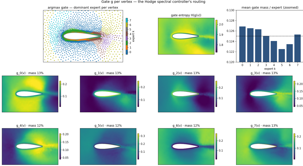
Figure S5: The gate g(v) for the illustrated case. Top: dominant expert at each vertex, per-vertex gate entropy, and mean gate mass per expert against the uniform 1/K line (vertical axis restricted to 0.120–0.130). Bottom: the eight weight fields g_k(v) . These panels describe routing for the displayed mesh rather than averages over the test set.
