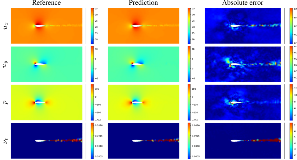
Figure S2: One test case at the reported checkpoint (epoch 380). Columns are the reference, the prediction and the absolute error; rows are u_x , u_y , p and \nu_t . All panels are on the model’s own working mesh in physical units, with the reference and the prediction sharing each field’s colour scale. The per-field relative L_2 for this case is 0.0047, 0.0260, 0.0281 and 0.0676. Test-set means are listed in table S7; the panel illustrates one case rather than a test-set average.
