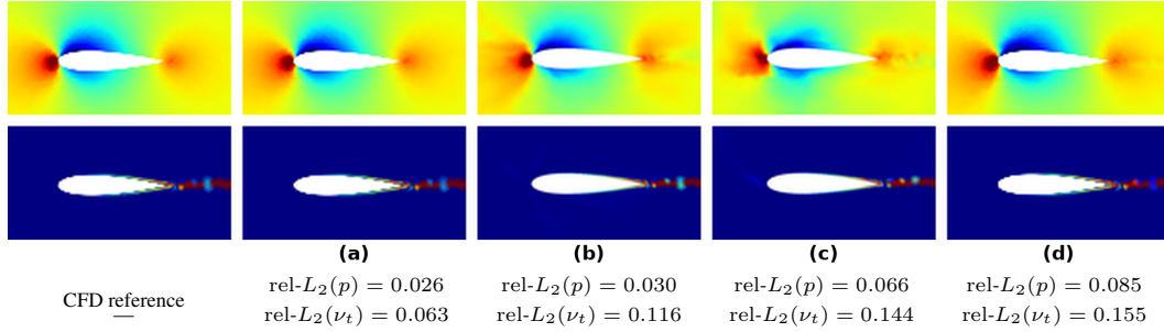
Figure 2: Pressure p (top) and turbulent viscosity \nu_t (bottom) on the reference colour scales; left to right, the CFD reference, (a) our model, (b) Transolver, (c) PointNet, and (d) the best PSD-star HodgeFormer. Values beneath each model panel are mean relative L_2 errors over the 200 test cases. The models differ more on \nu_t than on p ; the reference panel shows fine-scale structure in the \nu_t wake.
