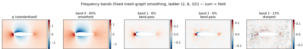
Figure S6: The fixed reference decomposition of the pressure field with the ladder (2, 8, 32) on the unweighted adjacency, for comparison with fig. S3. The normalized squared component norms for this illustrated field are [0.65, 0.06, 0.06, 0.23]; the components overlap.
