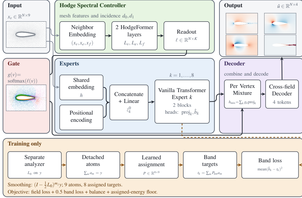
Figure 1: Overview of the model. The Hodge controller routes transformer experts that combine shared vertex embeddings with positional encodings at different frequency scales. Their representations are mixed and decoded into four fields. During training, a separate analyzer decomposes the reference fields into atoms, which a learned assignment combines into targets for the auxiliary expert heads (dashed path).
