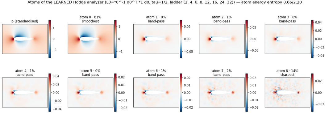
Figure S3: The nine telescoping atoms of the analyzer for the illustrated pressure field. Atom 0 is the coarsest remainder; atoms 1–7 are differences between smoothing levels, and atom 8 is the finest residual. The coarsest and finest components account for approximately 81% and 14% of the summed squared atom norms. Their sum reconstructs the field algebraically, subject to floating-point rounding (eq. (14)).
